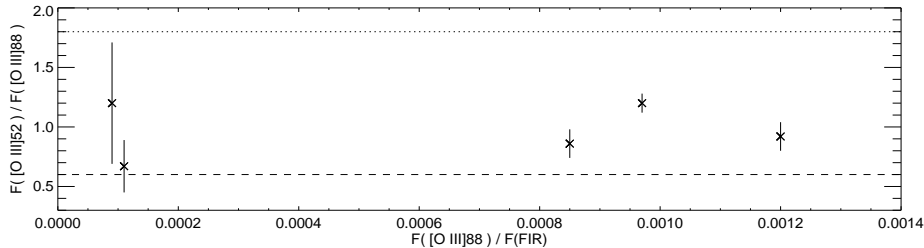
Figure 2. The [O III]52\mu m/[O III]88\mu m line ratio versus the [O III]88\mu m line to integrated far-infrared continuum flux ratio for the sample galaxies. The dashed and dotted lines show the [O III] line ratio in the low density limit ( \leq 100\text{ cm}^{-3} ) and for an electron density of 500\text{ cm}^{-3} , respectively (Fischer et al. 1999).
