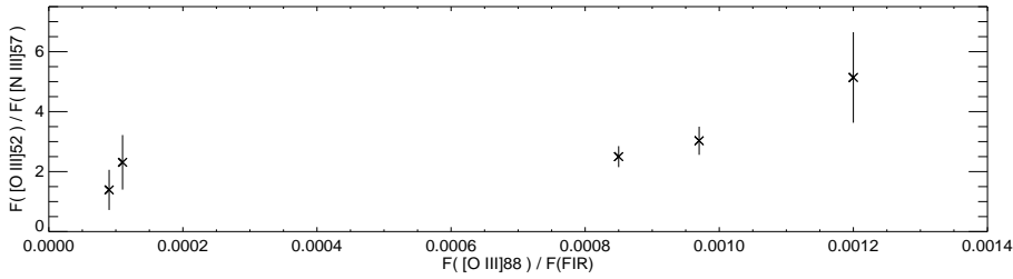
Figure 4. As in Figure 2 for the [\text{O III}]52\mu\text{m}/[\text{N III}]57\mu\text{m} line ratio.
