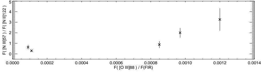
Figure 3. As in Figure 2 for the [\text{N III}]57\mu\text{m}/[\text{N II}]122\mu\text{m} line ratio.
