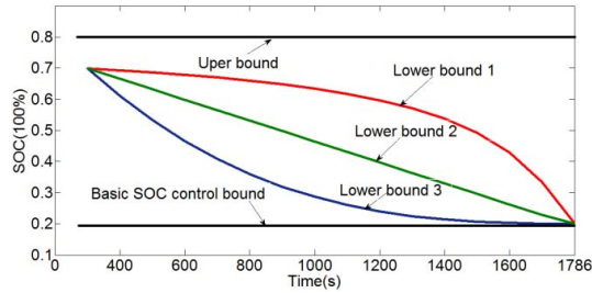
Fig. 8. SOC reference control bound examples.
