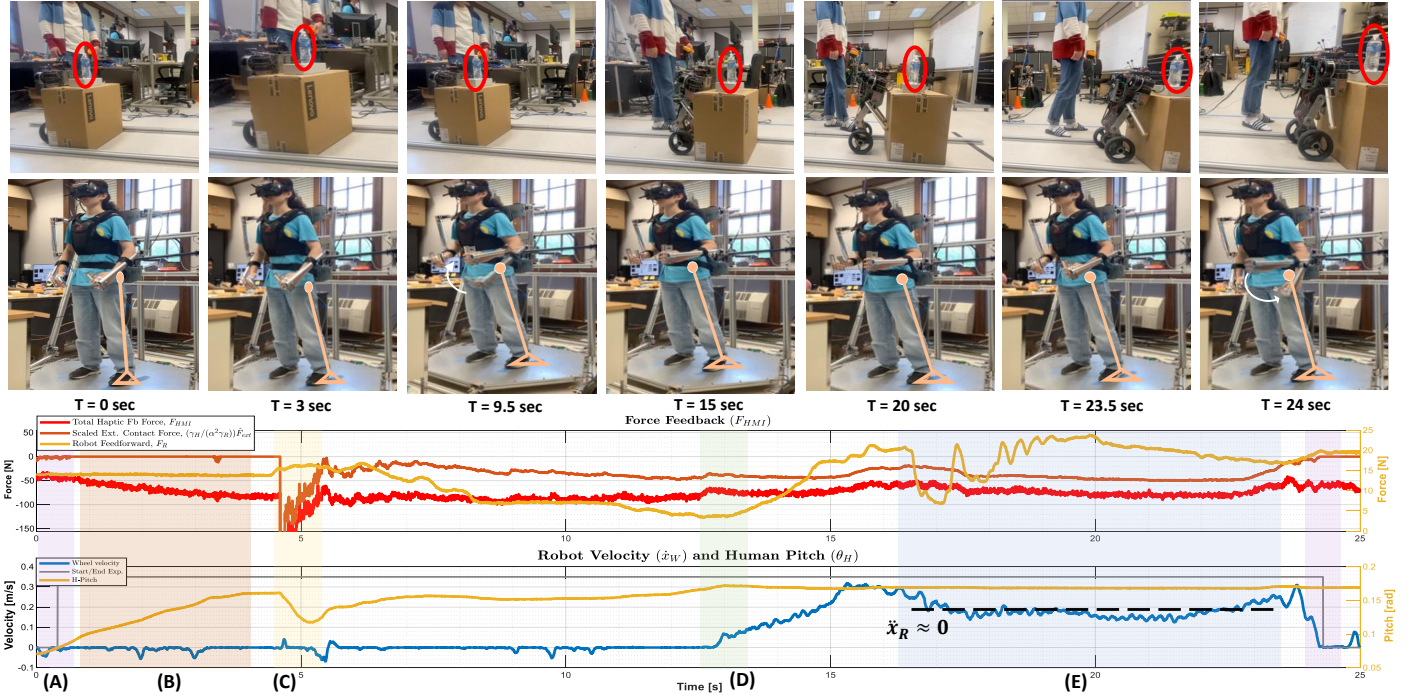
Fig. 8. Heavy box pushing experiment: A 8.5kg (67.5 % of m_R ) box with a balanced bottle is pushed at constant velocity. (A) shows in purple start and end of task. In (B) the pilot initially increases their lean without using their arms. At (C) the robot’s hands make contact with the box and begins pushing with the arms resulting in a sharp change in external contact force. The pilot continues moving their arms up until (D), where the robot breaks stiction and the box begins moving, accompanied by a change in external force. (E) shows the box moving at a constant velocity. At the end, the pilot breaks contact by lowering their hands. The right axis show the zoomed in feedforward force and human pitch in their respective graphs.
