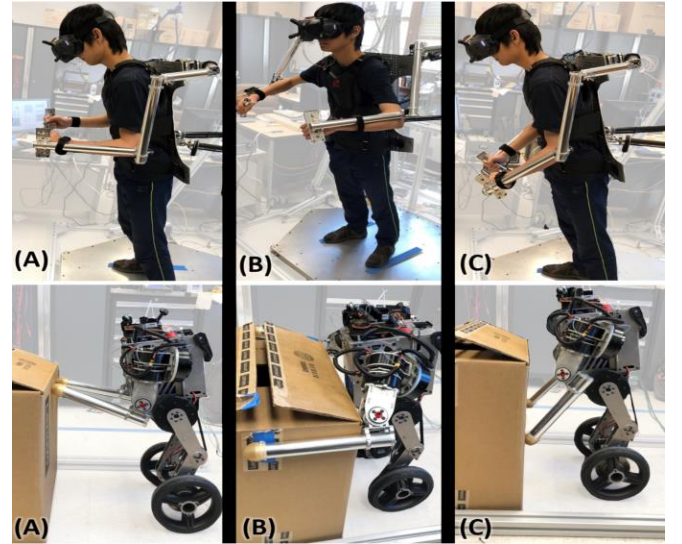
Fig. 7. The pilot tried different poses during box pushing experiments and adapted their strategy to move boxes weighing 8-13kg (63.5-105% of m_R ). In poses (A)-(B) the pilot was unable to push the box, but (C) was successful.
