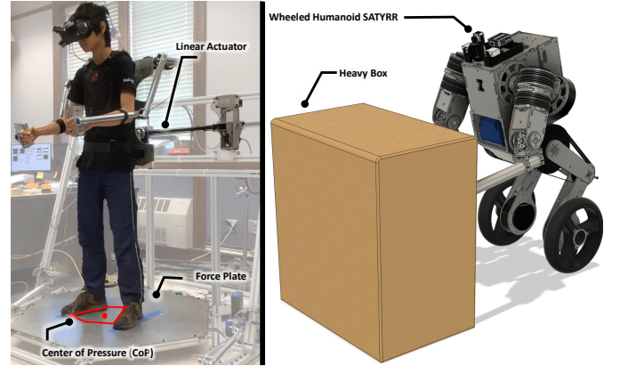
Fig. 1. Dynamic Mobile Manipulation: The pilot in the HMI (left) teleoperates SATYRR (right) to push a heavy box of unknown mass. Linear actuators deliver haptic feedback to human torso informing them of the robot-environment interaction forces. Supplementary video: https://youtu.be/QqcJsSH0YjY
