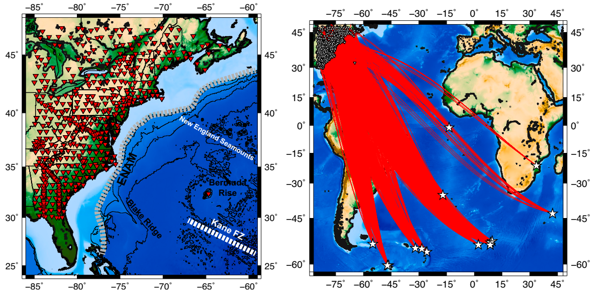
Fig. 1. Maps of the stations (left) and events (right) used in this study. Left: Stations (red triangles) used to examine qL scattering across the ENAM. The Kane Fracture Zone, Bermuda Rise, and New England Seamounts are also shown. The continent-ocean transition is highlighted by the dashed gray line. Right: Earthquakes (stars) used to measure qL scattering throughout our study region. Red lines show great-circle paths of the surface waves that provided measurable qL phases that met our quality control criteria. (For interpretation of the references to colour in this figure legend, the reader is referred to the web version of this article.)
