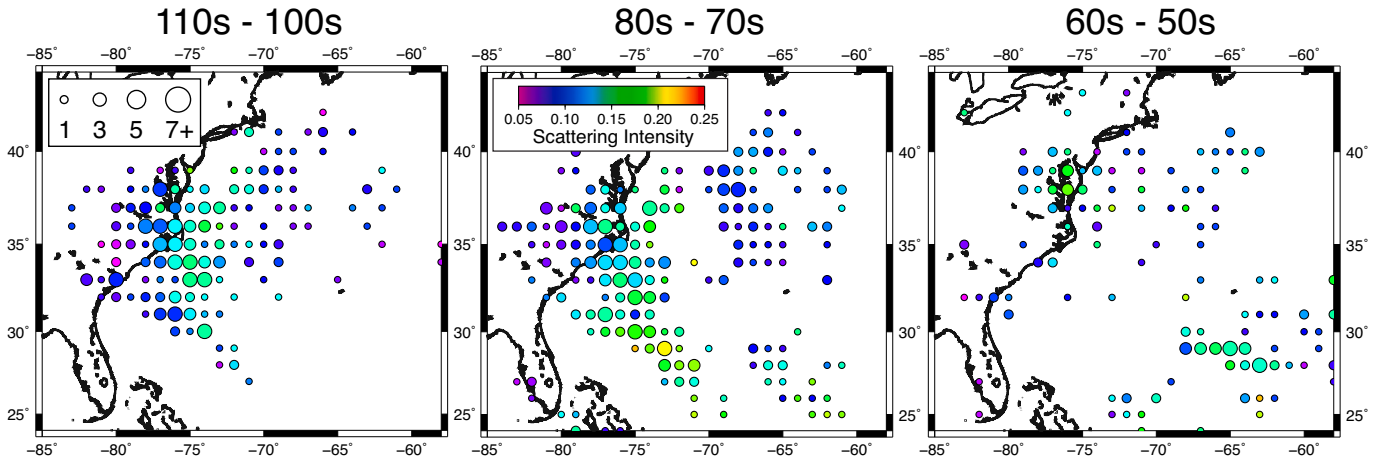
Fig. 5. Averaged qL scattering observations in all three frequency bands. Scattering measurements are averaged in 1^\circ bins. The colour of each circle represents the average scattering intensity for each cell, and each circle is scaled by the number of qL scatterers located in that bin.
