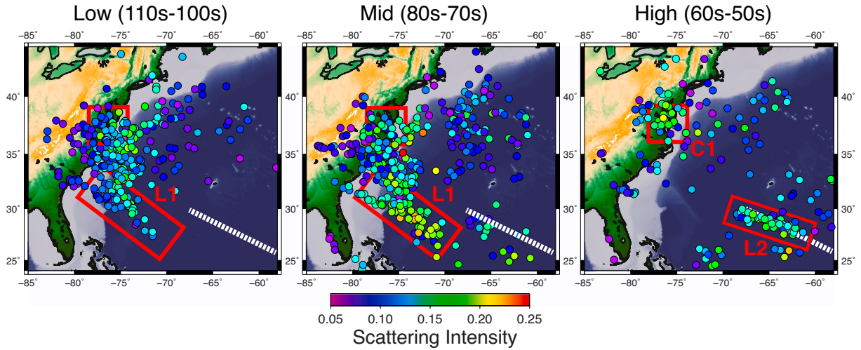
Fig. 4. qL scattering results throughout our study region in all three frequency bands. Anisotropic scatterers (circles) are located by back-projection along ray paths using the measured time delays. Colors give scattering intensity. The Kane Fracture Zone is shown by the white dashed line. Scattering is focused along the ENAM and linear feature L1 in the mid and low frequencies. In the high frequency data, measurements are concentrated around linear feature L2 and the onshore region C1.
