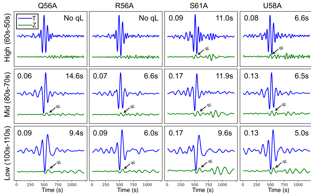
Fig. 3. Examples of qL scattering recorded in all frequency bands at 4 stations from the June 27th, 2014 event in the Scotia Arc. The transverse component is shown in blue and the vertical in green. All examples have strong, clear Love waves. qL scattering (highlighted with arrows) is present in all 4 cases in the low and mid frequencies and is absent in 2 examples from the high. Measured time delays and scattering intensities are shown in the upper right and left corners of the panels, respectively. (For interpretation of the references to colour in this figure legend, the reader is referred to the web version of this article.)
