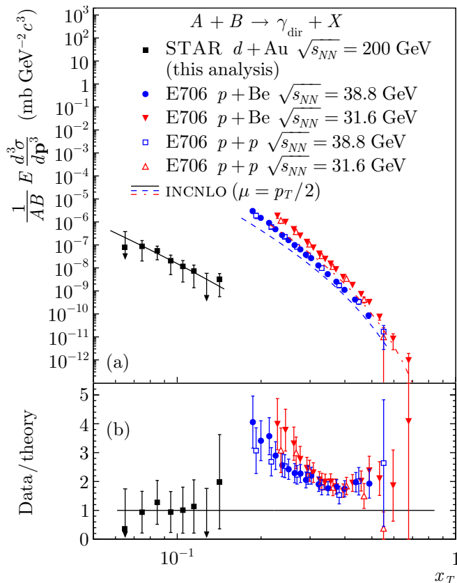
FIG. 29: (color online) (a) The cross sections per nucleon for direct photon production in d + Au collisions, compared to the measurements in p + p and p + A collisions by E706 experiment [70] at the comparable nucleon-nucleon center-of-mass energies. The theoretical curves were calculated with the INCNLO program [72] with \mu = p_T/2 . All data have statistical and systematic uncertainties summed in quadrature. The vertical arrows indicate our estimate of the 95% confidence level. (b) The ratio of the data and the corresponding calculations.
