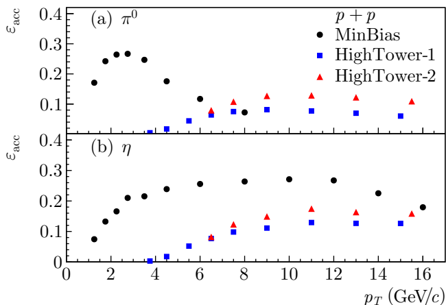
FIG. 13: (color online) Acceptance and efficiency correction factor \varepsilon_{\text{acc}} for (a) \pi^0 and (b) \eta , calculated from the Monte Carlo simulation for the p + p data.
