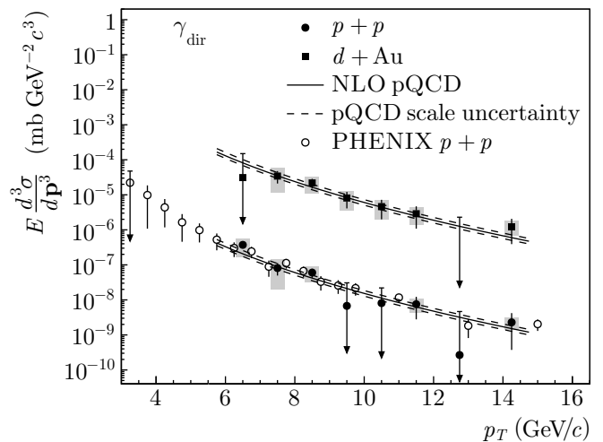
FIG. 28: The differential cross section for direct photon production at midrapidity in p + p and d + Au collisions at \sqrt{s_{NN}} = 200 GeV, compared to the PHENIX measurement [29] and to the NLO pQCD calculation [68], which was scaled with \langle T_{dA} \rangle [Eq. (23)] in case of d + Au collisions. The error bars are statistical the shaded bands are p_T -correlated systematic uncertainties. The arrows correspond to the 95% confidence limits, as defined in the text.
