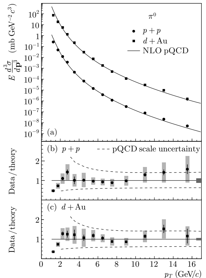
FIG. 22: (a) Cross section for inclusive \pi^0 production in p + p and d + \text{Au} collisions at \sqrt{s_{\text{NN}}} = 200 GeV, divided by the corresponding NLO pQCD calculations [52] for (b) p + p and (c) d + \text{Au} collisions. The error bars are statistical and shaded bands are p_T -correlated systematic uncertainties. Normalization uncertainties are indicated by shaded bands around unity in the lower panels.
