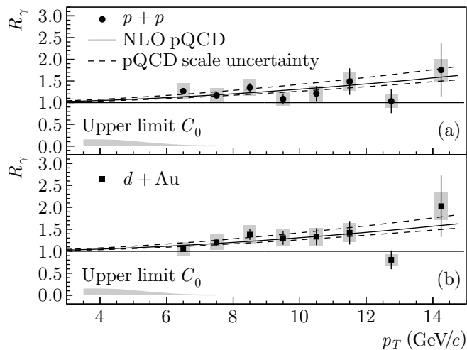
FIG. 27: The direct photon yield in (a) p + p and (b) d + Au collisions at \sqrt{s_{NN}} = 200 GeV, expressed in terms of the double ratio R_\gamma . The error bars are statistical and the shaded bands are p_T -correlated systematic uncertainties. The curves correspond to NLO pQCD calculations of the differential cross sections for direct photon [68] and \pi^0 [52] production in p + p collisions for different factorization scales \mu (the upper pQCD curve corresponds to \mu = p_T/2 ). The upper limit of the fractional neutral hadron contamination C_0 is shown as the shaded band at R_\gamma = 0 .
