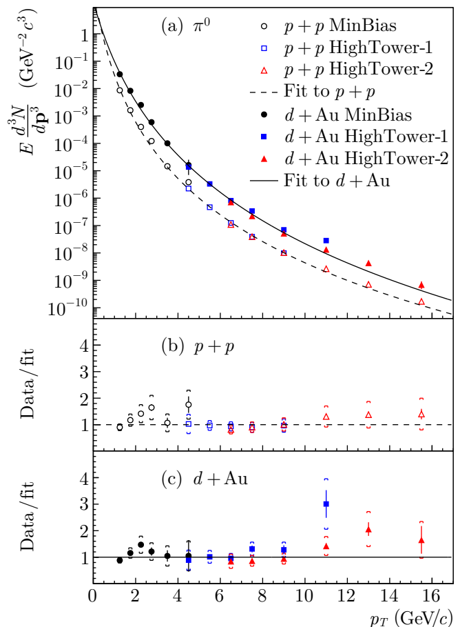
FIG. 15: (color online) (a) Invariant yield of \pi^0 per MinBias p + p and d + \text{Au} collision. Curves are the power law fits given in the text. Invariant yield divided by the fit to the (b) p + p and (c) d + \text{Au} data. The error bars are statistical and brackets in the lower panels are the systematic uncertainties.
