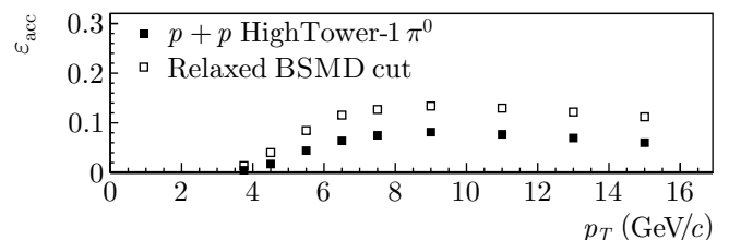
FIG. 14: Acceptance and efficiency correction factor \varepsilon_{\text{acc}} for the p + p HighTower-1 data, with standard set of cuts (solid symbols) and with SMD quality cut removed (open symbols).
