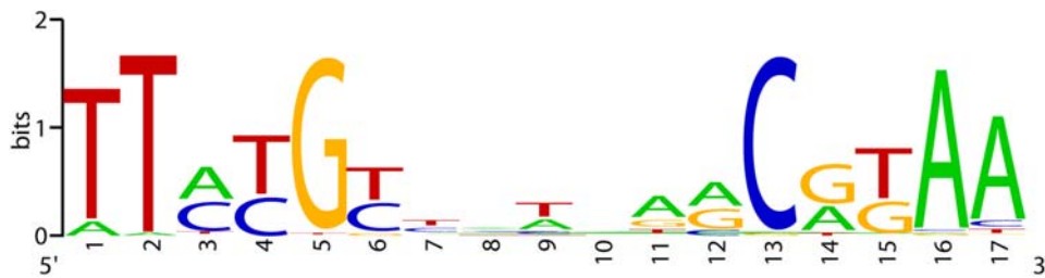
Figure 6. Sequence signature of a predicted site of a radiation response regulator. Four different nucleotides are shown by four letters (A, G, C, T) in different colors. The height of the letter is proportional to its contribution to the information content in the corresponding position of the multiple alignment used for “sequence logo” construction. The figure was constructed by the “sequence logo” program described previously [160]. doi:10.1371/journal.pone.0000955.g006
