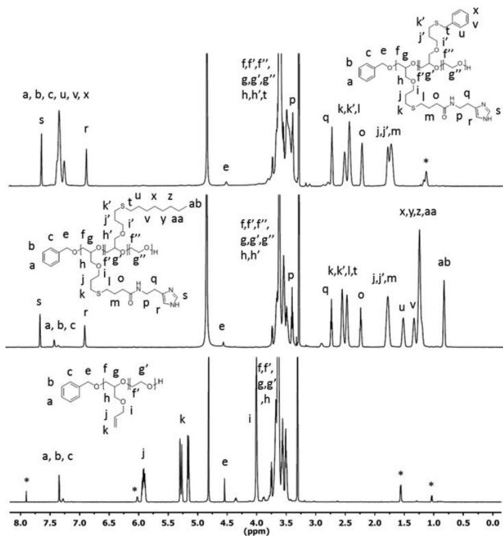
Fig. 1. ^1\text{H-NMR} (MeOD) of PAGE 22 -b-PEO 246 (bottom), P(HGE 11 -OGE 11 )-b-PEO 246 (middle), and P(HGE 10 -BGE 12 )-b-PEO 246 (top). * Corresponds to resonances from the allyl isomer.
