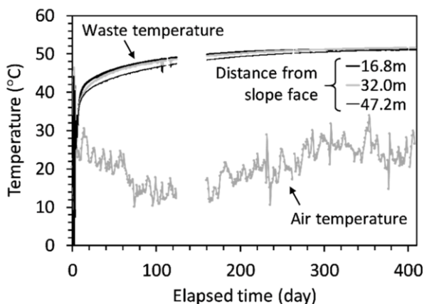
Figure 2. Temperature time series obtained for a 13-month monitoring period following waste placement.
