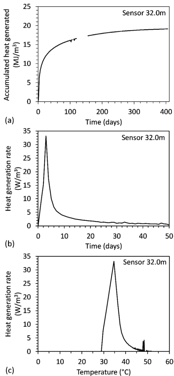
Figure 3. Estimates of heat generation at the location 32.0 m from the slope face: (a) Accumulated heat generated; (b) Heat generation rate as function of time; (c) Heat generation rate as function of temperature.
