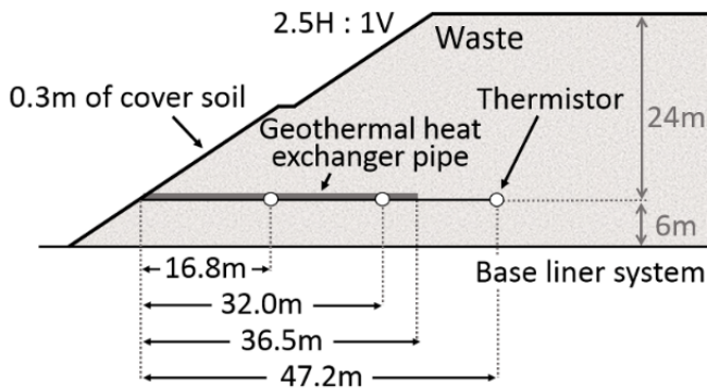
Figure 1. Cross-section showing the position of the thermistor string within the landfill.
