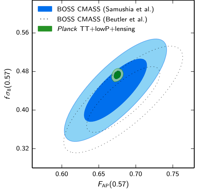
Fig. 17. 68% and 95% contours in the f\sigma_8 – F_{\text{AP}} plane (marginalizing over D_V/r_s ) for the CMASS-DR11 sample as analysed by Samushia et al. (2014, solid, our default), and Beutler et al. (2014, dotted). The green contours show the constraint from Planck TT+lowP+lensing in the base \Lambda CDM model.
