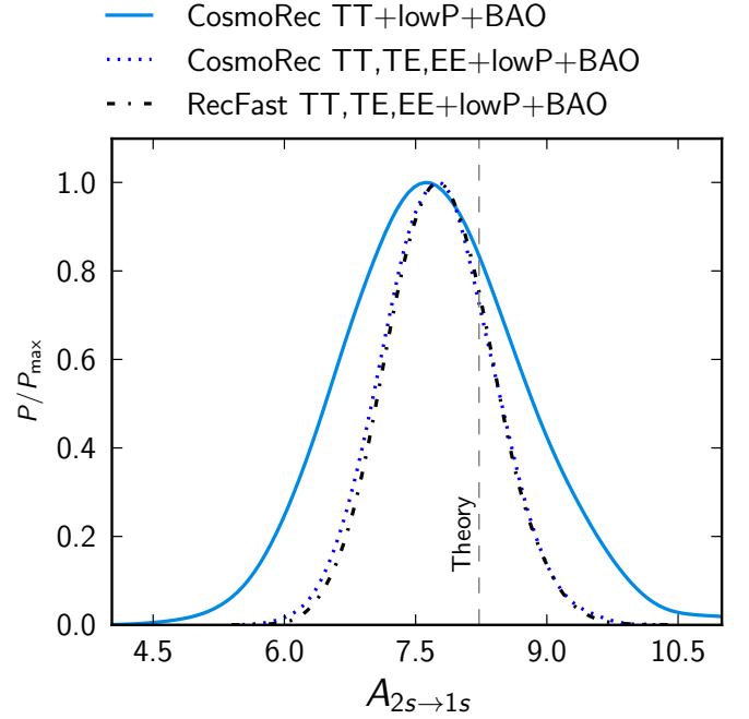
Fig. 42. Marginalized posterior for A_{2s-1s} , obtained using CosmoRec, with and without small-scale polarization data. We find good agreement with the theoretical value of A_{2s-1s} = 8.2206 \text{ s}^{-1} . For comparison, we also show the result for Planck TT,TE,EE+lowP+BAO obtained with recfast, emphasizing the consistency of different treatments.
