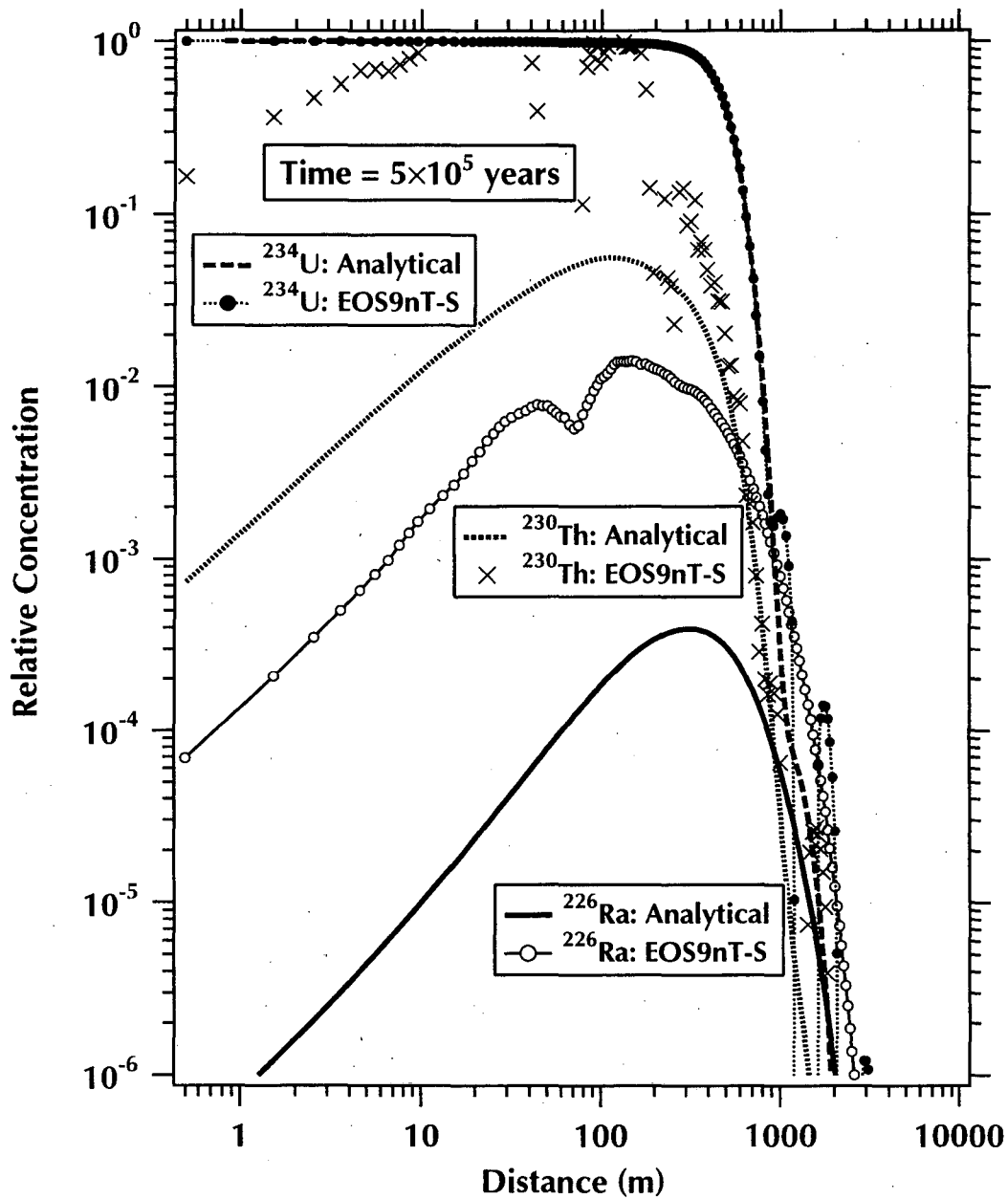
Figure 8. Comparison of analytical predictions of the concentration profiles of the species in the decay chain ^{234}\text{U} \rightarrow ^{230}\text{Th} \rightarrow ^{226}\text{Ra} to the EOS9nT solution with the Stehfest algorithm for Laplace formulation.
