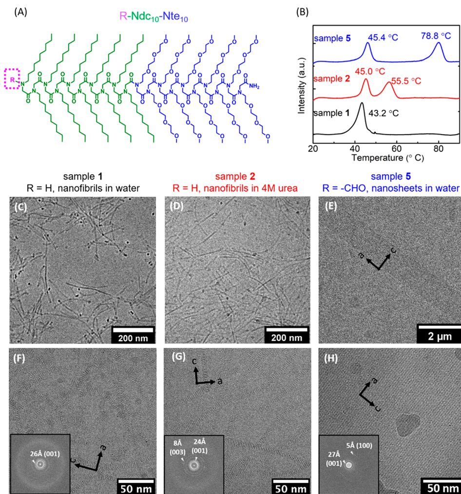
Figure 1. (A) Molecular structure of R-Ndc 10 -Nte 10 . (B) Solution DSC analysis of H-Ndc 10 -Nte 10 in water (sample 1), 4 M urea (sample 2), and F-Ndc 10 -Nte 10 nanosheets in water (where F = formyl) (sample 5). Low-dose cryo-TEM micrographs of peptoid nanostructures embedded in ice at (C–E) low magnification and (F–H) high magnification of samples 1, 2, and 5. In the high-magnification images (F–H), characteristic stripes are observed at d = 26 \pm 1 Å. Crystallographic axes are indicated (black arrows). Dark areas in all images represent the electron dense regions. The fast Fourier transforms are shown in the insets in (F–H).
