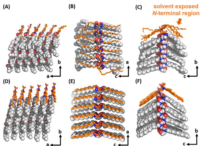
Figure 5. Stacks of lattice from the relaxed MD simulation models of (A–C) H-Ndc 10 -Nte 10 nanofibrils and (D–F) Ac-Ndc 9 -Nte 9 nanosheets. 19 The solvent-exposed Ndc residues neighboring to the N-termini are marked in orange. The computational models evidenced that the solvent-exposed N-terminus destabilized the lattice.
