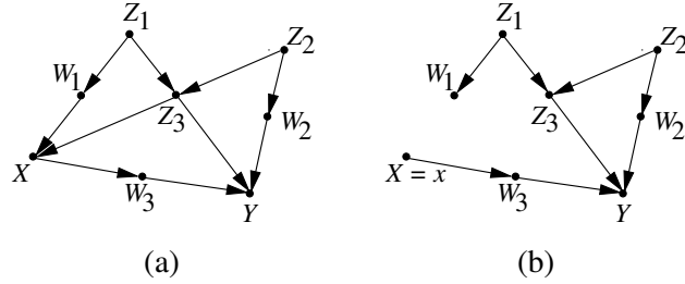
Figure 1: (a) Graphical model illustrating d -separation and the back-door criterion. U terms are not shown explicitly. (b) Illustrating the intervention do(X = x) .
