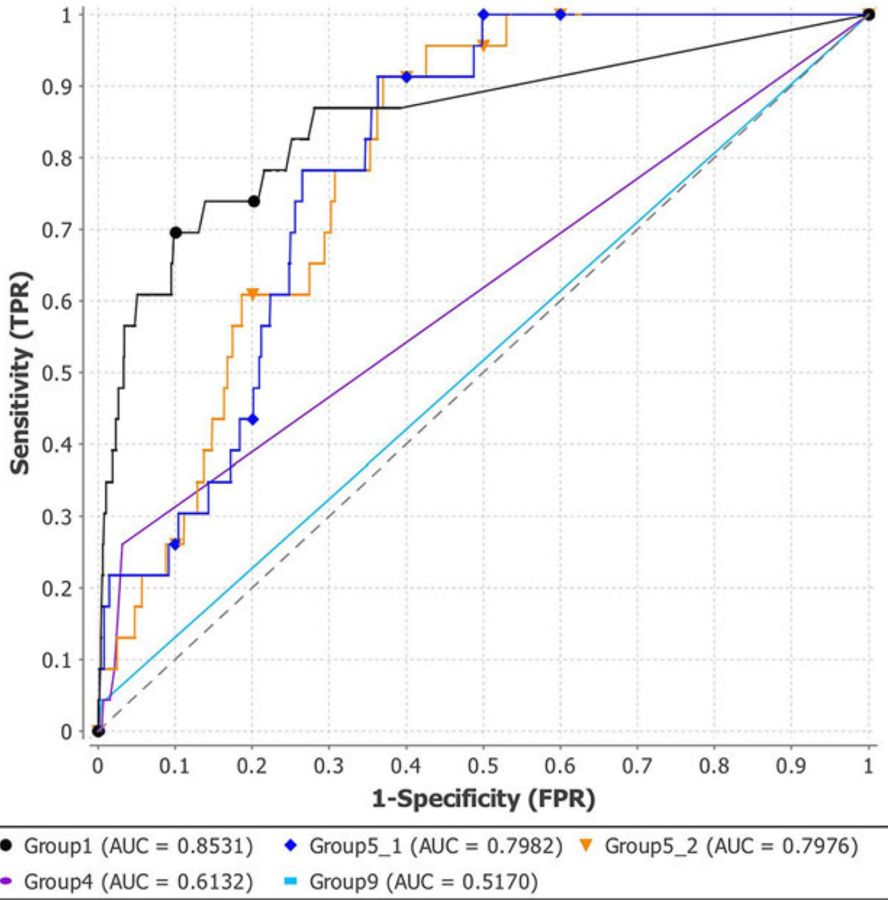
FIGURE 4. ROC AUC curves of the five submissions of PGP 2015
