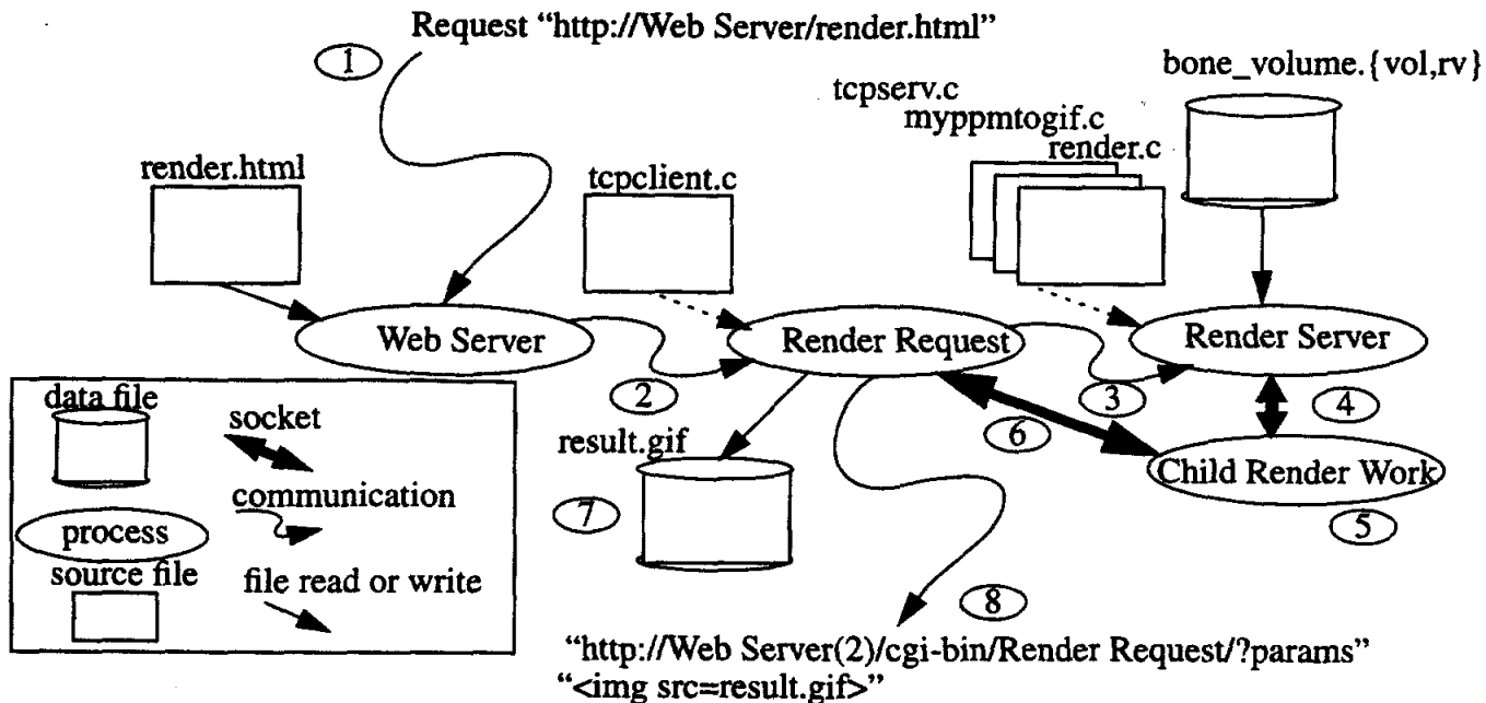
Figure 3: PermWeb architecture
