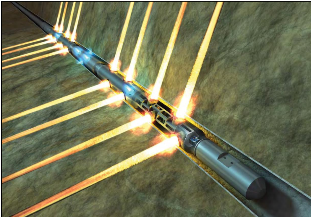
Figure 14: Illustration of a Modern Perforating Gun in Action.
