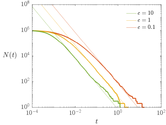
Figure 3: Simulations of the nested Kingman coalescent for various values of c , compared to the asymptotic form N(t) \sim 2\gamma/ct^2 given in Theorem 1. In each case the simulation was started with s = 1000 species each with n = 1000 members.
