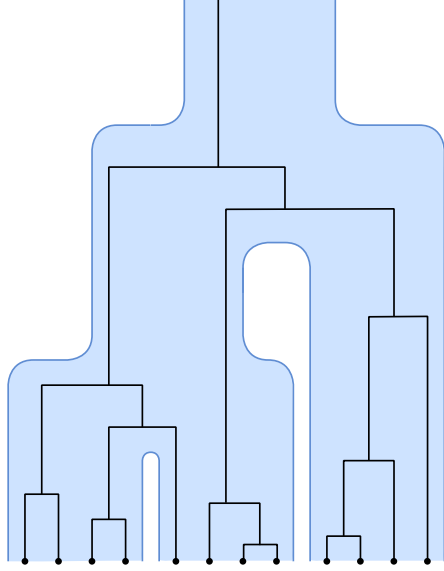
Figure 1: Illustration of the nested Kingman coalescent starting with s = 3 species and n = 4 lineages per species. Black lines show a possible ancestral tree for the sampled individuals, with lineage mergers constrained to lie within the species tree (shown behind in pale blue). The species mergers are described by a Kingman coalescent with rate c , while the within species lineage mergers form a Kingman coalescent with rate 1.
