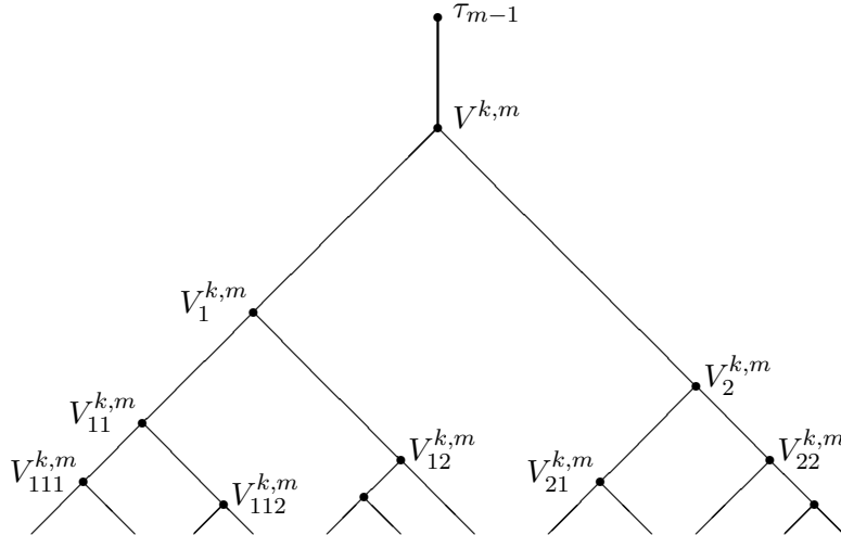
Figure 4: The tree \mathcal{T}^{k,m} .
