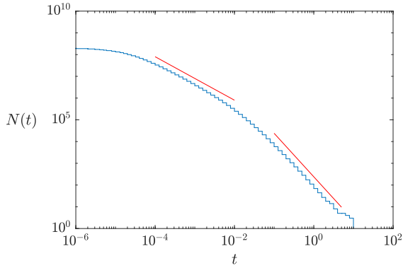
Figure 2: Simulation of the nested Kingman coalescent in the case n \gg s \gg 1 . Here the 1/t^2 phase is preceded by a period of 1/t decay, corresponding to the coalescence occurring within species, but before the species coalescence events kick in. The blue line shows the result of a single simulation with s = 2000, n = 100000, c = 0.1 , the red lines indicate slopes of -1 and -2 to illustrate the different scaling regimes.
