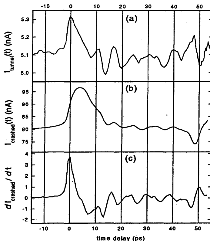
Figure 4. Time resolved current cross-correlation detected on the tip: (a) in tunneling range (5nA and 80mV settings), and (b) when the tip is crashed into the sample. (c) is the time derivative of (b).
