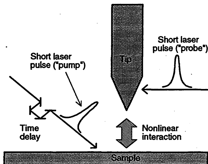
Figure 1. Ultrafast SPM (USPM) : Time resolution is achieved by modulating both the sample and the tip responses with two short optical pulses. A nonlinear tip response acts to correlate pump and probe signals.
