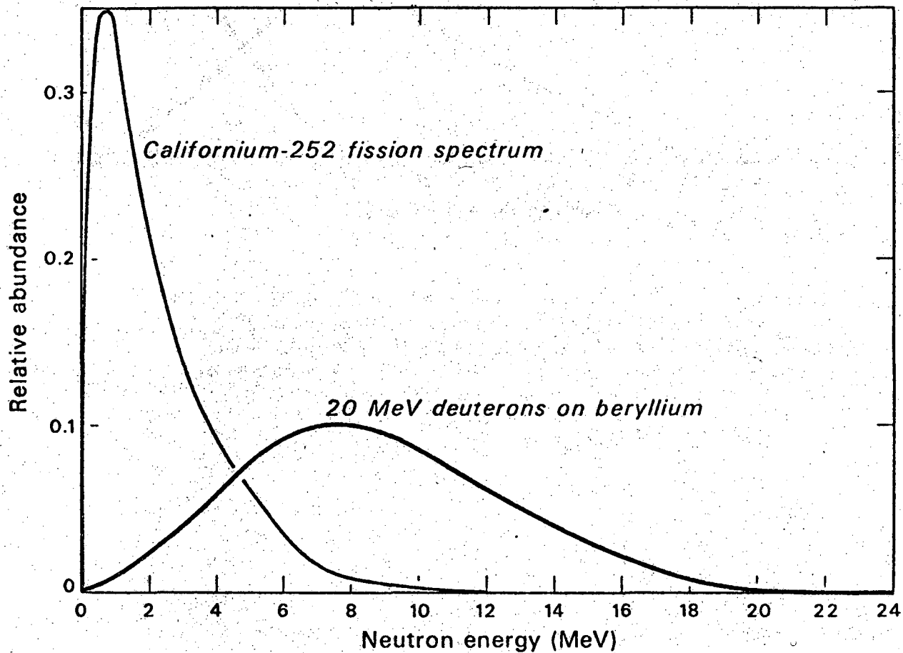
Fig. 1: Neutron spectra normalized so that the integral of N(E) is equal to 1 for californium-252 (3) and the beam from 20-MeV deuterons on beryllium (6). Experiment used 22-MeV deuterons.
