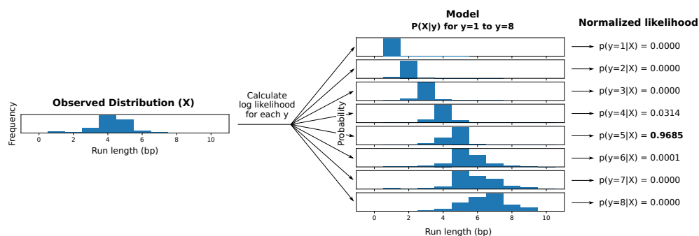
Figure C.10: Visual representation of run length inference. This diagram shows how a consensus run length is inferred for a set of aligned lengths (X) that pertain to a single position. The lengths are factored and then iterated over, and log likelihood is calculated for every possible true length up to a predefined limit. Note that in this example, the most frequent observation (4bp) is not the most likely true length (5bp) given the model.
