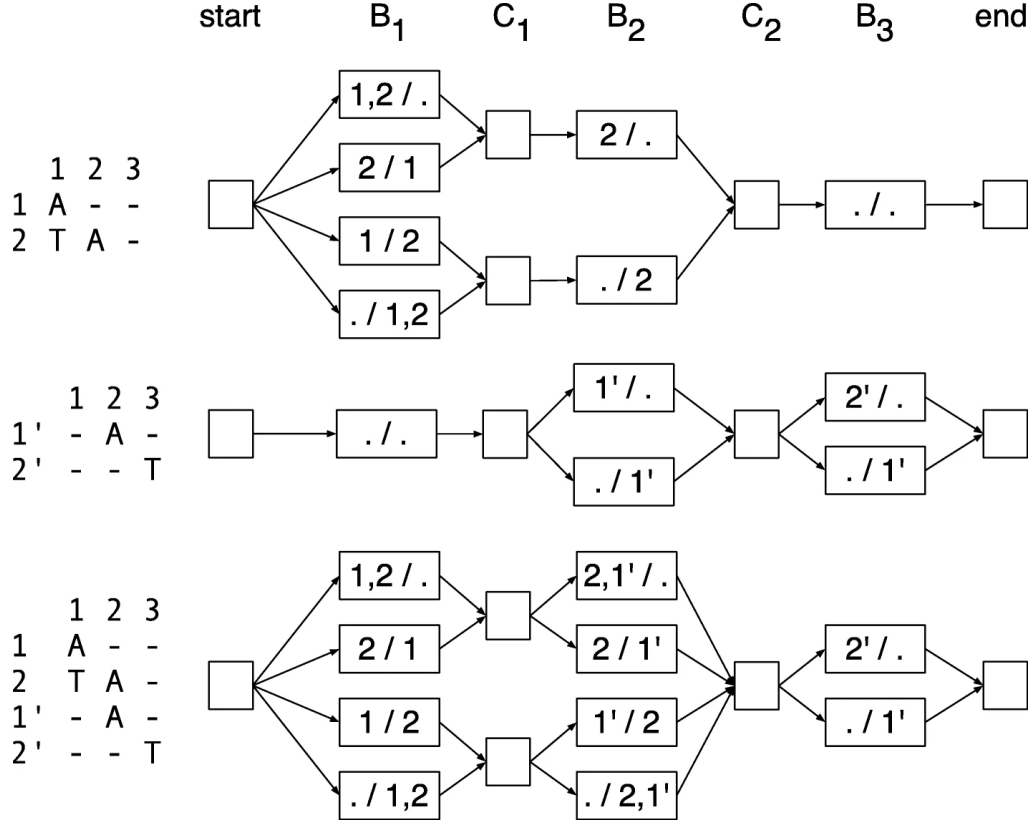
Figure 2.12: The merger of two read partitioning HMMs with the same number of columns. Top and middle: two HMMs to be merged; bottom: the merged HMM. Transition and emission probabilities not shown
