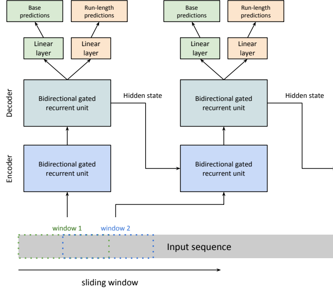
Figure C.12: The sequence-to-sequence model implemented in Helen.
