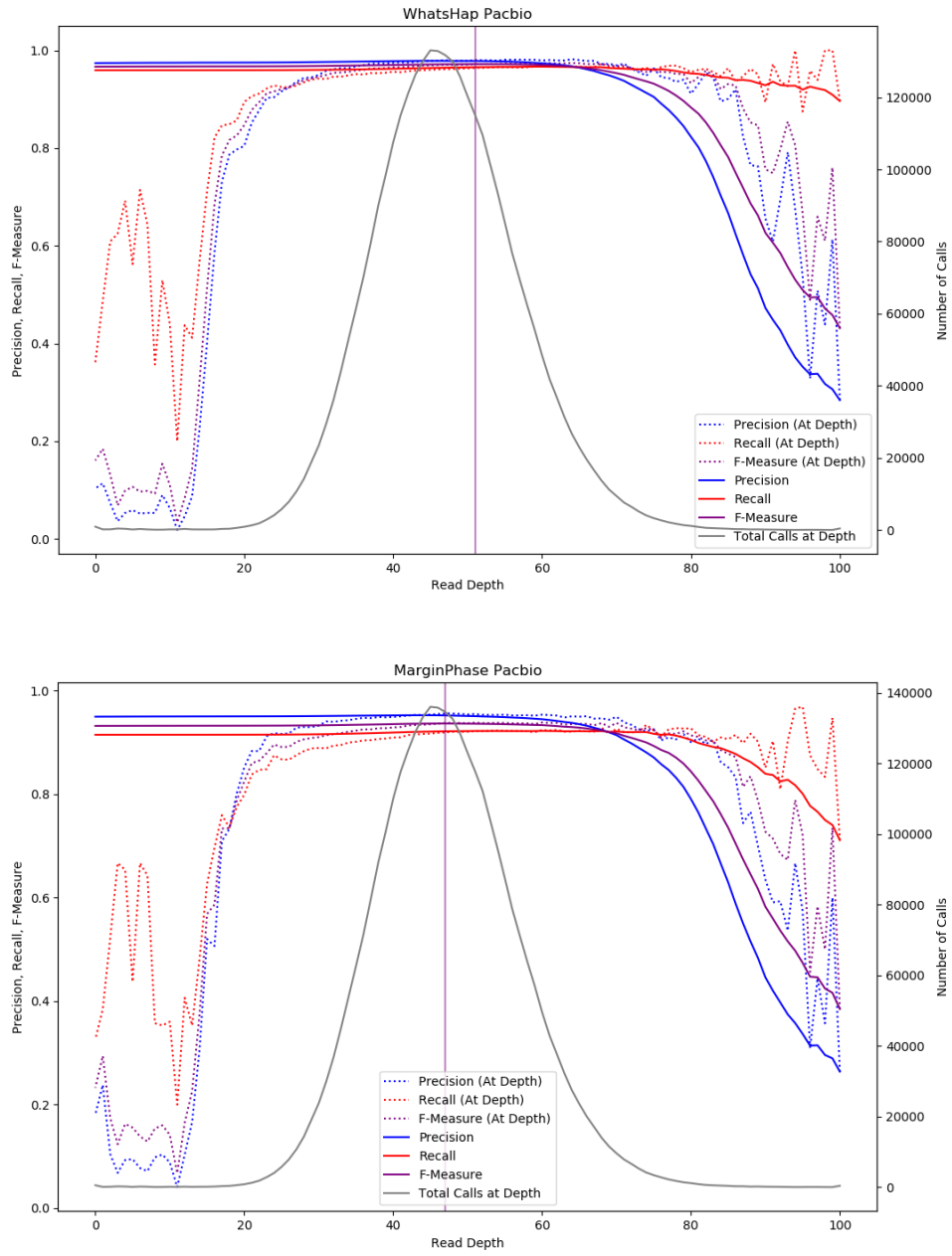
Figure B.3: Read Depth: PacBio Precision, Recall, and F-Measure as a function of depth.
