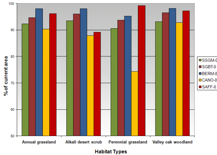
Figure 13. Net loss of natural/semi-natural habitat types under the Minimize Cost scenarios. ssgm = sweet sorghum, sgbt = sugar beets, berm = bermudagrass, cano = canola, saff = safflower.
