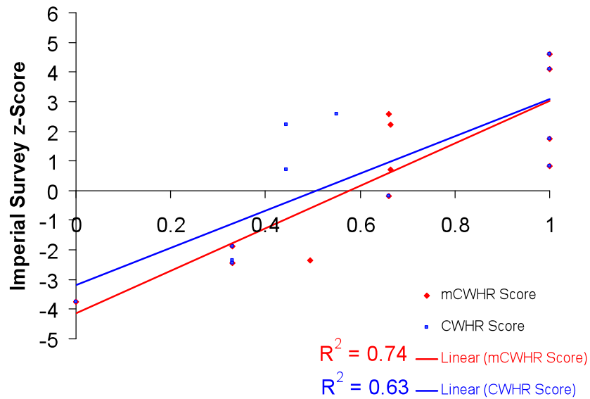
Figure C-2. Relationship between habitat suitability scores from CWHR and mCWHR modeling and z-scores for the Imperial Survey.
