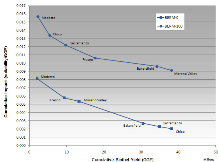
Figure 20. Cumulative trade-off curve for bermudagrass of impact versus biofuel production. berm = bermudagrass; Minimize Cost = -0, Minimize Loss = -100.
