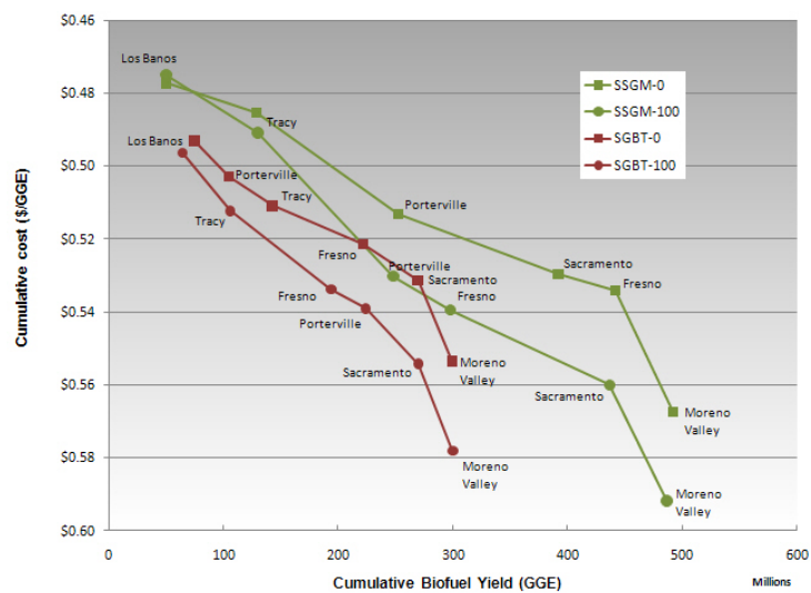
Figure 21. Cumulative trade-off curve for sugar crops of cost versus biofuel production. ssgm = sweet sorghum, sgbt = sugar beets; Minimize Cost = -0, Minimize Loss = -100.
