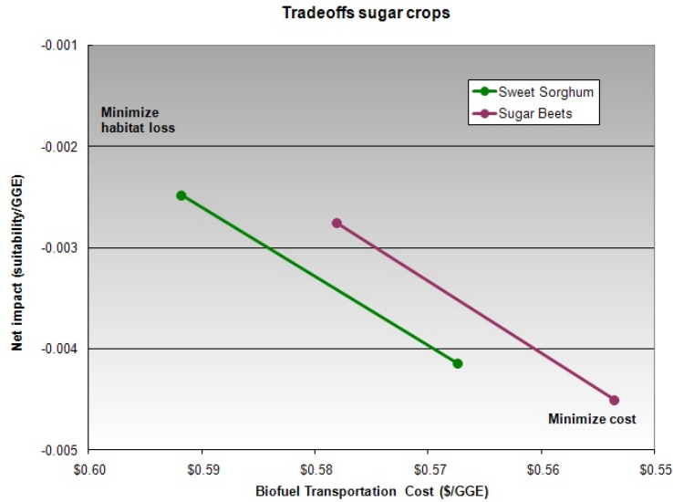
Figure 14. Trade-offs between cost and net impact on habitat suitability per GGE for sugar crops, sweet sorghum and sugar beets.
