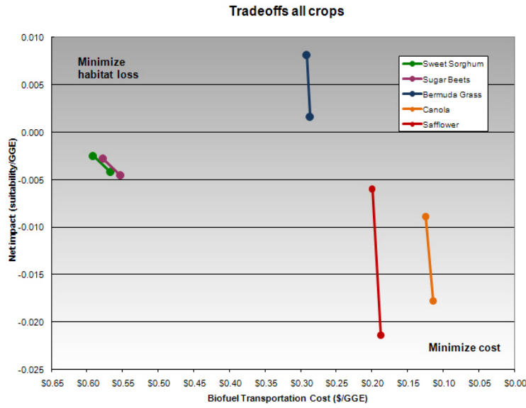
Figure 17. Trade-offs between cost and net impact on habitat suitability per GGE for all five biofuel crops.
