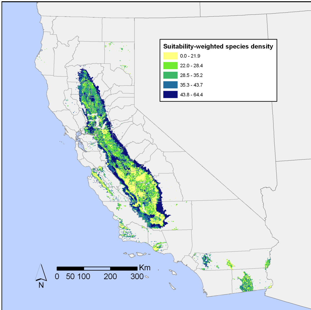
Figure 8. Map of suitability-weighted species density for agroecosystem species by section based on geographic range maps, mapped land use/land cover, and CWHR habitat suitability ratings.
