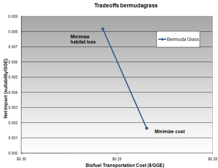
Figure 15. Trade-offs between cost and net impact on habitat suitability per GGE for bermudagrass.
