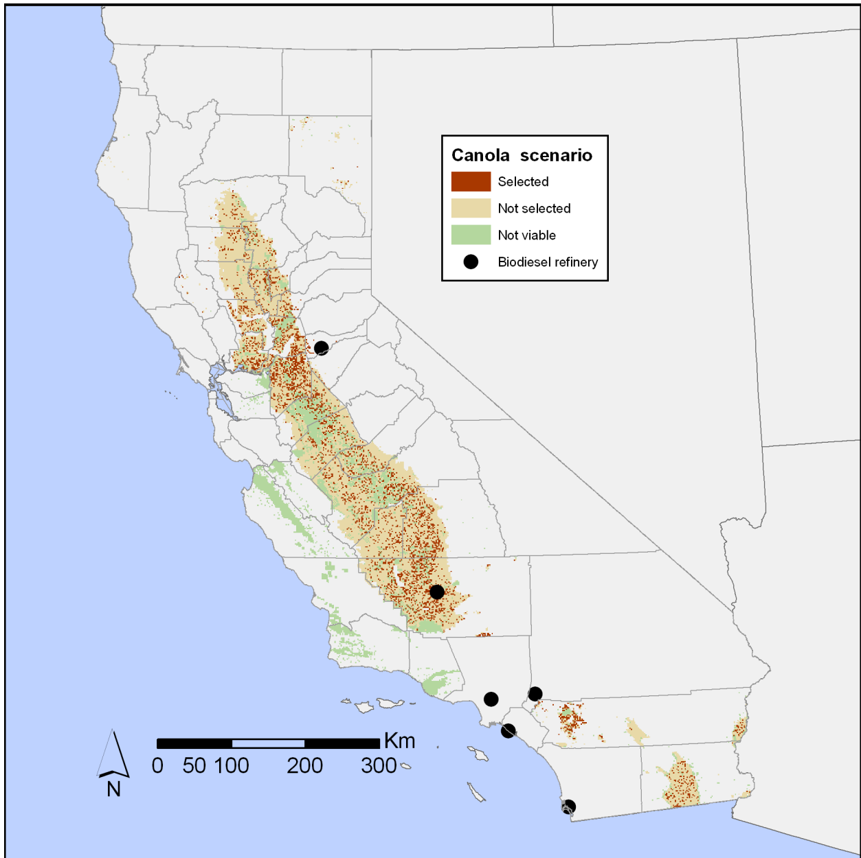
Figure D-8. Minimize Cost scenario for canola (cano1-0).
