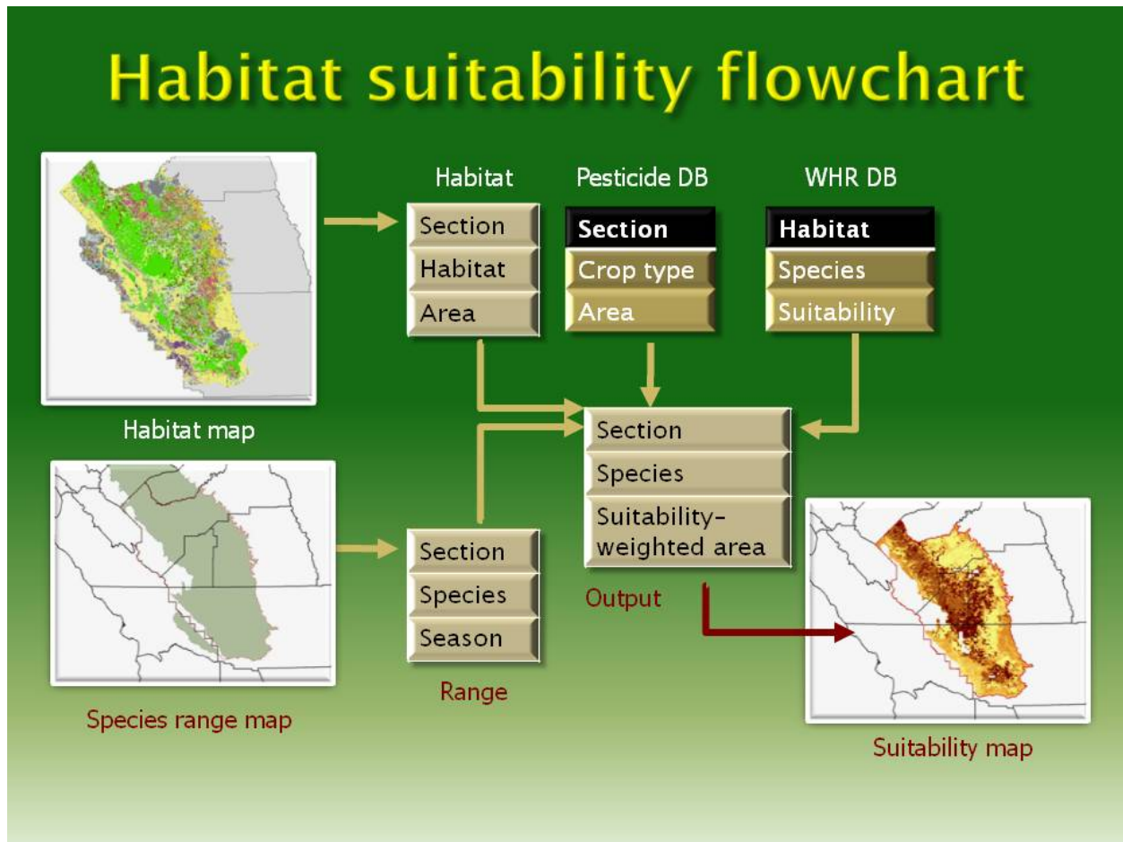
Figure 4. Flowchart of habitat suitability modeling based on PLSS sections.
