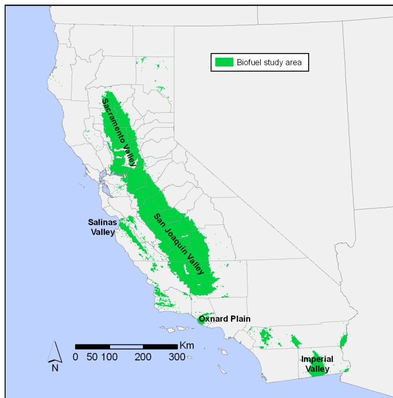
Figure ES-1. California agroecosystems considered for biofuel crop conversion in this study.
