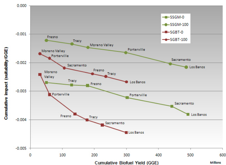
Figure 19. Cumulative trade-off curve for sugar crops of impact versus biofuel production. ssgm = sweet sorghum, sgbt = sugar beets; Minimize Cost = -0, Minimize Loss = -100.
