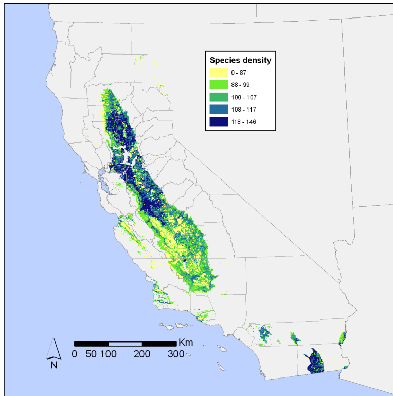
Figure ES-3. Potential number of terrestrial vertebrate species per square mile section (species density) based on geographic range maps, mapped land use/land cover, and CWHR habitat suitability ratings.
