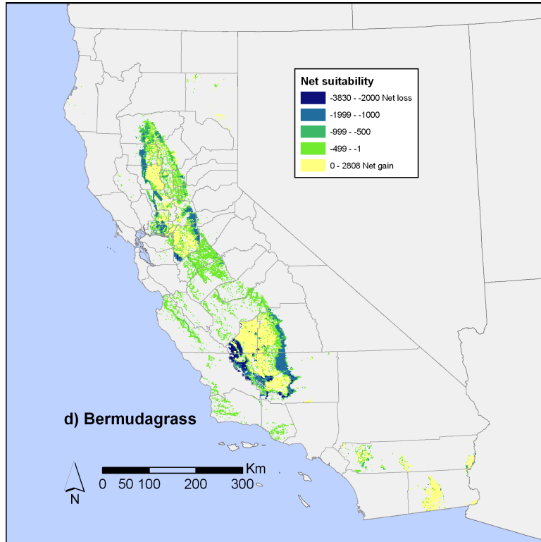
Figure 9 (cont). Suitability-weighted species density for all 53 Species of Special Concern. Net change in suitability-weighted species density if section were converted to c) sugar beets, and d) bermudagrass.
