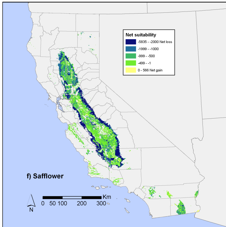
Figure 9 (cont). Suitability-weighted species density for all 53 Species of Special Concern. Net change in suitability-weighted species density if section were converted to e) canola and f) safflower.
