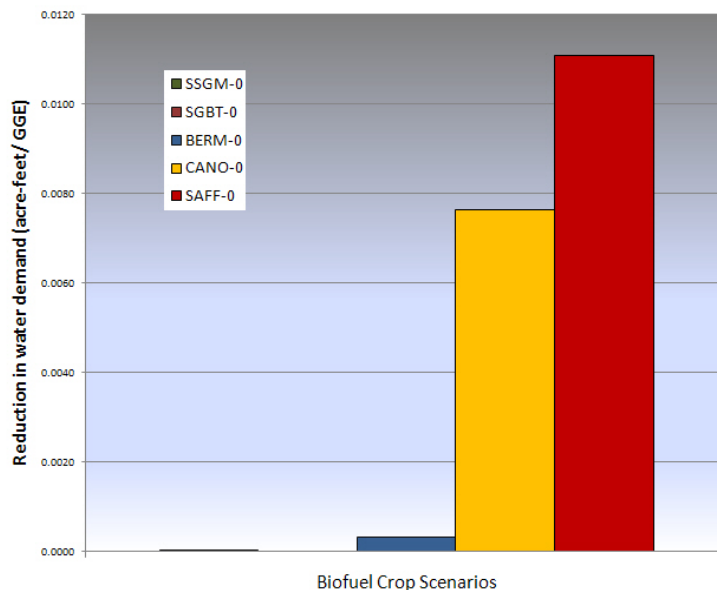
Figure 11. Reduction in water demand to produce one GGE by crop type in the Minimize Cost scenarios. ssgm = sweet sorghum, sgbt = sugar beets, berm = bermudagrass, cano = canola, saff = safflower.
