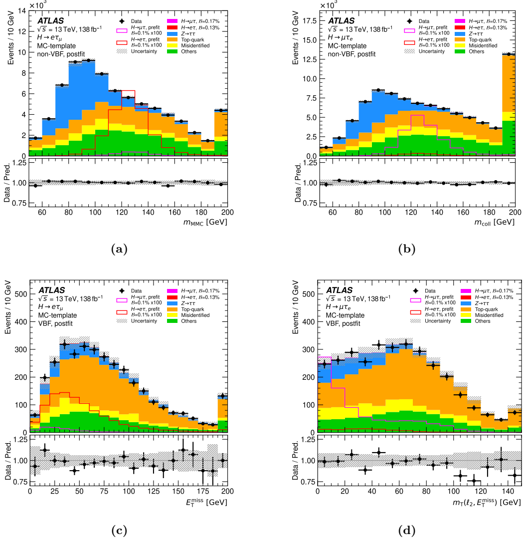
Figure 4. Distributions of representative kinematic quantities for e\tau_\mu (left) and \mu\tau_e (right) final states, after a simultaneous fit of the H \rightarrow e\tau and H \rightarrow \mu\tau signals, obtained by fitting the data of the MC-template \ell\tau_\nu channel: (a) the mass m_{\text{MMC}} and (b) m_{\text{coll}} [87] in the non-VBF category, (c) the missing transverse momentum E_{\text{T}}^{\text{miss}} and (d) the transverse mass m_{\text{T}}(\ell_2, E_{\text{T}}^{\text{miss}}) in the VBF category. Entries with values that would exceed the horizontal axis range are included in the last bin of each distribution. The hashed band represents the prefit statistical uncertainty, and the experimental and theoretical uncertainties obtained from the likelihood fit. Overlaid prefit signal shapes assume \mathcal{B}(H \rightarrow \ell\tau) = 0.1\% and are enhanced by a factor 100 for visibility. The postfit signal contributions are considered as part of the predictions.
