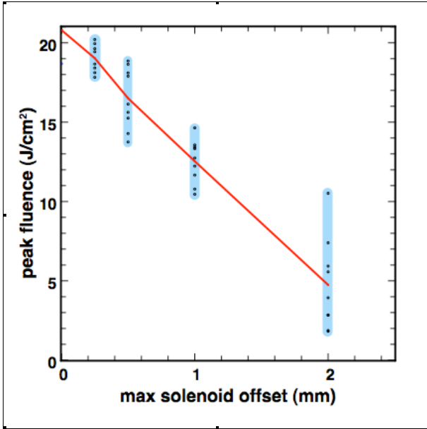
Figure 3. 3-D results from Warp showing the sensitivity of peak fluence when both ends of the focusing solenoids are given a transverse displacement with a magnitude up to a preset maximum offset. The dots mark the results of eight trials with different random numbers made for values of maximum offset, and the range of results for each value is indicated by a blue bar.
