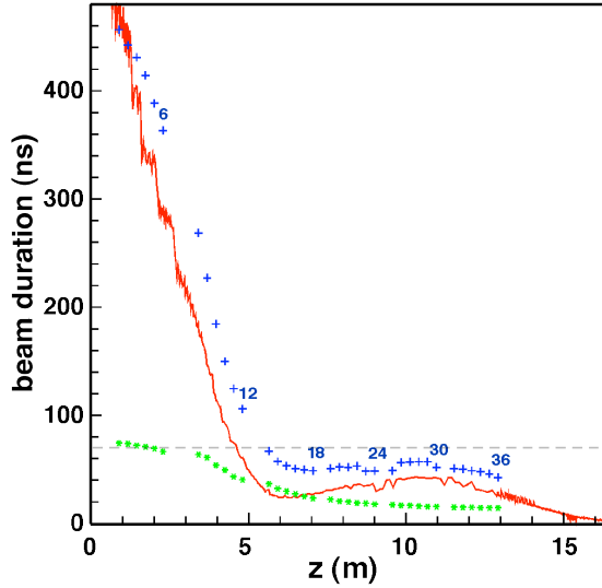
Figure 1. ASP plot of the NDCX-II beam duration. Just enough voltage variation is applied in blocks three through five to keep the beam duration below the 70-ns limit of the Blumleins, shown as a dashed horizontal line. Blue crosses note the transit time of the full beam through each gap, and the green stars indicate the single-particle transit time at the average beam energy. The red shows the beam duration as a continuous function of the longitudinal co-ordinate z .
