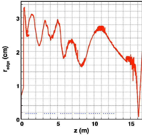
Figure 2. Edge radius from an axisymmetric source-to-target WARP simulation of a 45-nC L^+ beam. The acceleration waveforms were obtained from a 1-D simulation of the same beam and lattice. The small blue “x”s mark the axial centers of the thirty induction gaps in this simulation.
