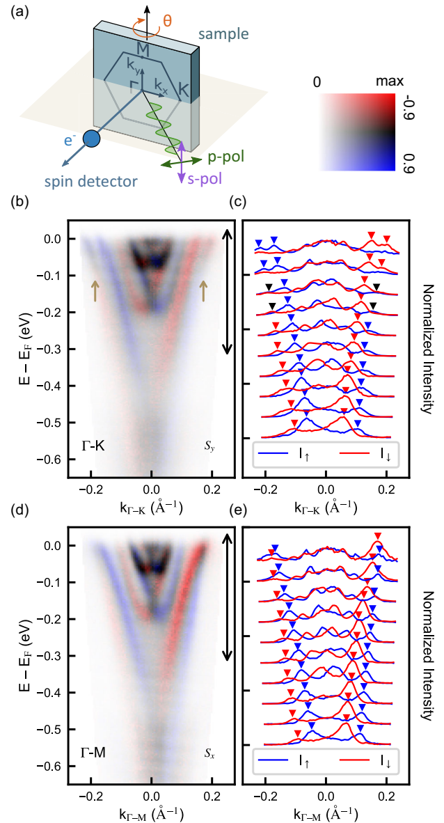
Fig. 2 Spin-resolved ARPES data on BiTeCl. a A schematic of the experimental geometry. Momentum-dependence is mapped by rotating the sample angle \theta . Data in this figure is obtained with s-polarized light. Images are plotted with a 2D colorscale shown in the upper-right: red-blue (vertical) denotes spin-polarization and white-black (horizontal) denotes photoemission intensity. b An in-plane ( S_y ) measurement along \Gamma -K. An unexpected reversal of the spin-polarization is seen in the outermost bands near E_F (beige arrows). c The corresponding momentum distribution curves (MDCs) of spin-up I_{\uparrow} and spin-down I_{\downarrow} intensities. Each MDC is integrated within an energy window of 34 meV. Altogether, the MDCs span the energy range from -329 to 41 meV as denoted by the double-arrows in (b). Each I_{\uparrow/\downarrow} pair is normalized by the maximum intensity for that pair to facilitate a comparison between MDCs at different energies. The markers are guides to the eye denoting peak positions, with blue-black-red coloring indicating the overall polarization of each peak. d , e An analogous dataset along \Gamma -M, in which the outermost bands merge into a single unpolarized peak near E_F .
