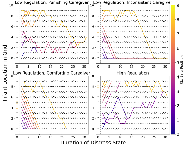
Figure 3: Visualizations of sample of infant agents’ learned policies, one from each of the subgroups found in Experiment 1. There are two sections to each subplot. To the left of the vertical dashed line, the optimal actions are shown for the happy state. Attractor states, both fixed points and cycle points, are noted with a colored square to indicate where the infant could reside in equilibrium while in a happy state. The best actions are visualized at arrows, pointing in the preferred direction of movement. Sideways arrows indicate remaining in the same position. To the right of the dotted line, the best actions are visualized for each point that the infant is distressed. Lines are drawn over these actions to indicate the path the infant would take if it remains distressed.
