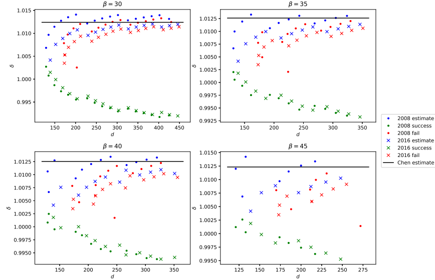
Figure 7.2: Plots of \delta for ternary secrets and \beta = 30, 35, 40, 45 .
