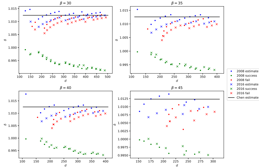
Figure 7.3: Plots of \delta for gaussian secrets and \beta = 30, 35, 40, 45 .
