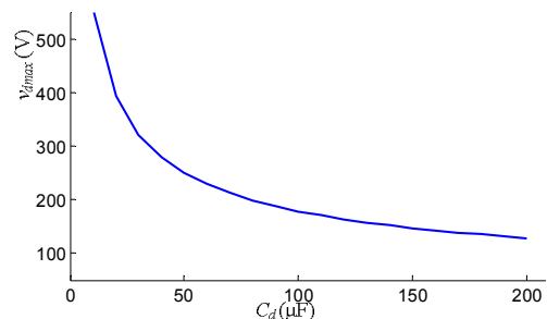
Fig. 6. Voltage stress versus the value of C_d .
