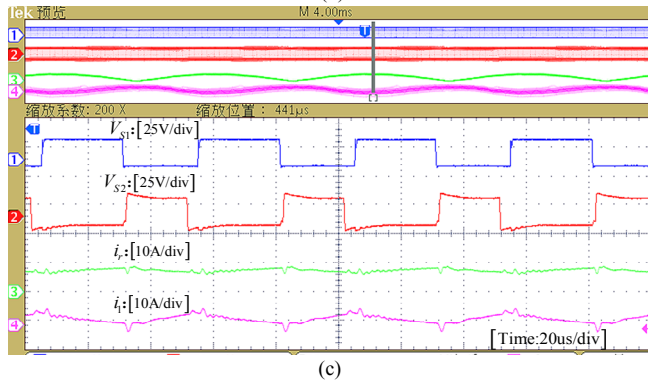
Fig. 13. Experimental waveforms of gate-emitter voltages, inductor currents i_r and i_l when the output voltage is 120V (the load power is 480 W). (a) Waveforms of V_{s1} , V_{s2} , i_r , and i_l . (b) Zoom-in waveforms of point A. (c) Zoom-in waveforms of point B.
