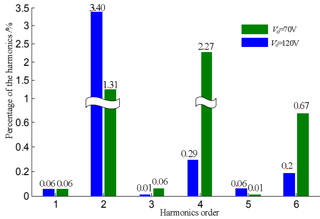
Fig. 12. Percentage of the output voltage harmonics versus its dc component.
