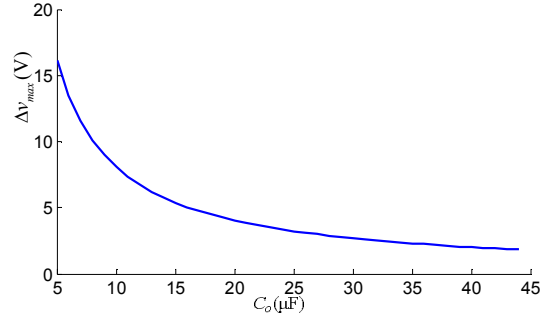
Fig. 8. Maximum value of the voltage ripple \Delta v_{max} versus the value of C_o .
