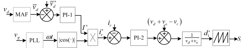
Fig. 4. Control scheme for the grid current.
