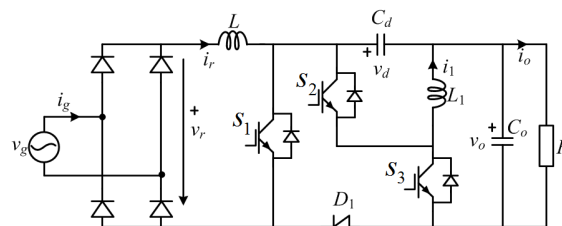
Fig. 1. Proposed circuit topology with wide output voltage and power decoupling capability.
