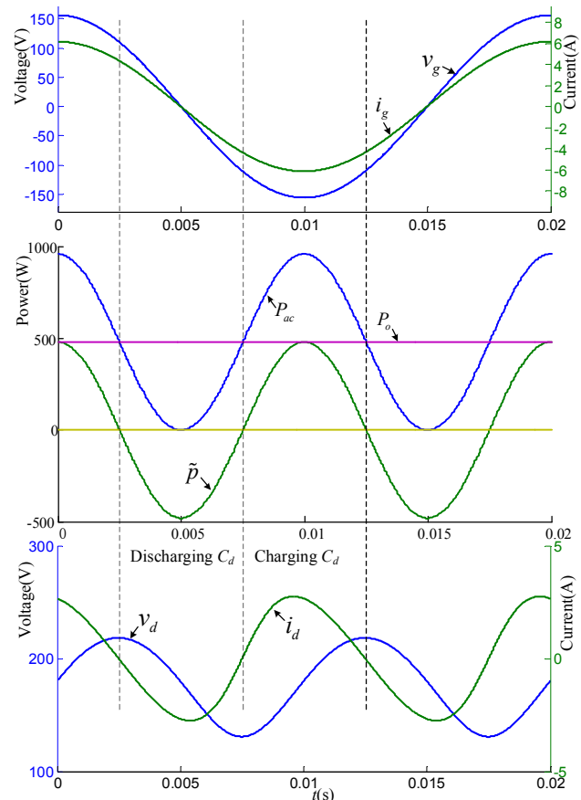
Fig. 3. Time domain waveforms of the grid voltage v_g , grid current i_g , power distribution, voltage v_d , and current i_d .
