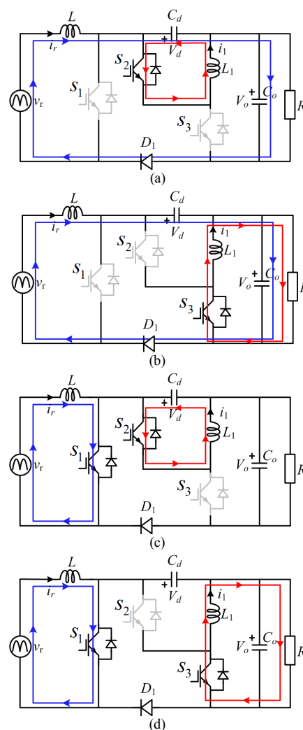
Fig. 2. Operating states of the proposed PFC rectifier. (a) State 1 ( S_1 =OFF, S_2 =ON, S_3 =OFF). (b) State 2 ( S_1 =OFF, S_2 =OFF, S_3 =ON). (c) State 3 ( S_1 =ON, S_2 =ON, S_3 =OFF). (d) State 4 ( S_1 =ON, S_2 =OFF, S_3 =ON).
