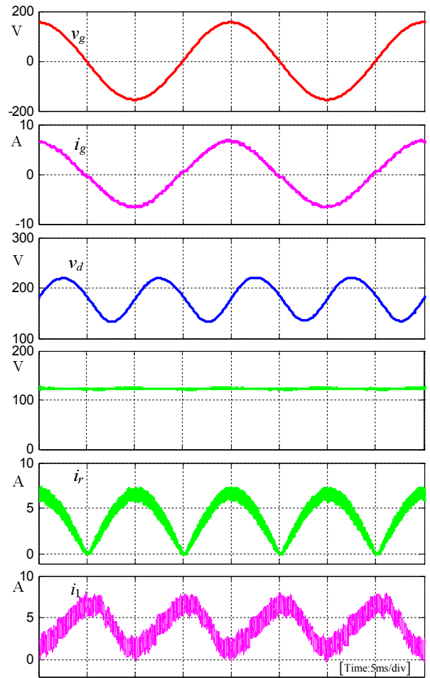
Fig. 9. Steady-state simulation waveforms of the grid voltage v_g , grid current i_g , capacitor voltage v_d , load voltage v_o , inductor current i_r , and inductor current i_l .
