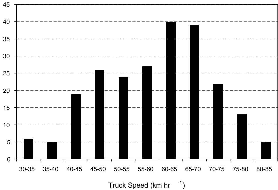
Figure 3. Truck speed distribution for the 226 HD trucks analyzed in this study, based on average values per truck through the tunnel.
