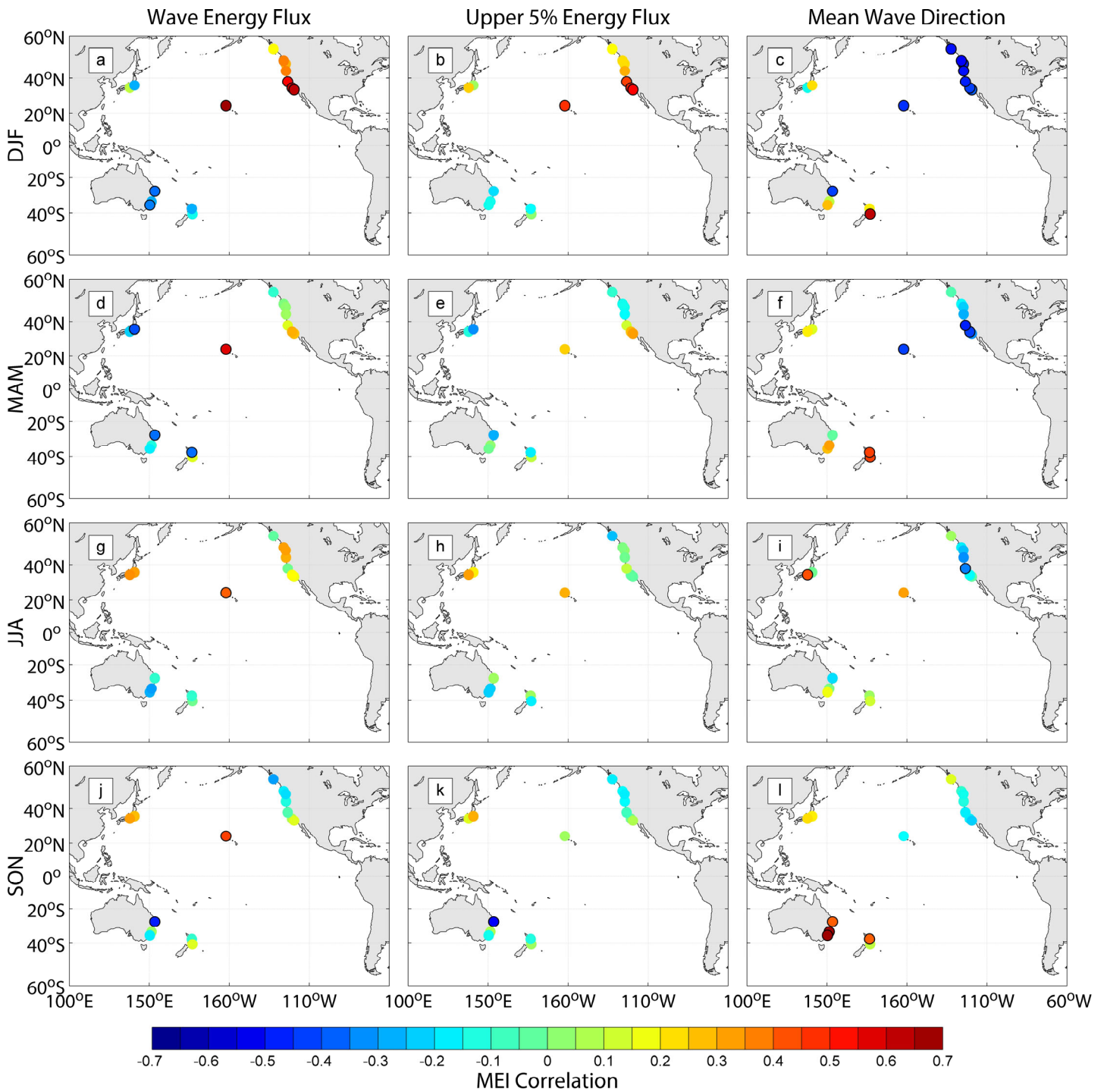
Figure 5. Wave metrics and MEI correlations. Correlation ( R ) between MEI and wave energy flux, upper 5% energy flux, and direction from sites across the Pacific Ocean basin for boreal winter (DJF), spring (MAM), summer (JJA), and fall (SON). Black outlines indicate significant correlations above the 95% confidence interval. (see Supplemental Fig. 7 for plots of all 12 indices)
