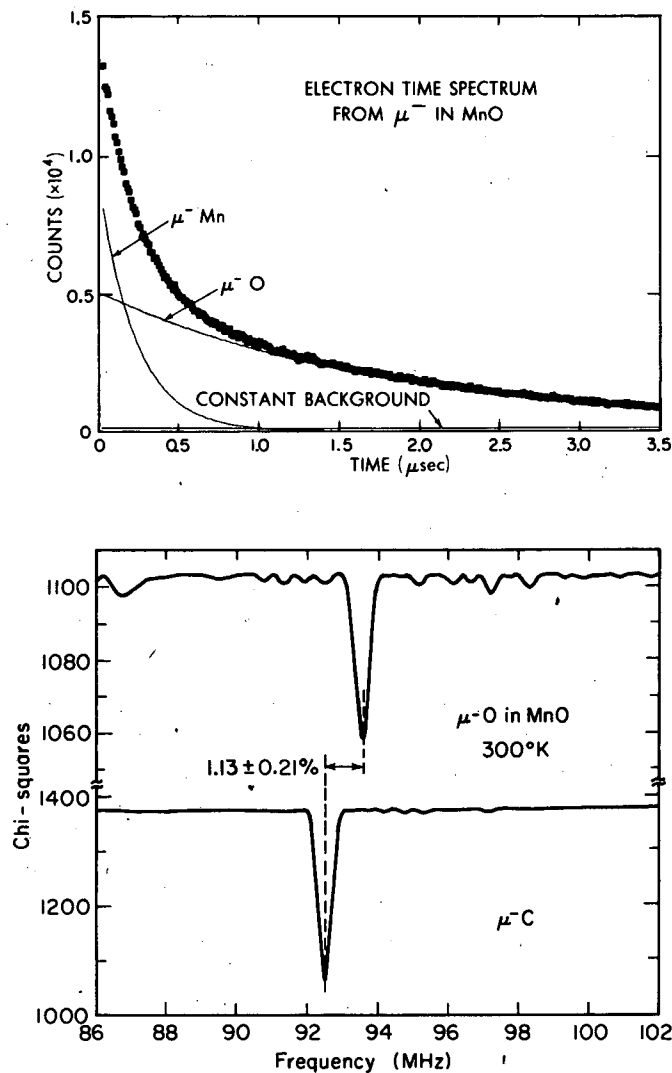
Fig. 5. Upper: Time spectrum of decay electrons from the muons stopped in a MnO target. The long-lived component comes from \mu^- \text{O} and the short-lived one from \mu^- \text{Mn} .
