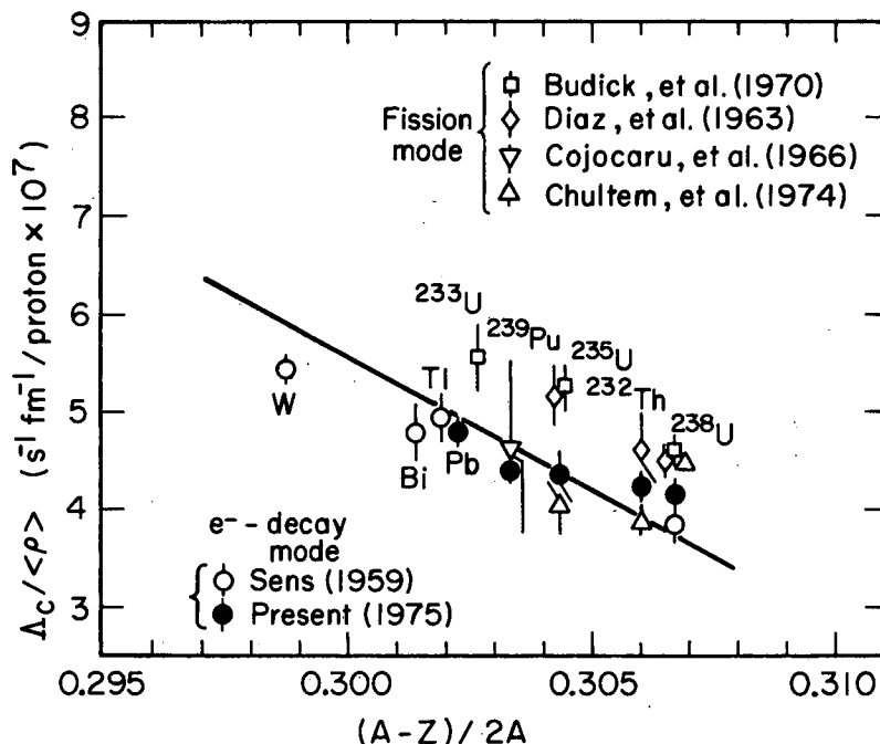
Fig. 6. Primakoff plot of muon capture rates in actinide region. The black circles are the present results. The lifetime of \mu^- Pb has also been determined to be 77.5 \pm 2.0 ns, and it is involved in this figure.
