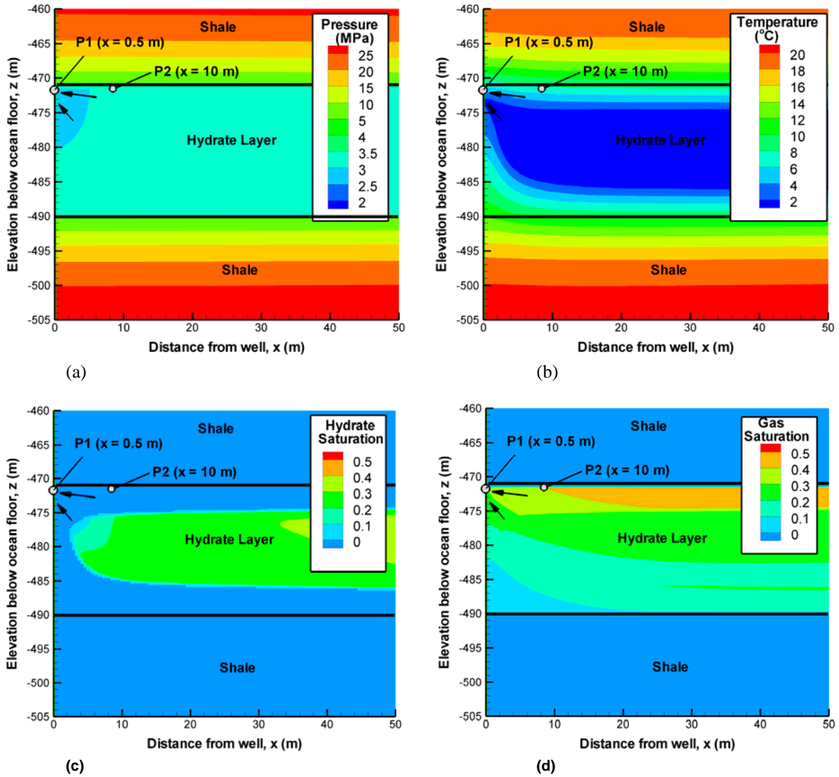
Figure 7 – Thermodynamic state after 6 months (180 days) of production for Case 1: (a) Pressure, (b) temperature, (c) hydrate saturation, and (d) gas (CH 4 ) saturation.
