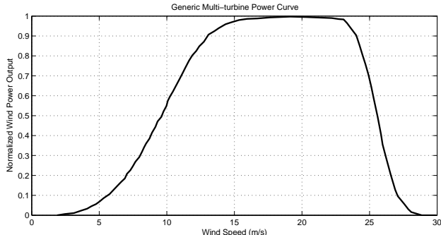
Figure 2: Generic multi-turbine power curve used to convert hub-height wind speed to wind power from Holttinen (2005).
