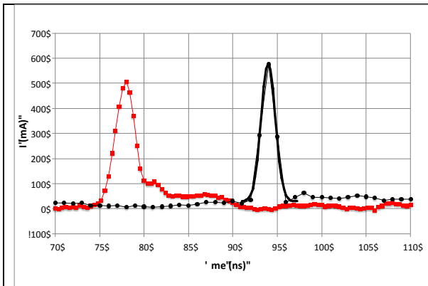
Figure 6: Faraday cup signals for two pulses. The pulse on the right followed induction cell tuning, which decreased the shoulder after the main peak. The fitted FWHM are 2.7 ns and 1.9 ns.
