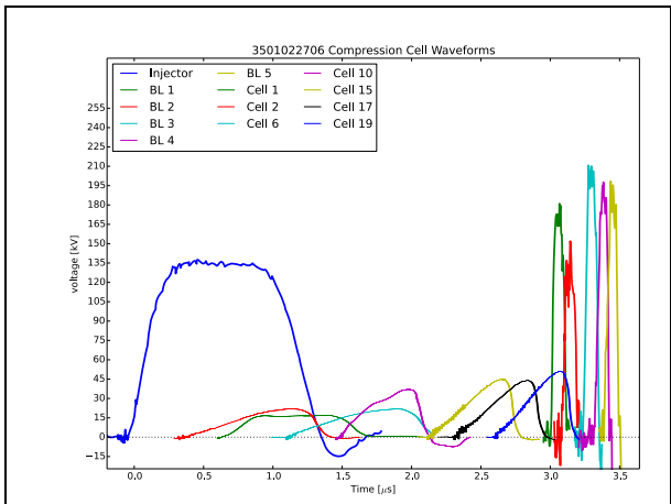
Figure 1: Voltage waveforms for each of the 12 acceleration gaps in NDCX-II.
