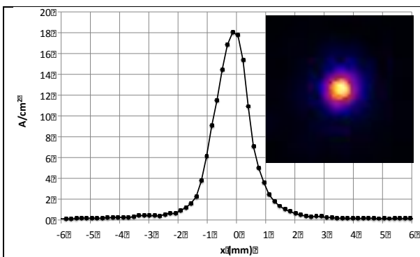
Figure 7: Beam distribution at the target plane measured with the Al 2 O 3 :Cr scintillator and gated CCD camera. The curve is a horizontal lineout near the center of the beam and the inset image (10x10 mm 2 ) shows the distribution details. (CCD pixel size = 0.17 mm on the scintillator).
