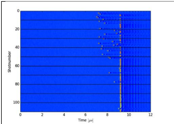
Figure 2: Blumlein timing for 110 successive shots. The voltage for shot numbers 1-80 was increased until the timing stabilized to 2.4 ns with only one outlier in 30 shots.
