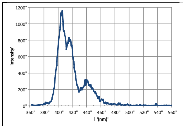
Figure 9: Ionoluminescence spectrum from YAP:Ce due to 1.2 MeV Li + ions bombarding in a few ns pulse. The diagnostic sensitivity decreases rapidly for \lambda < 400 nm due to the fiber optic coupling from the target chamber to the streak camera.
