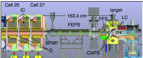
Figure 3: Side view of the end of the accelerator (cells 25-27) followed by the drift compression section, final focusing and target chamber. FEPS: Ferroelectric plasma source; G: acceleration gaps; LC: light collection and fiber optics diagnostics.
