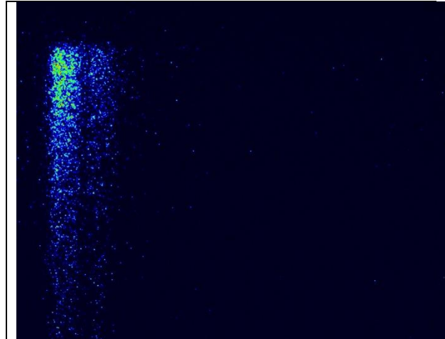
Figure 8: Ionoluminescence of YAP:Ce measured with a streaked optical spectrometer. The vertical time range is 100 ns and the abscissa range is 363 < \lambda < 800 nm. The optical fiber sensitivity drops sharply for \lambda < 400 nm.
