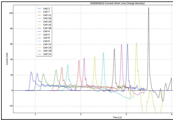
Figure 5: Current waveforms along the accelerator derived from the 15 capacitive beam position monitors and the inductive current monitors.
