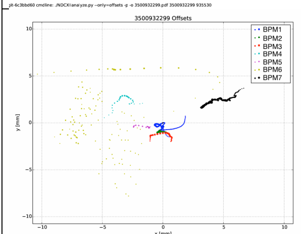
Figure 4: The centroid motion for a single bunch is shown at each of seven BPMs before (top) and after (bottom) dipole field adjustments.
