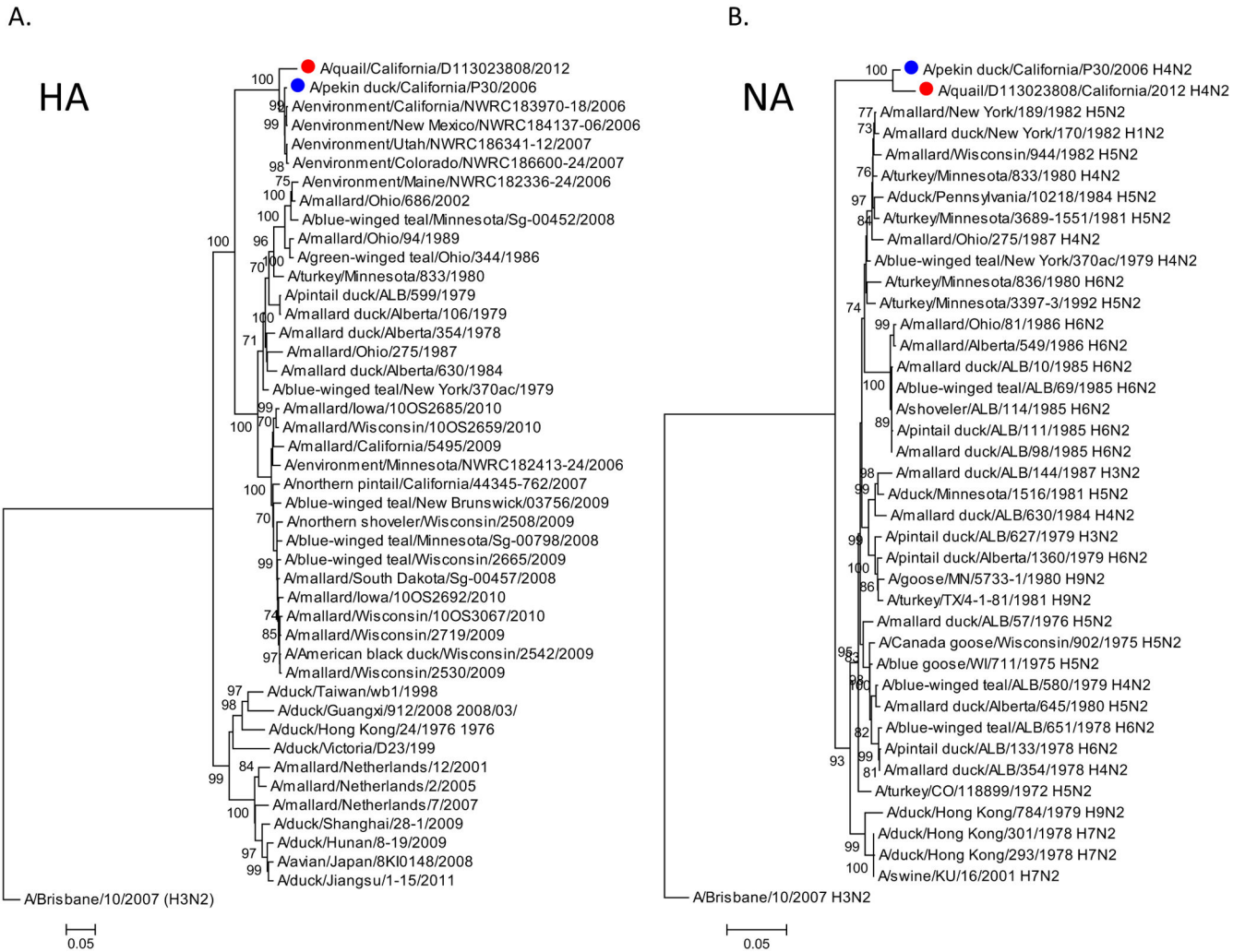
Figure 1. Origin of A /Quail/California/D113023808/2012 (H4N2) (Quail/CA12). The phylogenetic relationship of the (A) HA and (B) NA genes of Quail/CA12. The tree was constructed by using the neighborhood-joining method with a bootstrap value of 1000. The scale bar indicates the number of nucleotide substitutions.
