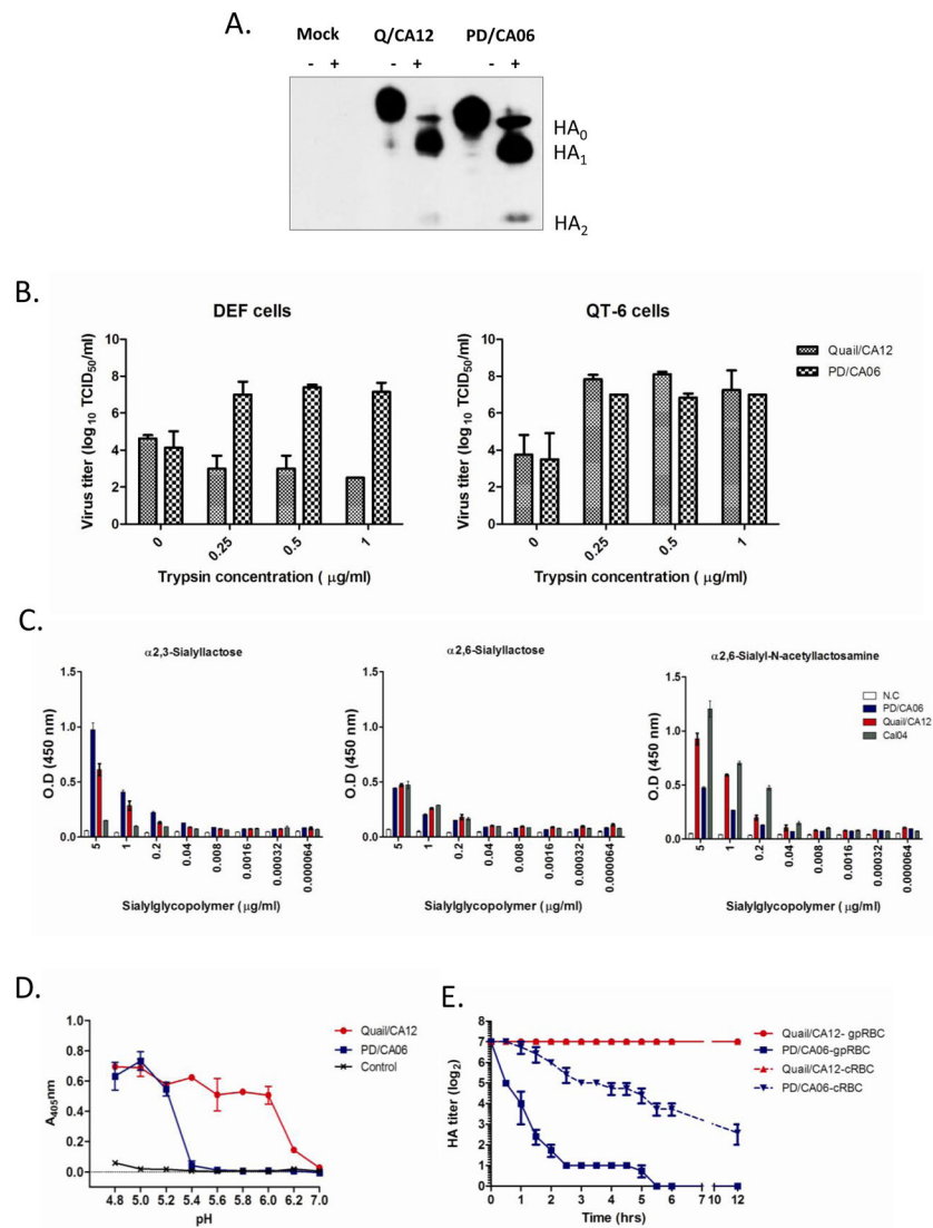
Figure 4. Biological features of the HA and NA of Quail/CA12 and PD/06. (A) Proteolytic cleavage of HA in the presence (+) and absence (-) of trypsin. (B) Replication in duck embryonic fibroblasts (DEF) (B) and quail-origin QT-6 cells (C) across a range of trypsin concentrations after 72 h. (C) Receptor-binding specificity (A) to \alpha 2,3- and \alpha 2,6-linked sialic acids was determined in a solid-phase binding assay. N.C denotes negative control. (D) Stability of the HA protein across a range of pH values was assessed by determining the pH at which virus fusion was triggered to cause hemolysis of RBCs. (E) NA activity was determined by a virus elution assay. GpRBC and cRBC indicate hemagglutination performed with guinea pig and chicken RBC respectively
