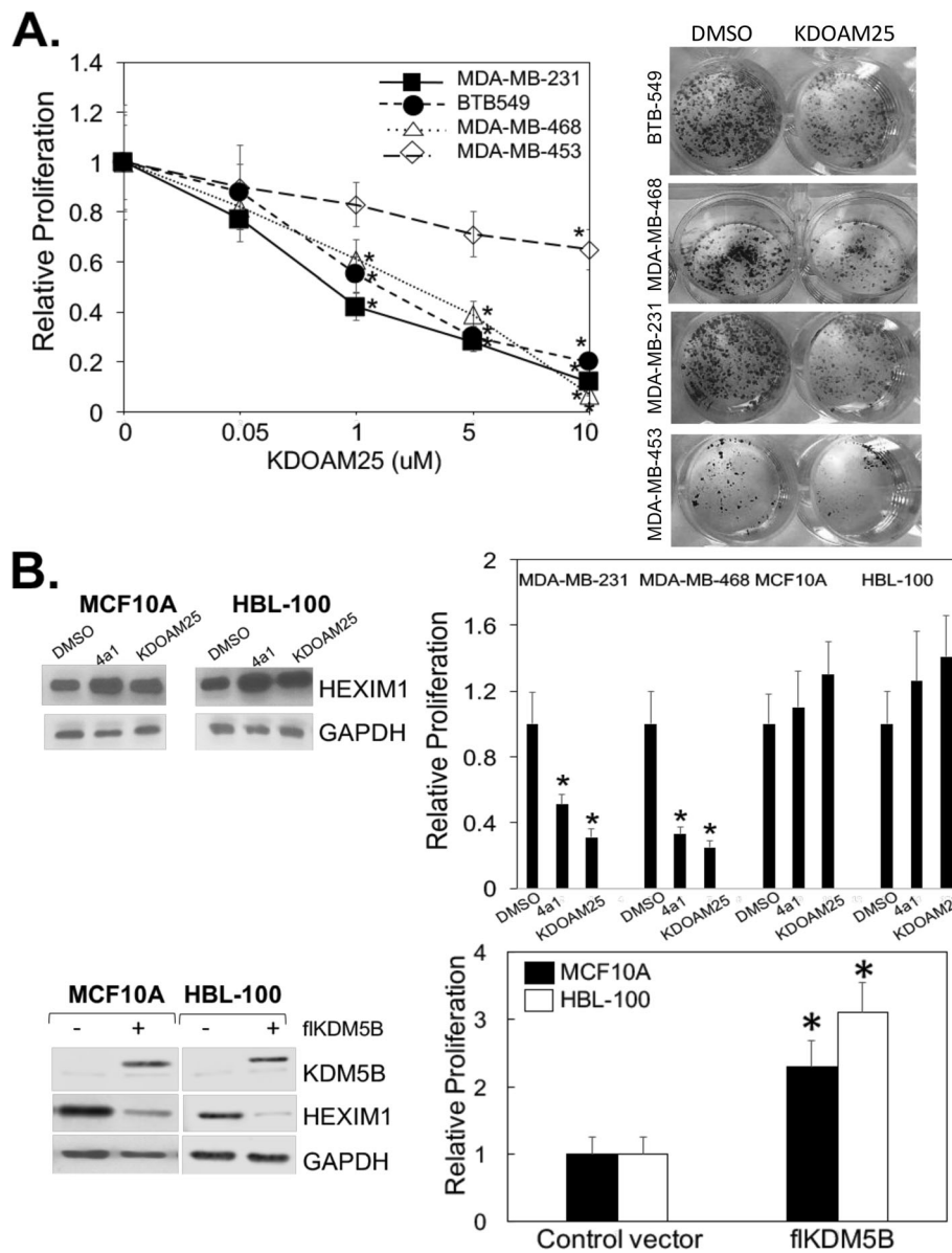
Fig. 5 Induction of HEXIM1 expression and inhibition of proliferation of TNBC subtypes by KDM5B inhibitors. a Left panel: TNBC lines were treated with DMSO or indicated concentrations of KDOAM25 for 6 days and subjected to MTT assays to assess proliferation. Right panel: TNBC lines were treated with DMSO or KDOAM25 (representing IC50) for 2 weeks and subjected to colony formation assays. b Different breast cell lines were transfected or treated with DMSO, 4a1 (100 μM), or KDOAM25 (500 nM) for 10 h and processed for western blot analyses of indicated proteins or subjected to MTT assays to assess proliferation. Figures are representative of at least three experiments. Upper panel: * P < 0.01 relative to DMSO-treated control of the same cell line based on t test. Lower panel: * P < 0.01 relative to cells of the same cell line transfected with control vector based on t test
