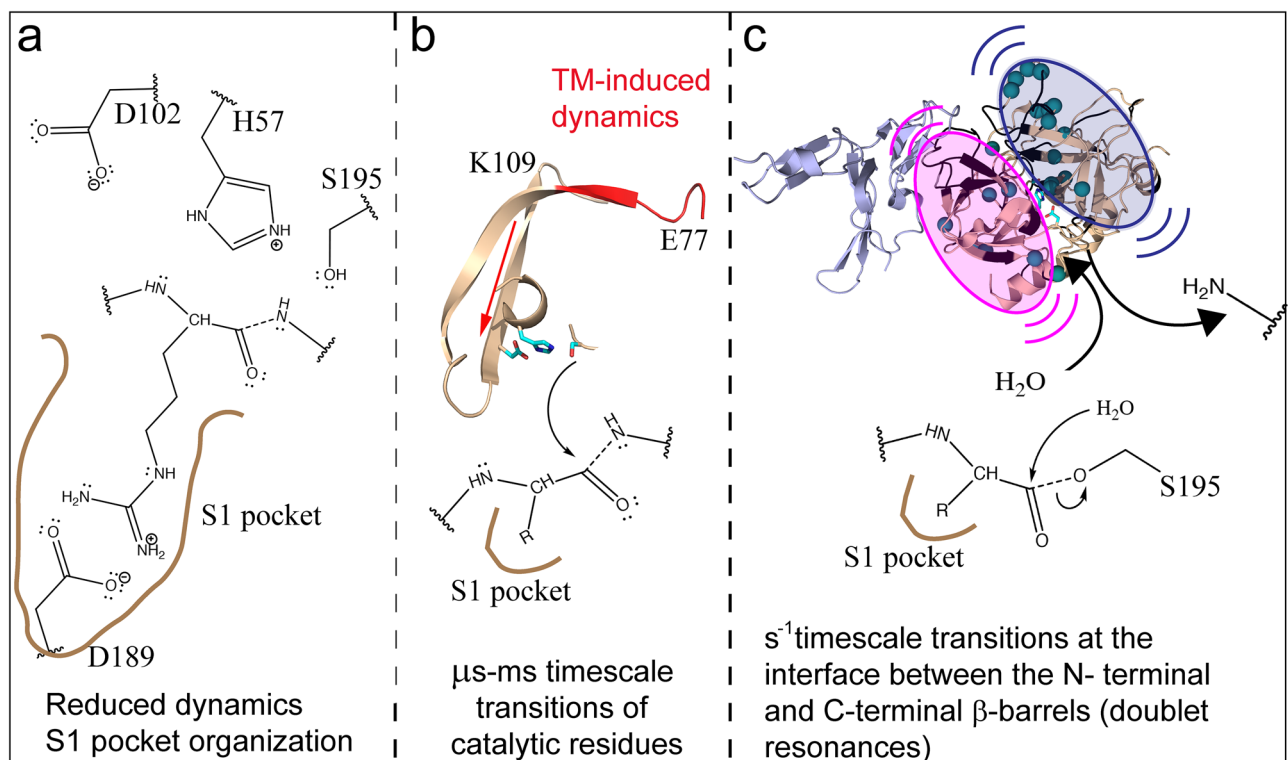
Figure 7. A model that describes the steps of the serine protease mechanism. (a) TM decreases dynamics in the substrate binding pocket to promote protein C binding. (b) TM induces \mu\text{s} - \text{ms} dynamics that may promote the optimal activity of the catalytic triad. The backbone of residues 77-84 CT (108-116seq) is colored red, and the backbone of residues 56-58 CT (78-80seq), 85-113 CT (117-146), and 195 CT (241seq) are colored wheat. The side chains of the catalytic triad are shown as cyan sticks. (c) Doublet resonances indicate TM induced dynamics on the seconds time scale of the N-terminal (pink oval) and C-terminal (blue oval) \beta -barrels that may be required for the release of the first product from Ser 195 CT and entry of H 2 O into the active site for acyl enzyme hydrolysis.
