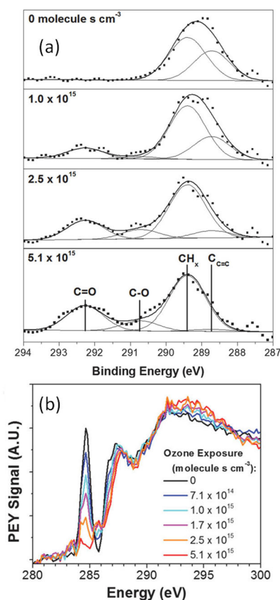
Fig. 22. (a) XPS spectra of squalene nanoparticles at different oxidation conditions. (b) NEXAFS spectra of carbon K edge of squalene nanoparticles at various ozone exposures. Reprinted with permission from ref. 162. Copyright (2016) American Chemical Society.
