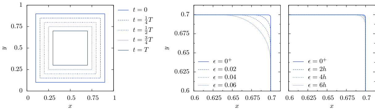
Figure 3.9. Evolution of a square shrinking with unit speed ( T = \frac{1}{5} ) (left), and the solution at time t = T obtained on the same grid ( h = 1/512 ), with \epsilon fixed (middle) and \epsilon coupled to h (right).
