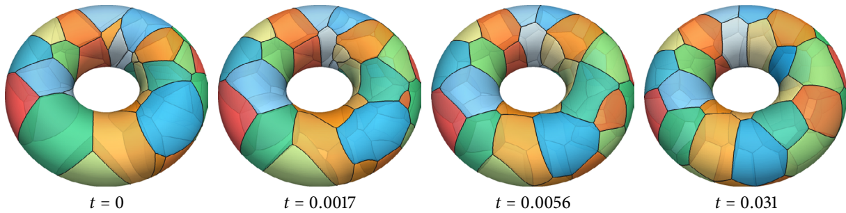
Figure 4.17. Mean curvature flow with volume targeting in a torus.
