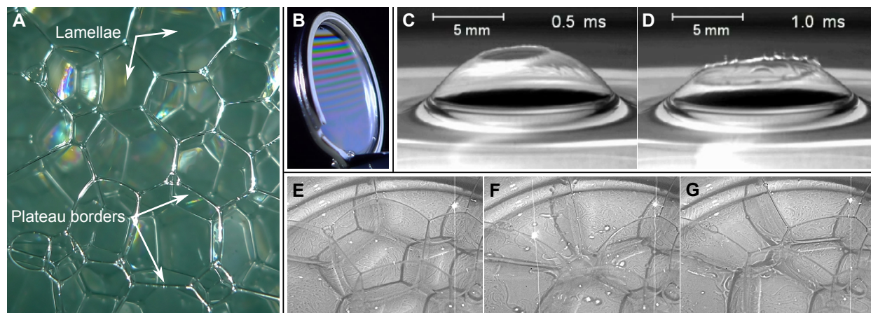
Figure 6.1. Physics of foam drainage. (a) A foam of soap bubbles made with common washing detergent. (b) Drainage and thin-film interference – a keyring suspended in soap solution makes a film, which then drains due to gravity. The subsequent variations in film thickness create interference patterns when lit with white light. This image was captured with a consumer digital camera. (c,d) Rupture of a lamella; reproduced from [90] by permission from Macmillan Publishers Ltd, Nature , copyright 2010. (e,f,g) Rearrangement – a lamella (centre of (E)) bursts, leading to macroscopic rearrangement of a foam. The frames are from a movie captured using a CCD black and white camera.
