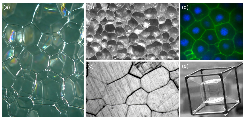
Figure 1.1. Examples of multi-region physics. (a) A soap bubble foam made with common washing detergent. (b) Metallic foam made out of aluminium (reproduced from [6]). (c) Grains in a polycrystalline metal (reproduced from [7]). (d) Cells in a zebrafish, stained so that the cell membranes are green and nuclei blue (reproduced with permission from [8]). (e) Minimal surfaces formed by steady-state soap films.
