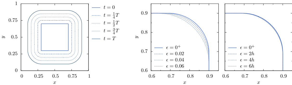
Figure 3.7. Evolution of an initially square interface expanding with unit speed ( T = \frac{1}{5} ) (left), and the solution at time t = T obtained on the same grid ( h = 1/512 ), with \epsilon fixed (middle) and \epsilon coupled to h (right).
