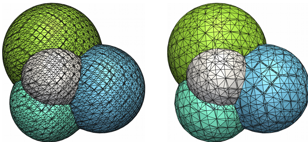
Figure 5.2. A multiphase mesh of a five-phase system of four spheres, using the polygon chopping method (Algorithm 3). Four pairwise surfaces and three quadruple point junctions are visible. (Left) Using the standard decomposition of dividing a grid cell into six tetrahedra, without vertex snapping. (Right) Using the body centred cubic lattice, with vertex snapping.
