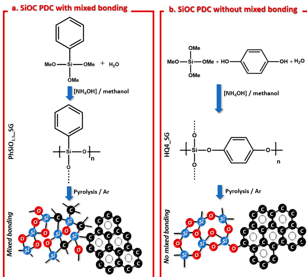
Figure 1. (a) Synthesis of PhSiO 1.5_SG using trimethoxyphenylsilane (TMOPS) precursor to synthesize a polymer with the phenyl group bonding directly to silicon resulting in a SiOC PDC with mixed bonding. (b) Synthesis of HQ4_SG using hydroquinone (HQ) and tetramethylorthosilicate (TMOS) precursors to synthesize a polymer with the phenyl group bonding to the silicon through Si-O-C bridges resulting in a SiOC PDC without mixed bonding.
