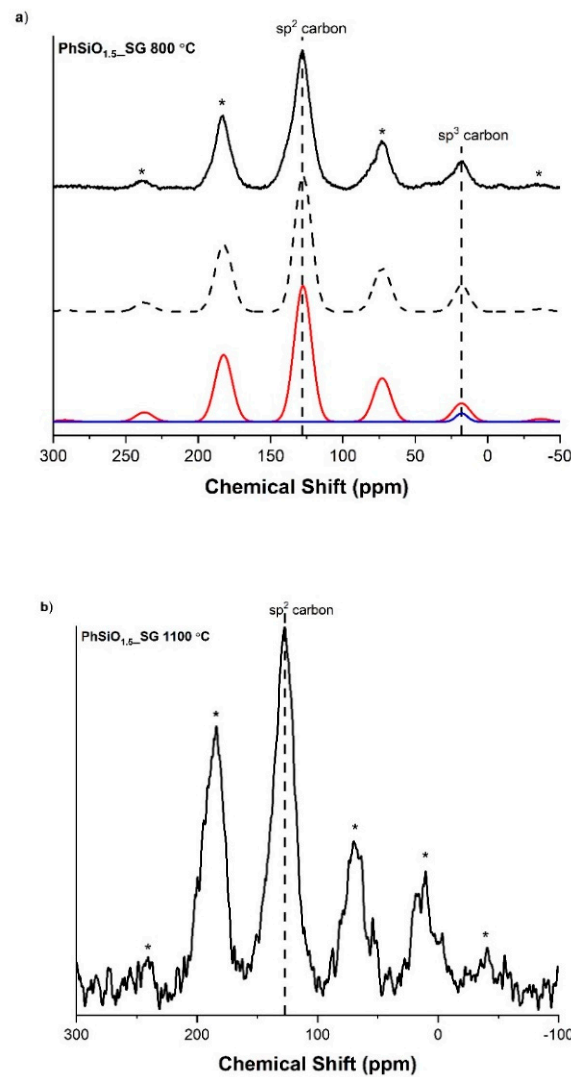
Figure 7. ^{13}\text{C}(^1\text{H}) CPMAS NMR for \text{PhSiO}_{1.5}\text{SG} samples. (a) Sample pyrolyzed to 800\text{ }^\circ\text{C} with peaks at \sim 127 ppm and 18 ppm, corresponding to \text{sp}^2 hybridized carbon and \text{sp}^3 hybridized carbon, respectively. (b) Sample pyrolyzed to 1100\text{ }^\circ\text{C} with an isotropic peak at \sim 127 ppm, corresponding to \text{sp}^2 hybridized carbon. The stars * denote spinning side bands.
