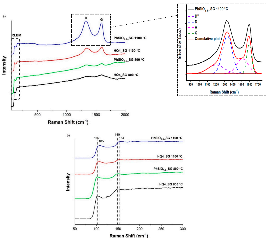
Figure 9. Raman spectra of PhSiO 1.5 -SG and HQ4_SG samples. (a) The entire spectra from 50 to 2000\text{ cm}^{-1} with inset showing the Raman fitting of PhSiO 1.5 -SG 1100\text{ }^\circ\text{C} and (b) the spectra from 50 to 300\text{ cm}^{-1} to show details of the RLBM bands.
