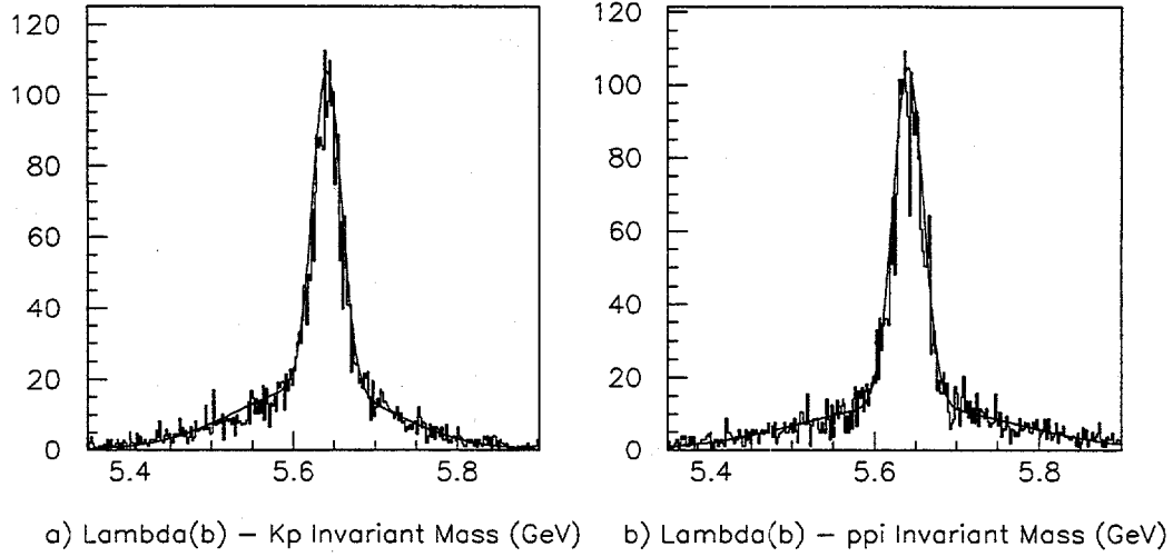
Figure 4.6: Results of the fit to the Monte Carlo generated \Lambda_b dihadron invariant mass spectra. (Units are in GeV.)
