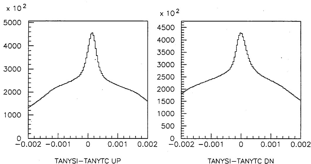
Figure 3.42: Distribution of \Delta Y_{\text{slope}} for a subset of the hadron data set. The left (right) plot shows the distribution for the upper (lower) arm of the silicon micro-vertex detector.
