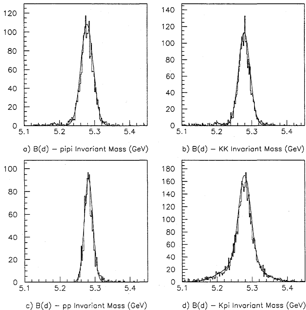
Figure 4.4: Results of the fit to the Monte Carlo generated B_d dihadron invariant mass spectra. (Units are in GeV.)
