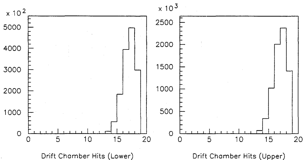
Figure 3.6: Distribution of the number of drift chamber hits in accepted hadron tracks. The distribution for tracks in the lower (upper) arm of the spectrometer are on the left (right).
