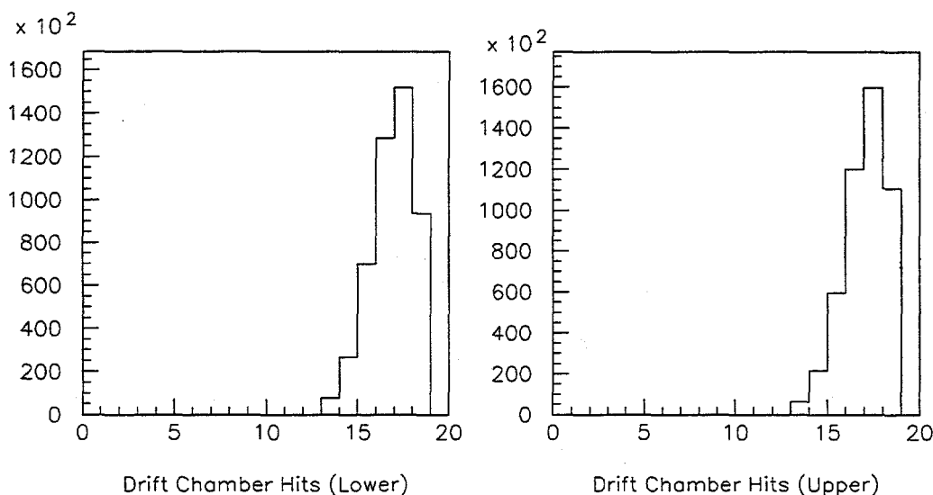
Figure 3.5: Distribution of the number of drift chamber hits in accepted muon tracks. The distribution for tracks in the lower (upper) arm of the spectrometer are on the left (right).
