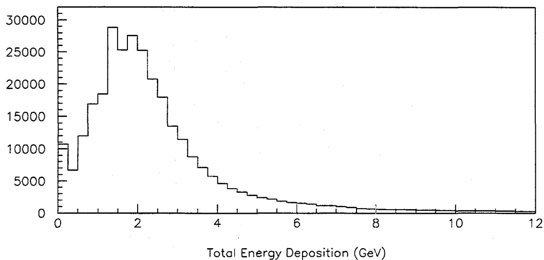
Figure 3.21: Distribution of the total energy deposited by good muons in the calorimeter.
