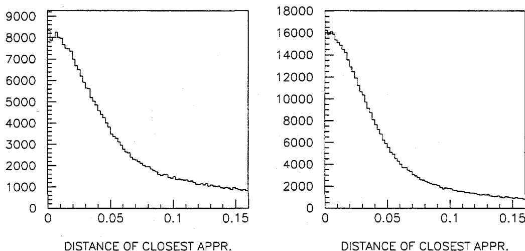
Figure 3.63: Distribution of the distance of closest approach for opposite-sign muon tracks (left) and hadron tracks (right), from a subset of the data, used in the final event cut. (Units are in inches.)
