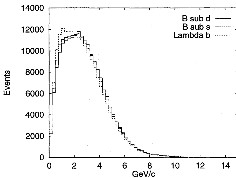
Figure 1.12: Center-of-mass P_t spectrum for B_d , B_s , and \Lambda_b hadrons produced in the interaction of 800 GeV protons with a fixed target (Monte Carlo).
