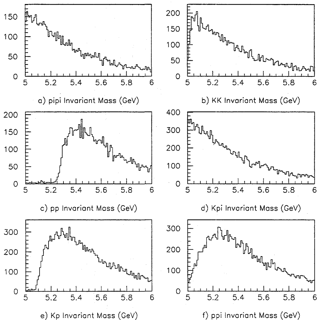
Figure 4.8: Plots of the different dihadron invariant mass spectra with loose cuts. (Units are in GeV.)
