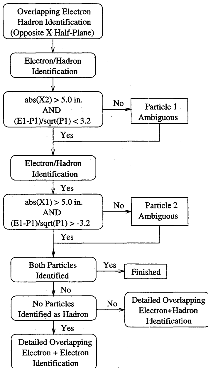
Figure 3.26: Flow chart of the opposite X half-plane overlapping electron-hadron identification algorithm.
