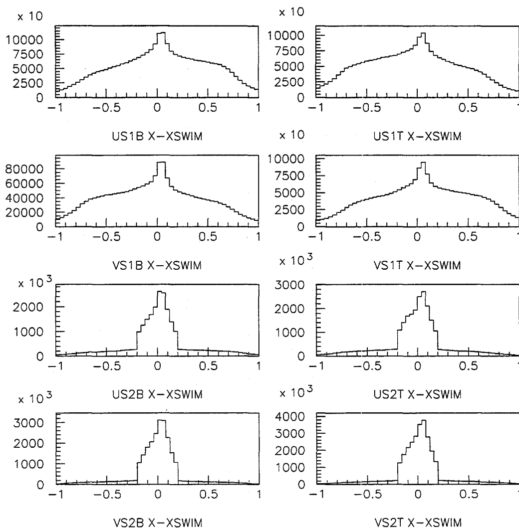
Figure 3.50: Distribution of the distances between the closest silicon hits on the various U/V planes and the iterated X position of the spectrometer track at the respective planes for a subset of the hadron data set. (Units are in inches.)
