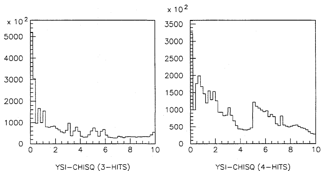
Figure 3.46: Distribution of the \chi^2 per degree of freedom for 3 and 4 hit candidate Y-tracks in a subset of the hadron data set.
