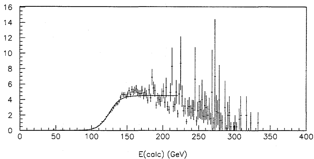
Figure 3.103: Ratio of the distributions of E_{calc} for events triggered by E_H and E_L . (Linear scale.)
