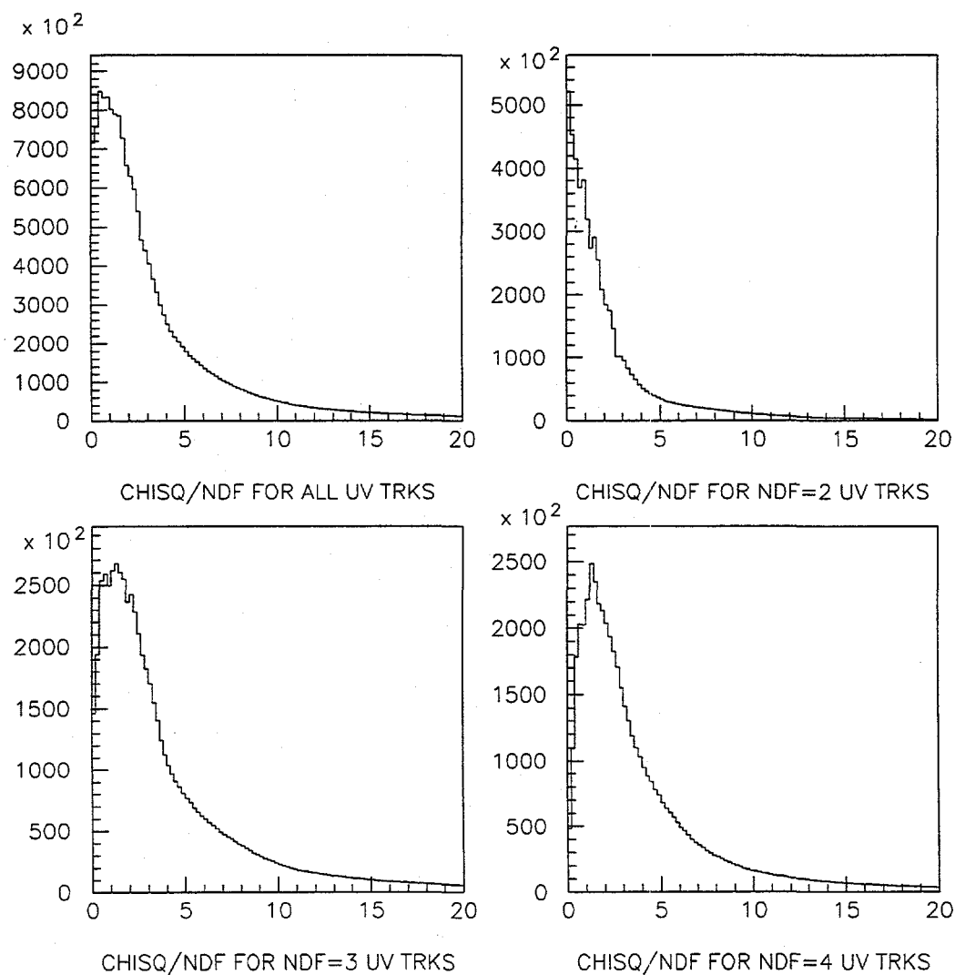
Figure 3.56: Distributions of the \chi^2 per degree of freedom for tracks with 6 or more hits, 6 hits, 7 hits and 8 hits for a subset of the hadron data set.
