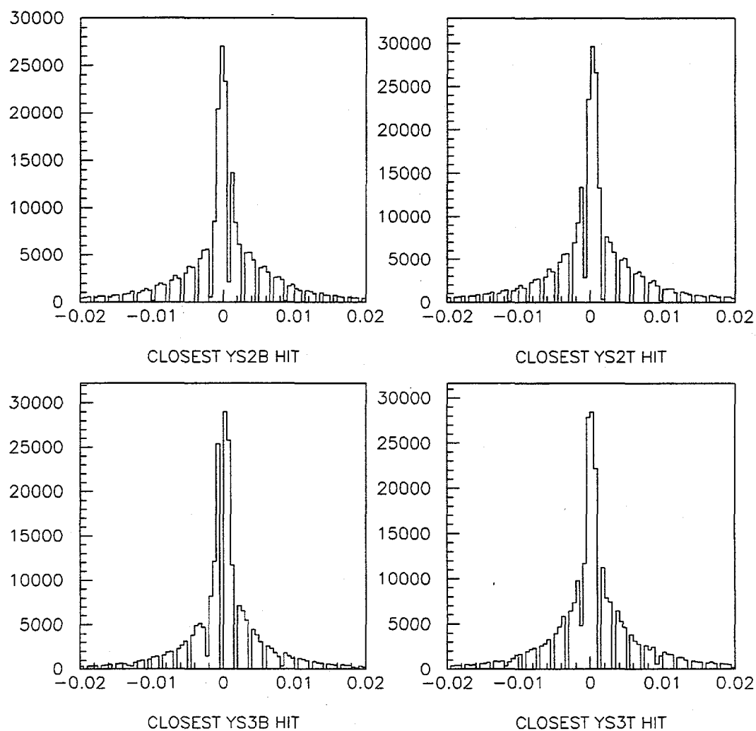
Figure 3.75: Distribution of the distances between the closest hits on the non-seed silicon Y planes and the candidate Y-track for Monte Carlo generated prompt J/\psi decays to two muons. (Units are in inches.)
