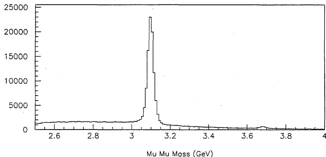
Figure 3.115: Invariant mass spectrum for events where both particles were identified as muons only and where the average silicon hit multiplicity was less than 7. (Units are in GeV.)
