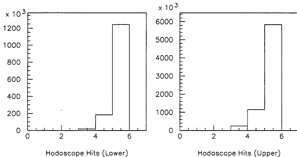
Figure 3.8: Distribution of the number of hodoscope hits in accepted hadron tracks. The distribution for tracks in the lower (upper) arm of the spectrometer are on the left (right).
