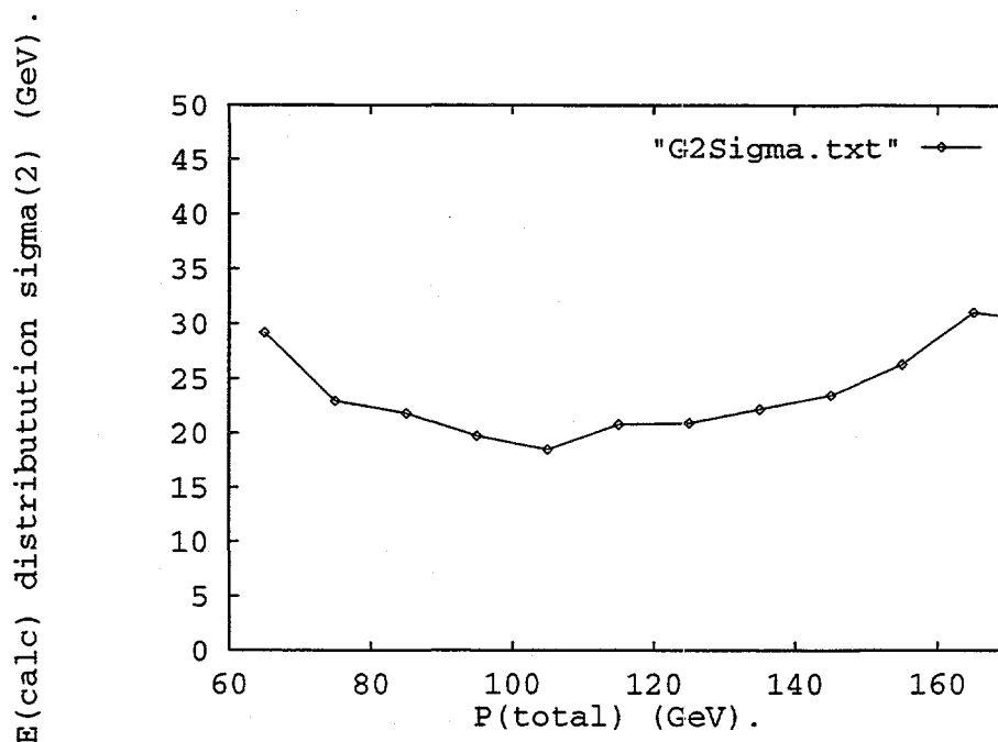
Figure 3.109: Variance ( \sigma_2 ) of the second Gaussian in the distribution of E_{calc} as a function of P_{total} for events triggered by E_L .
