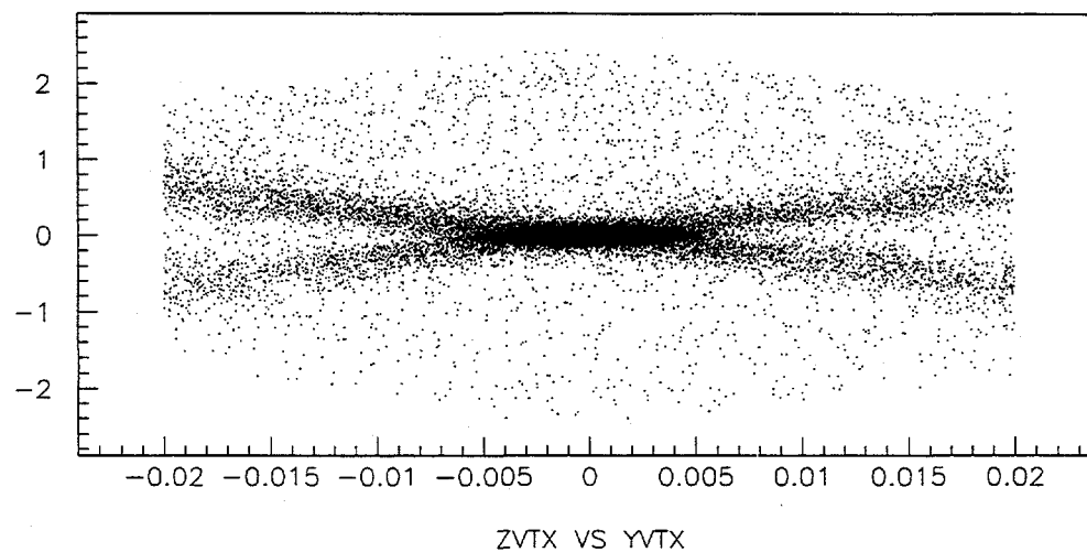
Figure 3.117: A scatter plot of the vertex Z versus Y position for dimuon events where the average silicon hit multiplicity is greater than or equal to 7. (Units are in inches.)
