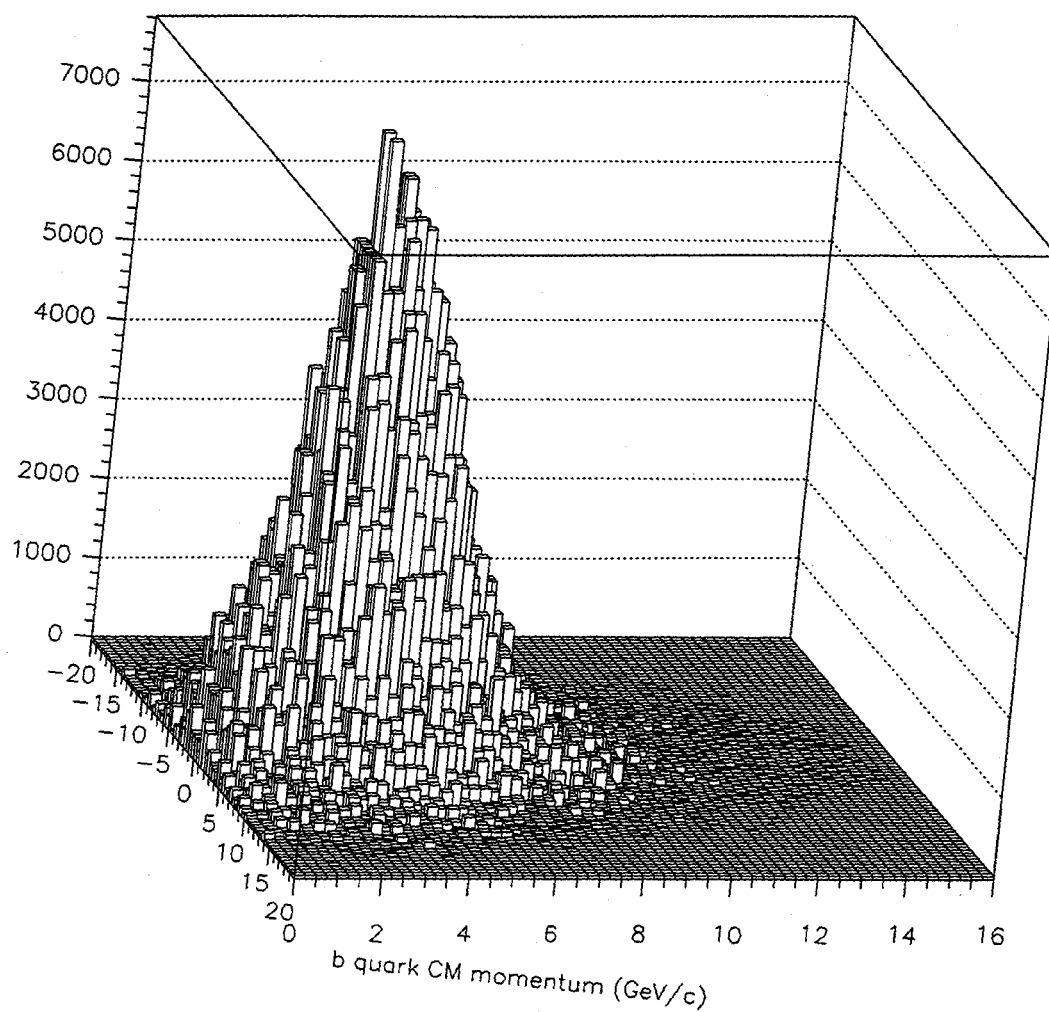
Figure 3.66: Production (P_t, P_t) spectrum (center of mass) for b -quarks produced in proton on proton interaction (Monte Carlo). The P_t axis is on the bottom with the range (0,16), the P_t axis is on the left with the range (-20,20).
