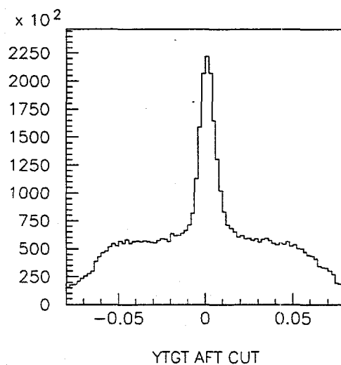
Figure 3.73: Distribution of y_{target} - y_{track}(z_{target}) for Monte Carlo generated prompt J/\psi decays to two muons. (Units are in inches.)
