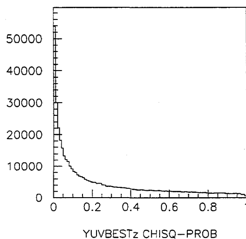
Figure 3.86: Distribution of the probability for the track fit \chi^2 per degree of freedom, for Monte Carlo generated prompt J/\psi decays to two muons, used in the final silicon track cut.
