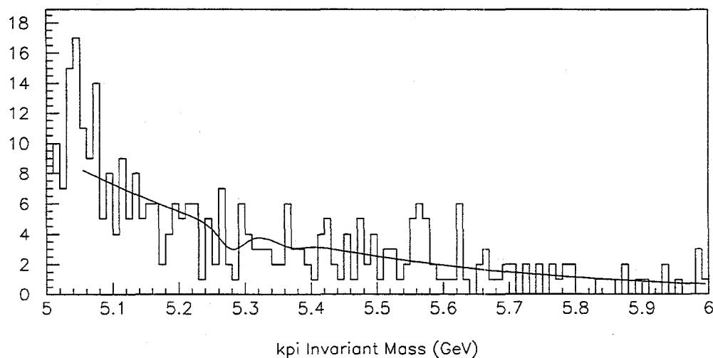
Figure 4.15: Results of the maximum likelihood fit to the invariant mass spectrum of the dihadron events assuming one pion and one kaon in the event. (Units are in GeV.)
