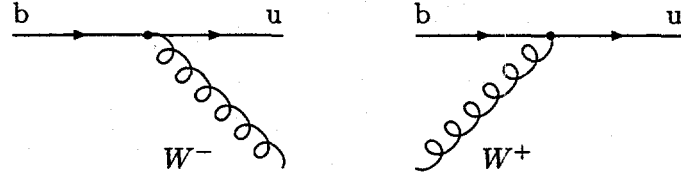
Figure 1.1: W emission/absorption diagrams.
