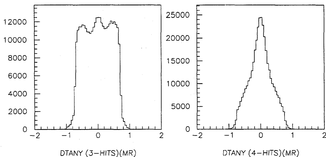
Figure 3.77: Distribution of \Delta Y_{\text{slope}} for Monte Carlo generated prompt J/\psi decays to two muons. The left plot shows the distribution for tracks with 3 hits and the right for 4 hit tracks. (Units are in milli-radians.)
