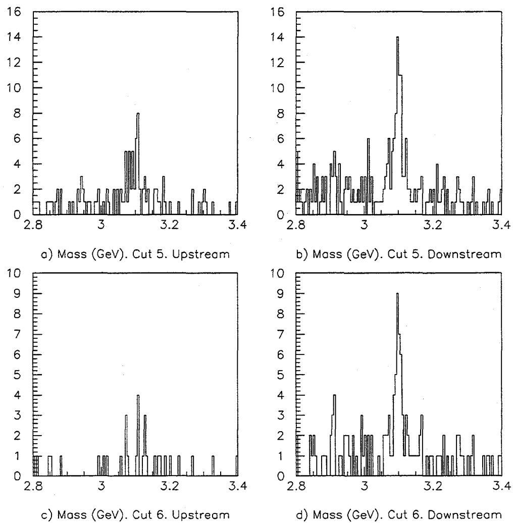
Figure 3.120: Invariant mass plots for successively tighter values of the impact parameter and Z vertex cuts.
