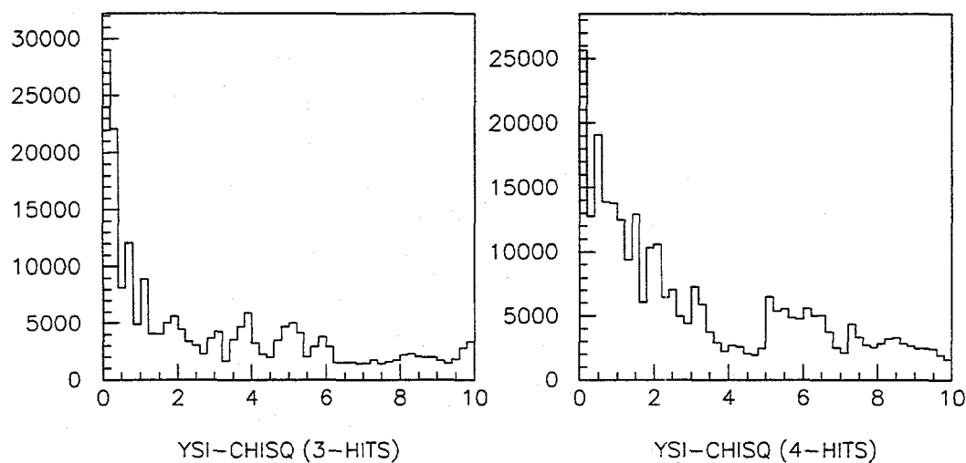
Figure 3.76: Distribution of the \chi^2 per degree of freedom for 3 and 4 hit candidate Y-tracks for Monte Carlo generated prompt J/\psi decays to two muons.
