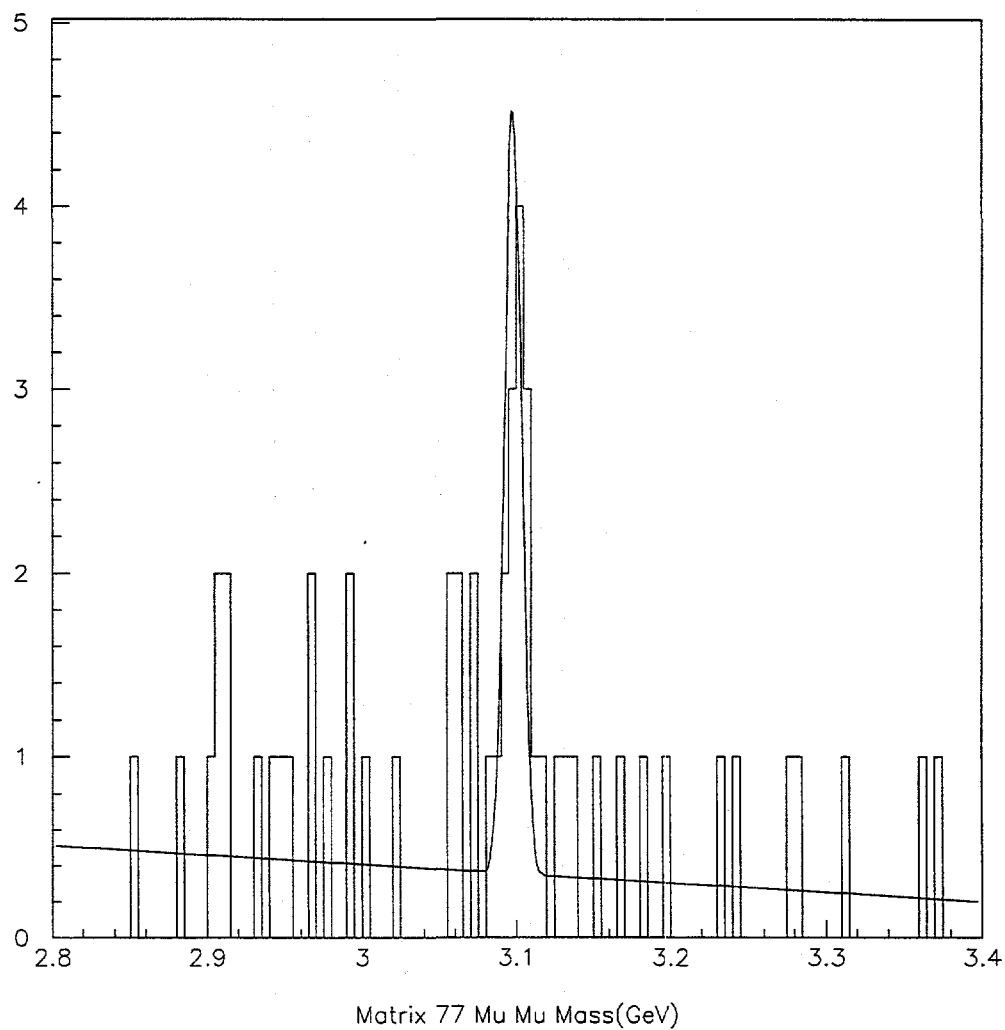
Figure 4.3: Results of the fit of a single fixed width Gaussian and a linear background to the dimuon invariant mass spectrum from run period 2. (Units are in GeV.)
