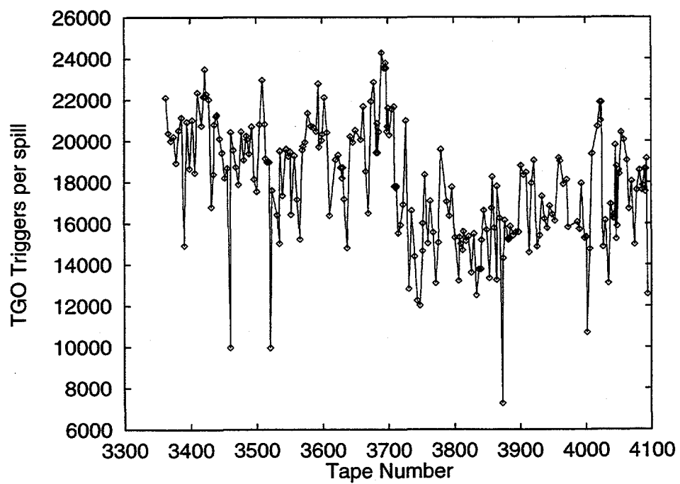
Figure 2.10: Average number of TGO triggers per spill as a function of tape number.
