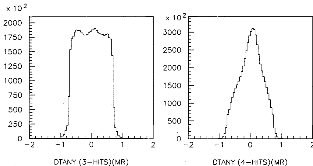
Figure 3.48: Distribution of \Delta Y_{\text{slope}} for a subset of the hadron data set. The left plot shows the distribution for tracks with 3 hits and the right for 4 hit tracks. (Units are in milli-radians.)
