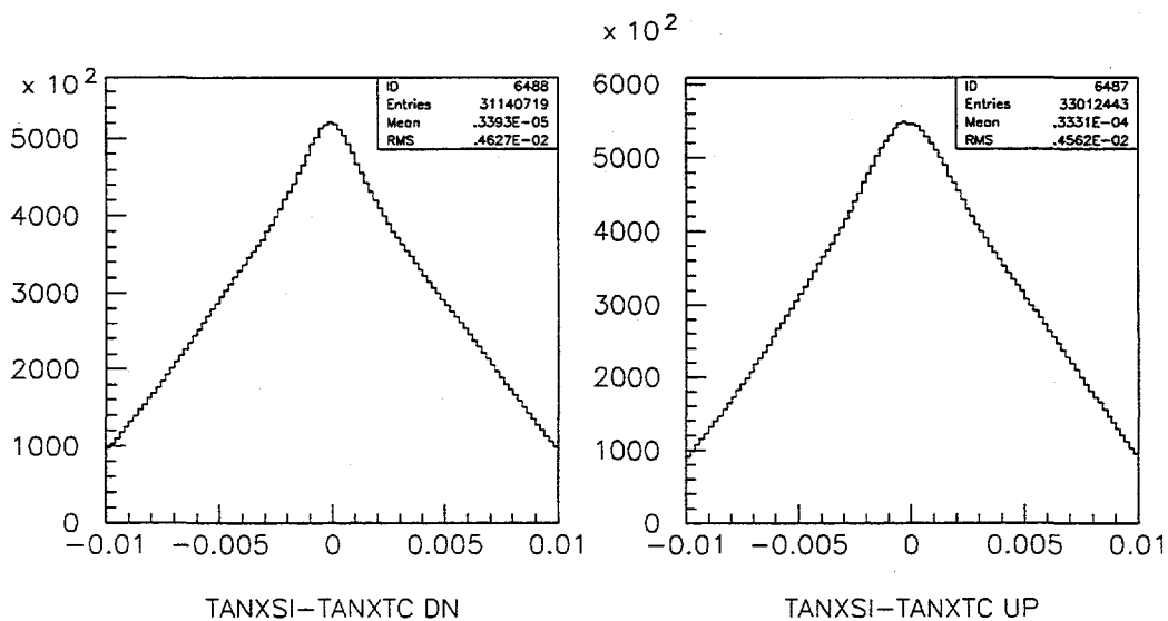
Figure 3.52: Distribution of \Delta X_{\text{slope}} for the muon data set. The left (right) plot shows the distribution for tracks in the lower (upper) arm of the silicon detector.
