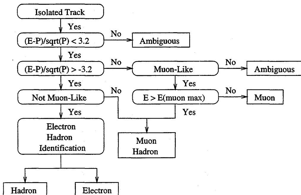
Figure 3.20: Flow chart of the calorimeter isolated particle identification algorithm.
