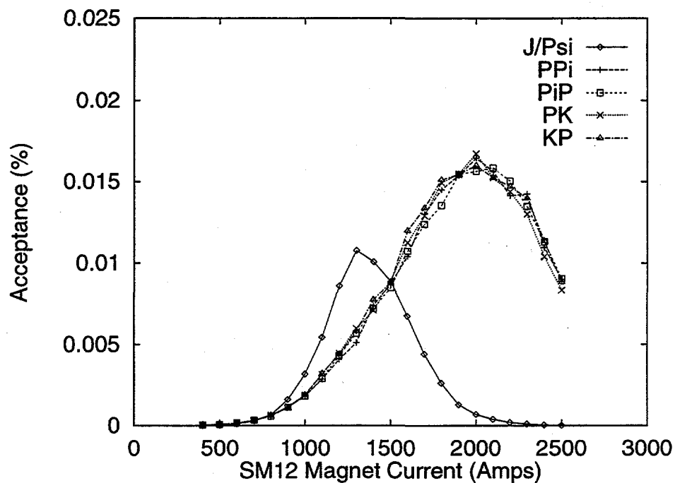
Figure 2.5: Acceptance of the spectrometer for various \Lambda_b decays as a function of SM12 current.
