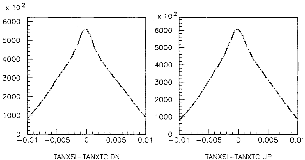
Figure 3.53: Distribution of \Delta X_{\text{slope}} for a subset of the hadron data set. The left (right) plot shows the distribution for tracks in the lower (upper) arm of the silicon detector.
