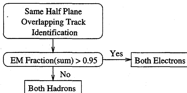
Figure 3.29: Flow chart of the same X half-plane overlapping electron hadron plane identification algorithm.
