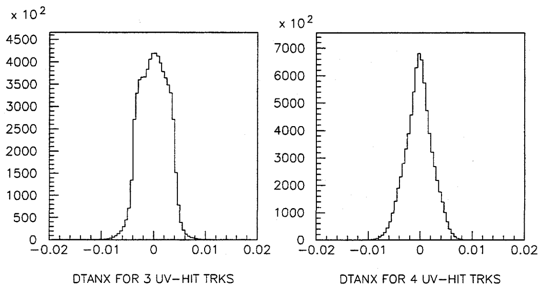
Figure 3.57: Distribution of \Delta X_{\text{slope}} for a subset of the muon data set. The left plot shows the distribution for 3-hit UV tracks and the right, for 4-hit UV tracks.
