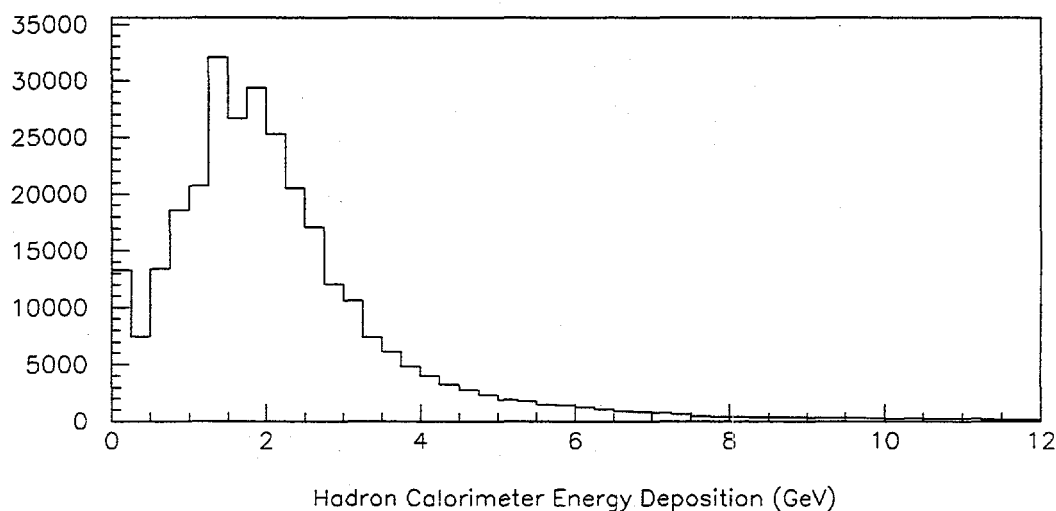
Figure 3.14: Distribution of the energy deposited in the hadron calorimeter by good muons.
