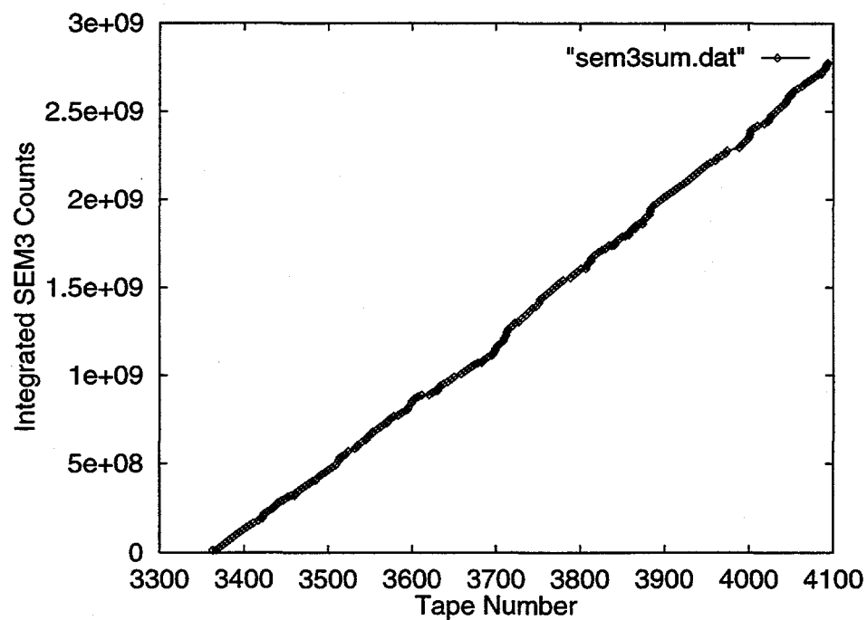
Figure 2.7: Integrated number of incident protons (in SEM3 counts) as a function of tape number.
