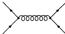
Figure 1.8: Quark - anti-quark diagram.
