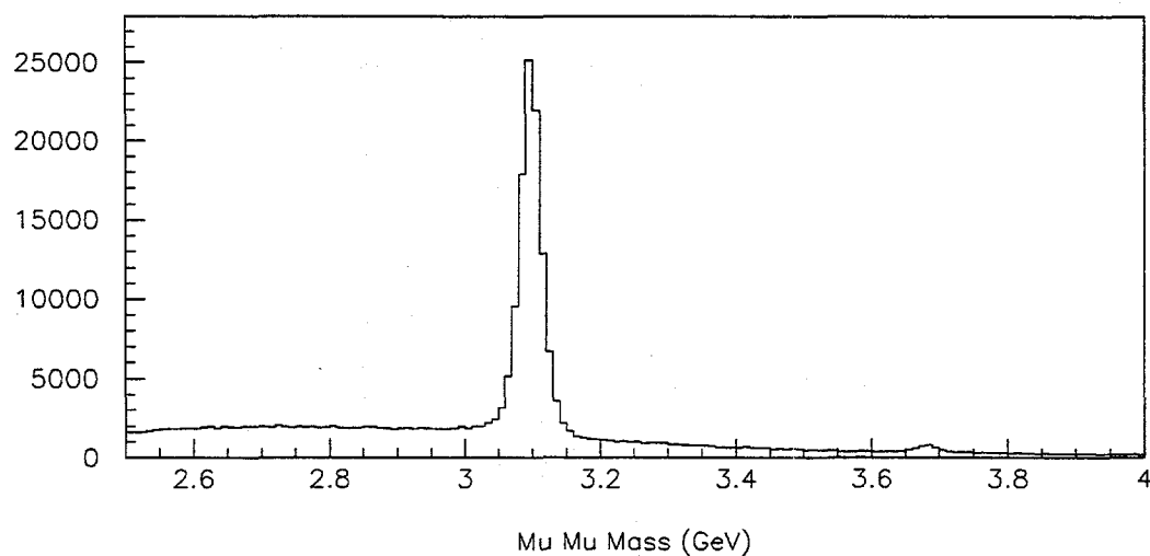
Figure 3.113: Invariant mass spectrum for events where both particles were identified as muons only. (Units are in GeV.)
