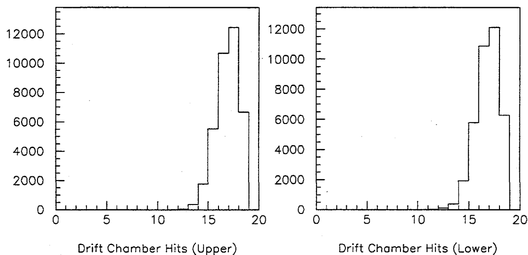
Figure 3.89: Distribution of the number of drift chamber hits in accepted upper (left) and lower (right) arm muon tracks for Monte Carlo generated prompt J/\psi decays to \mu^+\mu^- .
