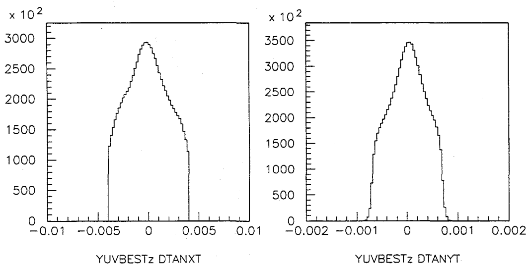
Figure 3.60: Distribution of \Delta X_{\text{slope}} (left) and \Delta Y_{\text{slope}} (right) for a subset of the muon data set before the final cut.
