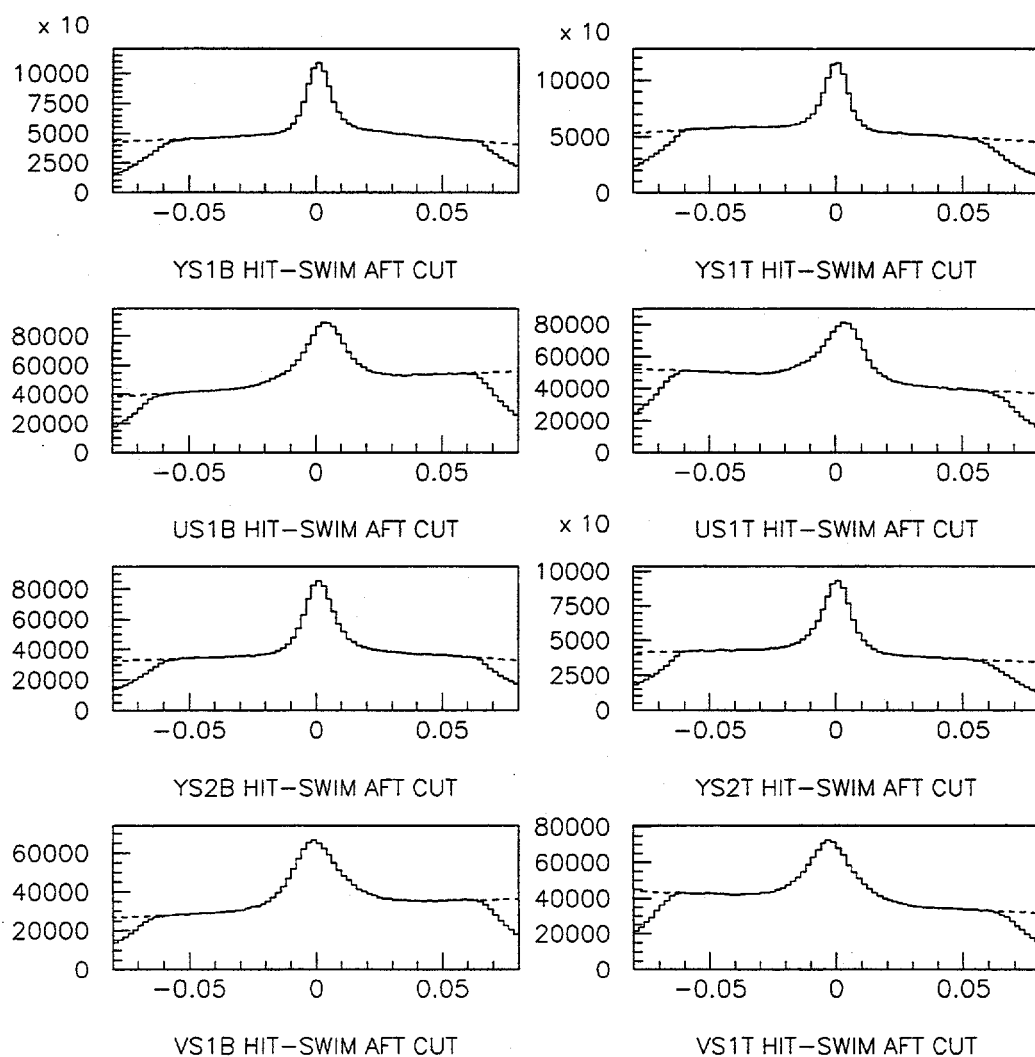
Figure 3.36: Distribution of the distances between the hits on a plane and the iterated Y position of the spectrometer track at that plane for a subset of the muon data set. (Units are in inches.)
