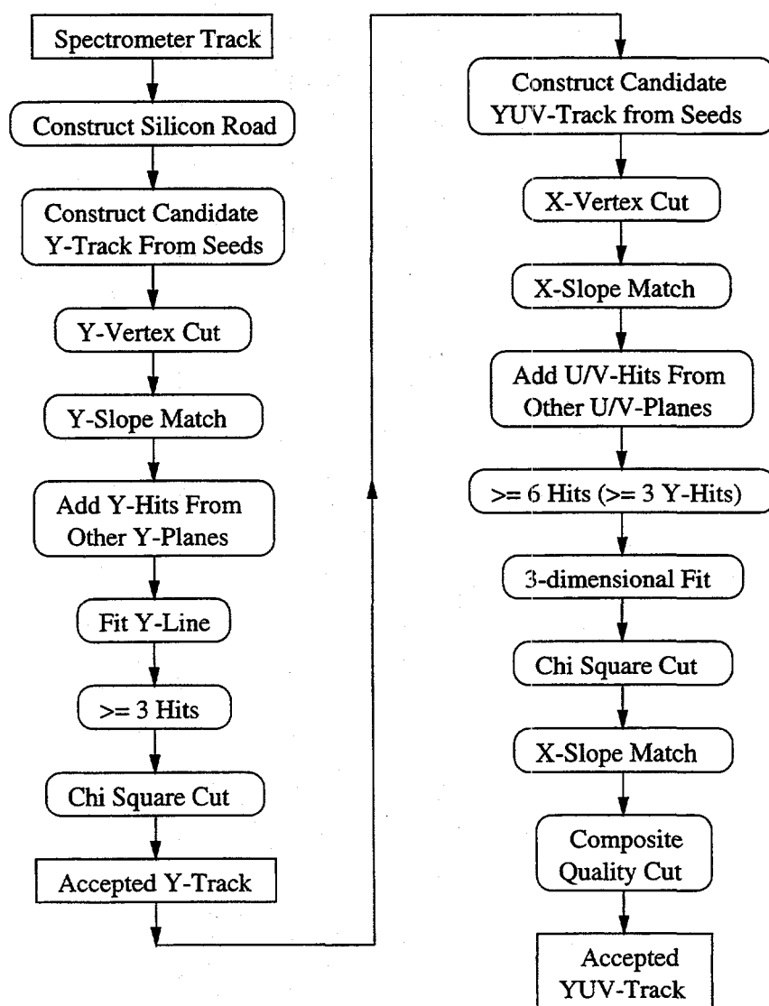
Figure 3.35: Flow chart of the silicon track reconstruction algorithm.
