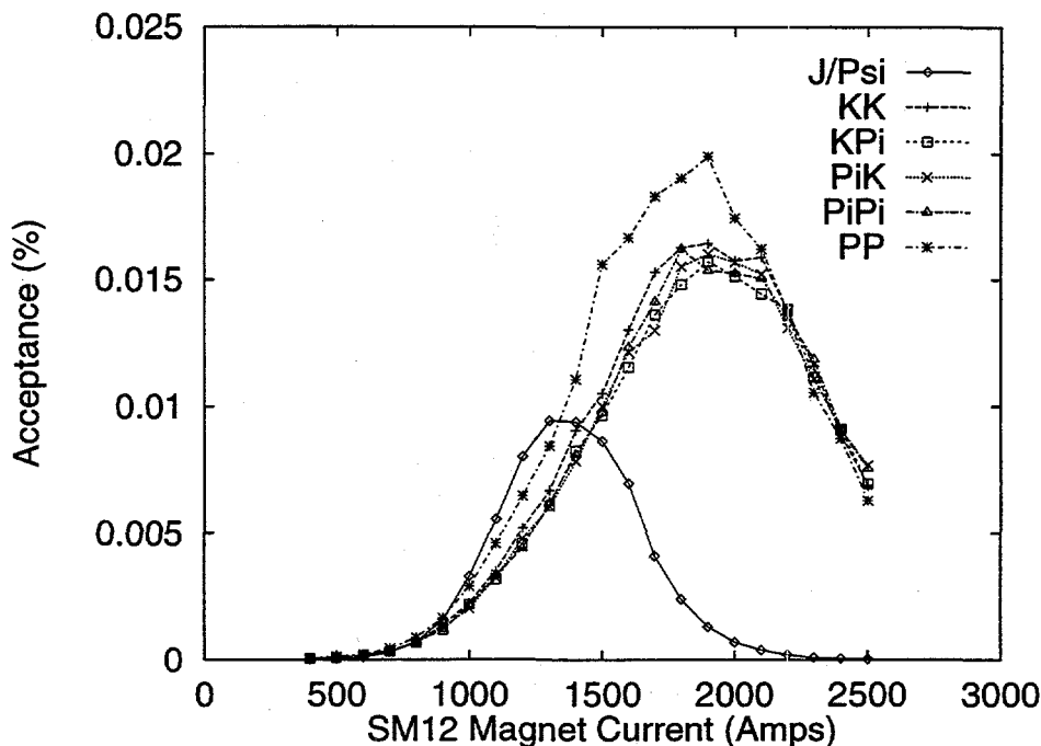
Figure 2.4: Acceptance of the spectrometer for various B_s decays as a function of SM12 current.
