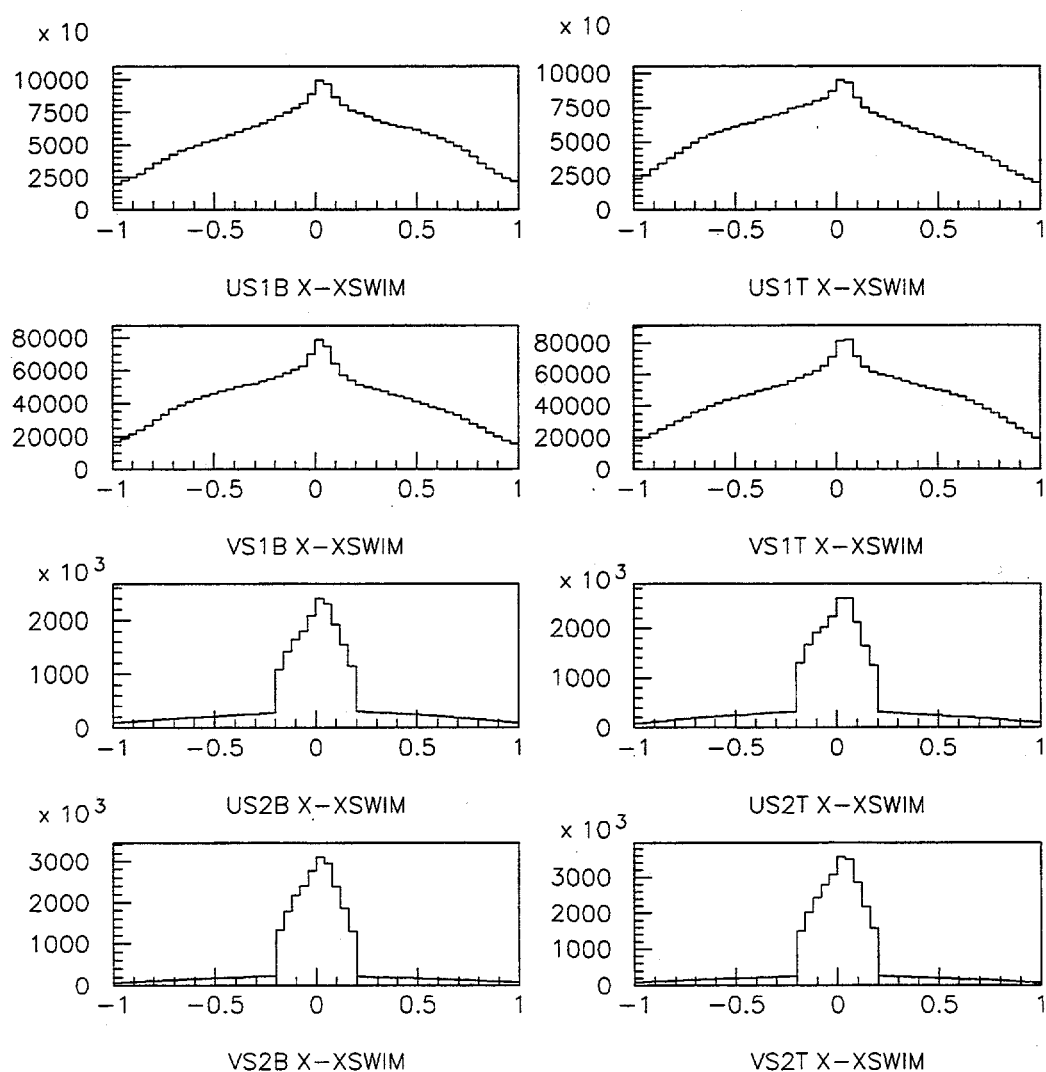
Figure 3.49: Distribution of the distances between the closest silicon hits on the various U/V planes and the iterated X position of the spectrometer track at the respective planes for a subset of the muon data set. (Units are in inches.)
