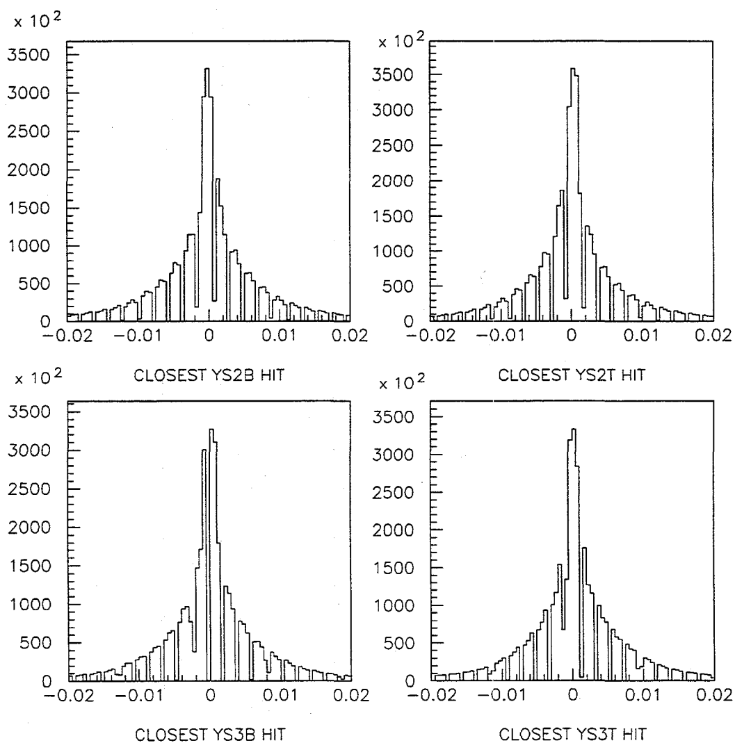
Figure 3.43: Distribution of the distances between the closest hits on the non-seed silicon Y planes and the candidate Y-track for a subset of the muon data set. (Units are in inches.)
