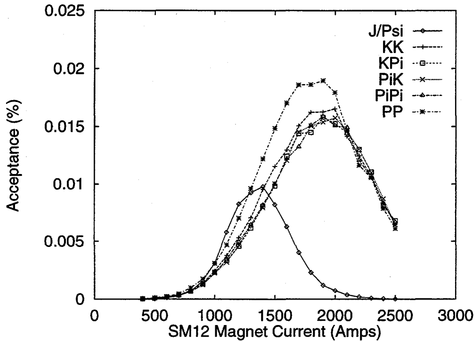
Figure 2.3: Acceptance of the spectrometer for various B_d decays as a function of SM12 current.
