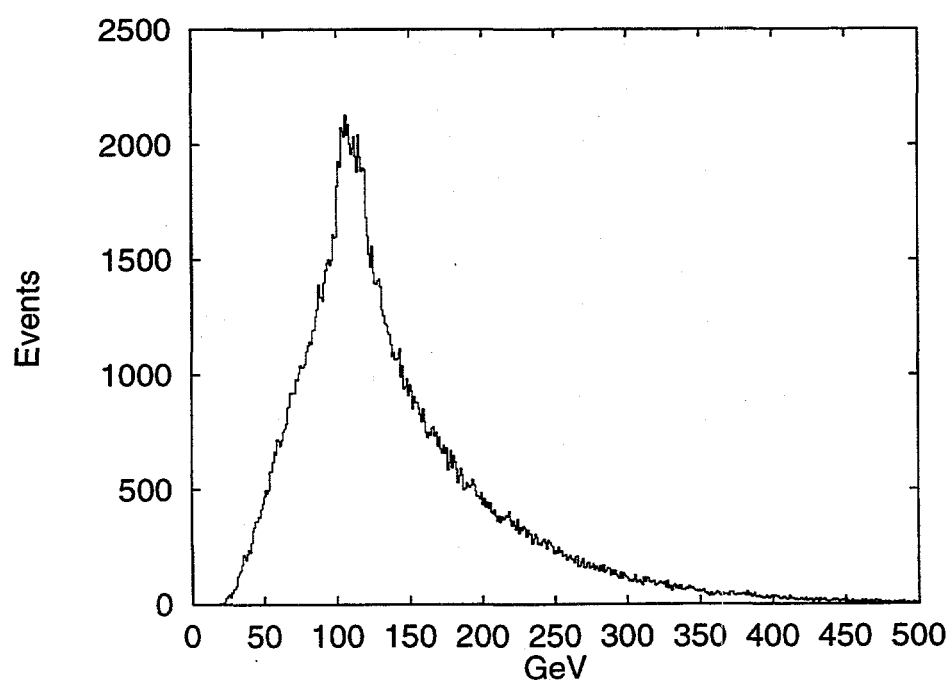
Figure 1.14: Laboratory frame energy spectrum of B_d mesons produced in the interaction of 800 GeV protons with a fixed target (Monte Carlo).
