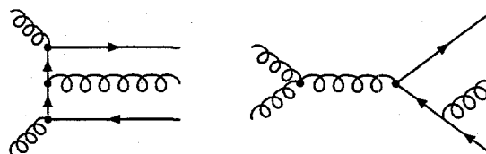
Figure 1.10: NLO diagrams with a real gluon.
