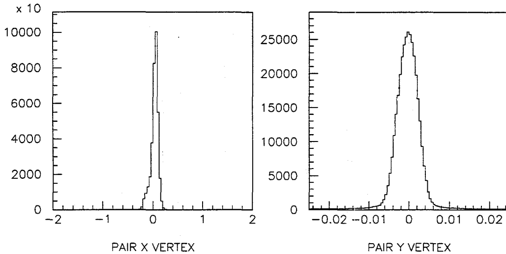
Figure 3.65: Distribution of the distance in X and Y to the target position of the decay vertex for a subset of the hadron data set. The plot on the left is the X distance and the right is the Y distance. (Units are in inches.)
