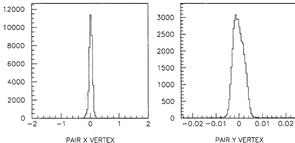
Figure 3.88: Distribution of the distance in X and Y to the primary interaction vertex position from the decay vertex for Monte Carlo generated prompt J/\psi decays to two muons. The plot on the left is the X distance and the right is the Y distance. (Units are in inches.)
