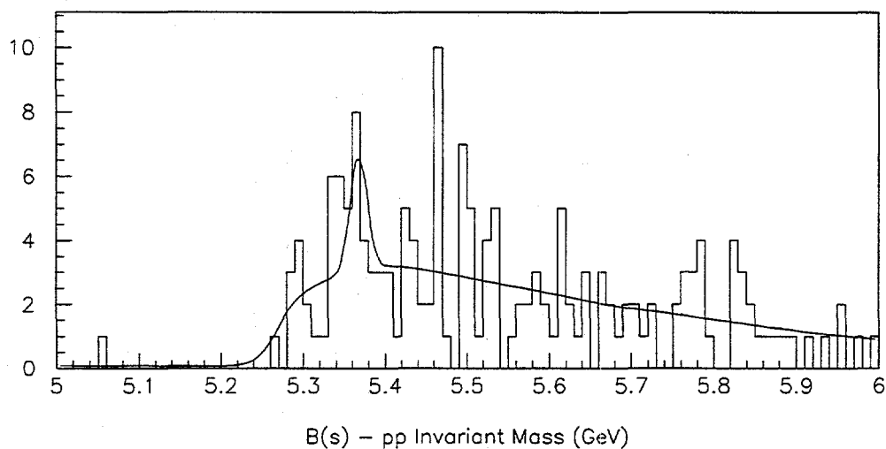
Figure 4.14: Results of the maximum likelihood fit to the invariant mass spectrum of the dihadron events assuming two protons for the B_s decay. (Units are in GeV.)
