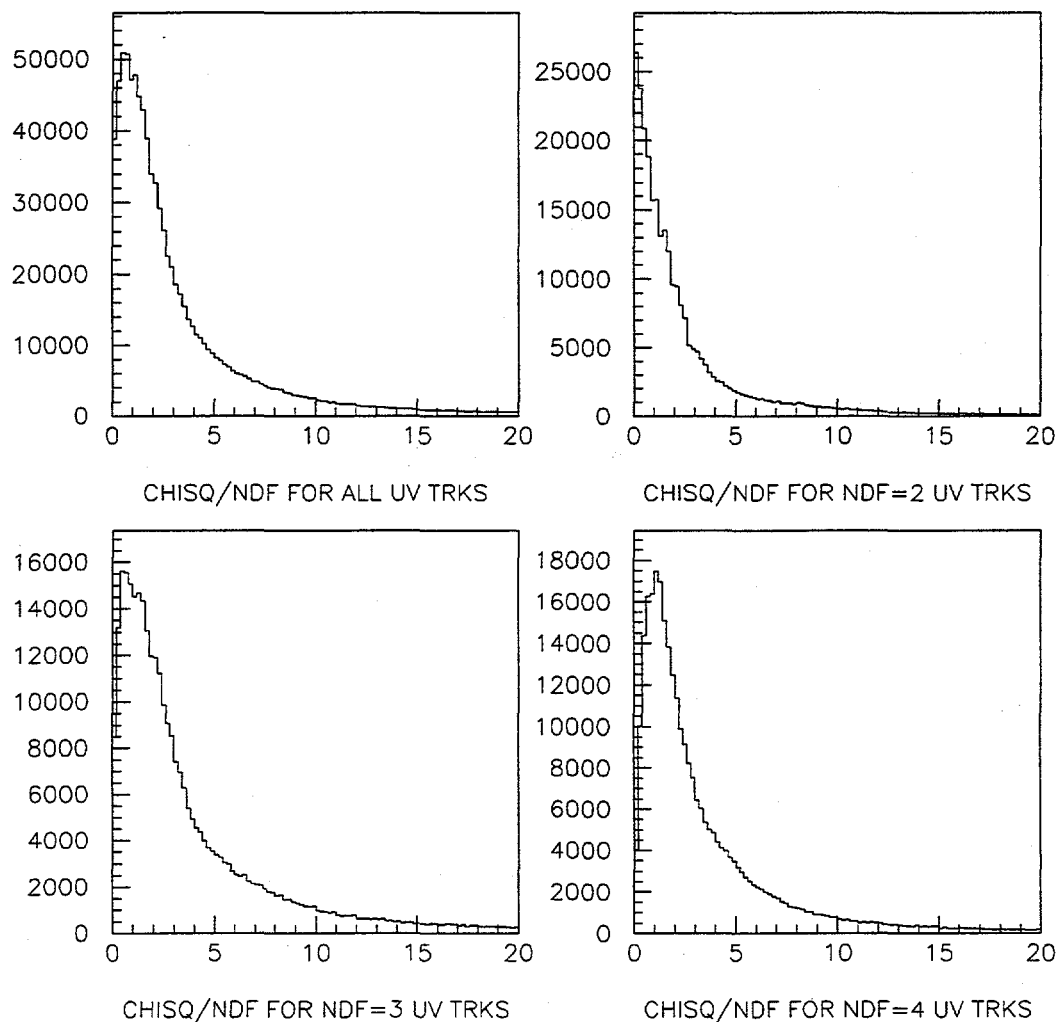
Figure 3.82: Distribution of the \chi^2 per degree of freedom distributions for tracks with 6 or more hits, 6 hits, 7 hits and 8 hits for Monte Carlo generated prompt J/\psi decaying to two muons.
