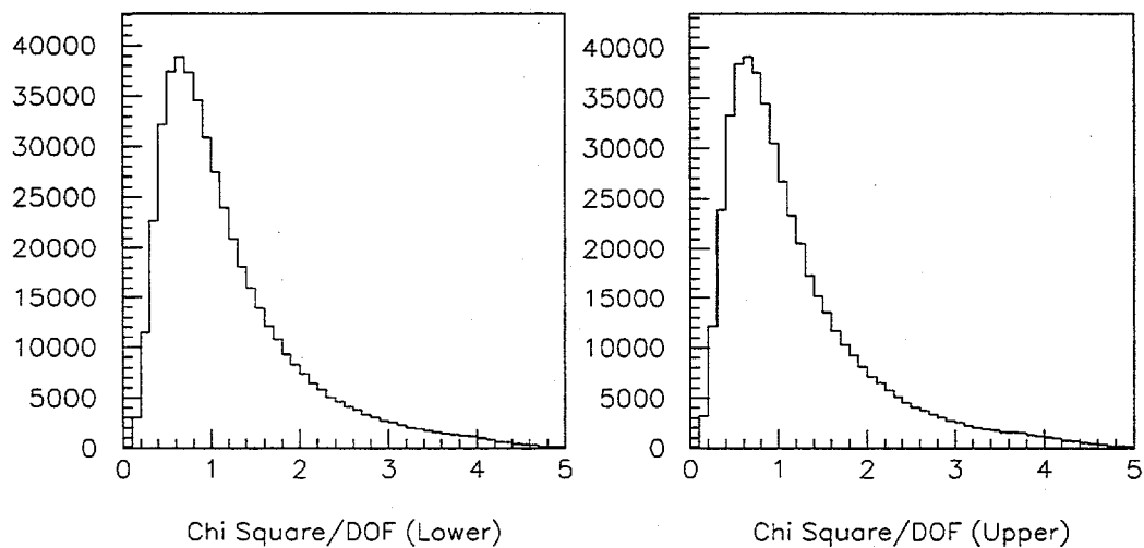
Figure 3.9: Distribution of the \chi^2 per degree of freedom for accepted muon tracks. The distribution for tracks in the lower (upper) arm of the spectrometer are on the left (right).
