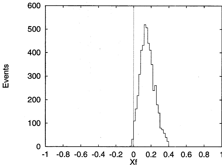
Figure 3.95: X_F spectrum of accepted B mesons for B \rightarrow \pi^+\pi^- assuming 100% detector efficiency (Monte Carlo).
