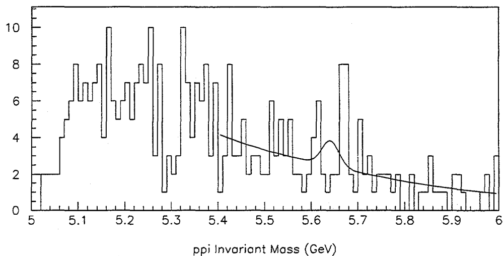
Figure 4.16: Results of the maximum likelihood fit to the invariant mass spectrum of the dihadron events assuming one pion and one proton. (Units are in GeV.)
