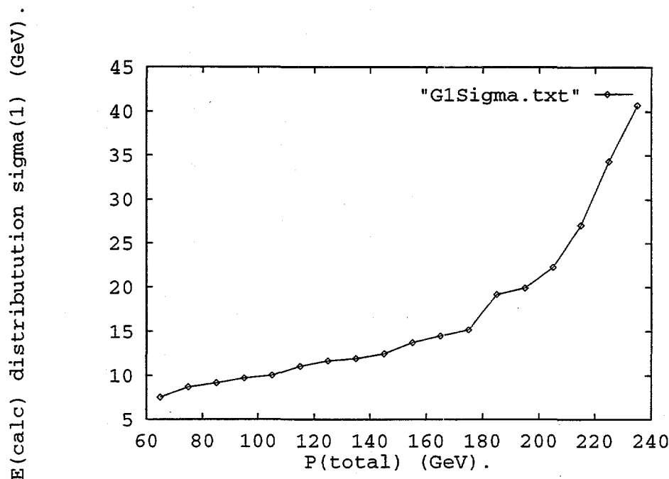
Figure 3.107: Variance ( \sigma_1 ) of the first Gaussian in the distribution of E_{calc} as a function of P_{total} for events triggered by E_L .
