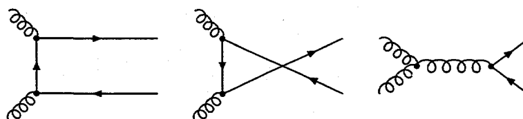
Figure 1.9: Gluon - gluon fusion diagrams.
