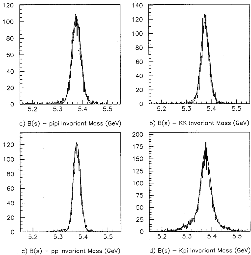
Figure 4.5: Results of the fit to the Monte Carlo generated B_s dihadron invariant mass spectra. (Units are in GeV.)
