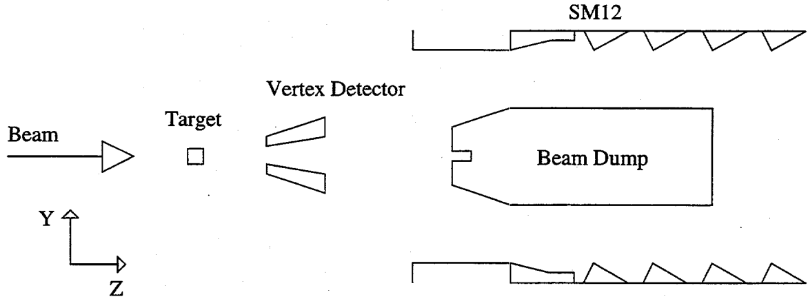
Figure 2.2: Schematic of the region around the target, SM12 and beam dump.
