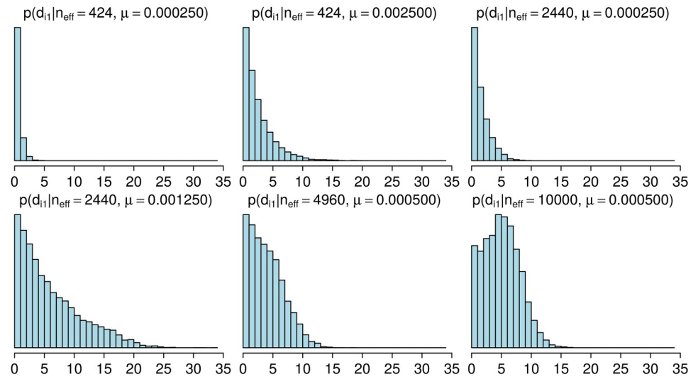
Fig 4. Distributions of pairwise distances for populations simulated with different parameters. The histograms show the estimated probability mass functions \hat{p}_{\text{sim}}(d_{11} | n_{\text{eff}}, \mu) with selected parameter vectors (n_{\text{eff}}, \mu) . Increasing \mu and/or n_{\text{eff}} tends to increase the distances. Each histogram represent variability in a simulated population at a single time point 6,000 generations after the beginning of the simulation.
