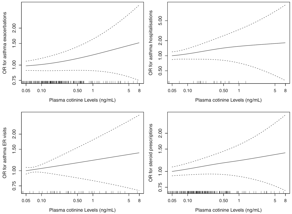
Figure 3: Dose-response of plasma cotinine and asthma exacerbations in the past 12 months, from generalized additive models using penalized splines. Results presented for total asthma exacerbations and separately for asthma-related hospitalizations, asthma-related ER visits and prescription of oral steroids for asthma.
