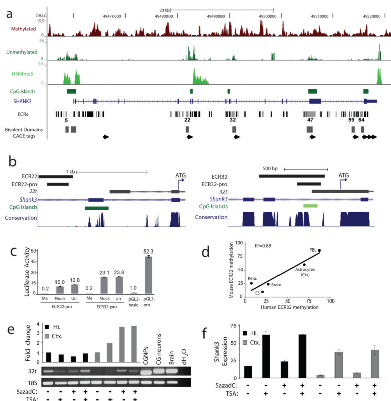
Figure 3. Novel transcripts initiate from differentially methylated, evolutionarily conserved intragenic promoters in a cell context-dependent manner
