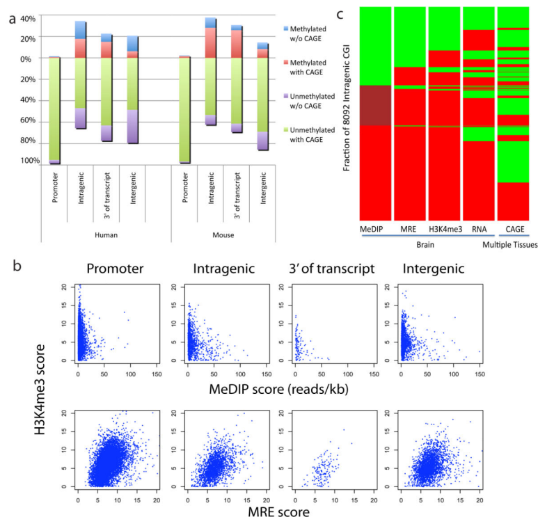
Figure 2. Differentially methylated intragenic CGIs exhibit features of promoters
