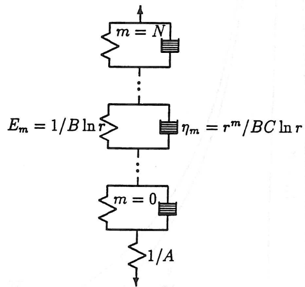
Figure 4: Discrete modified Kuhn model: representation as a generalized Kelvin model
