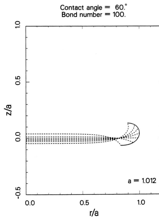
Figure 1. Meridian of container (solid curve) for contact angle 60^\circ and several Bond numbers showing meridians of some of the symmetric equilibrium solution surfaces (dashed curves), all having the same contact angle and energy, and enclosing the same volume of liquid.
