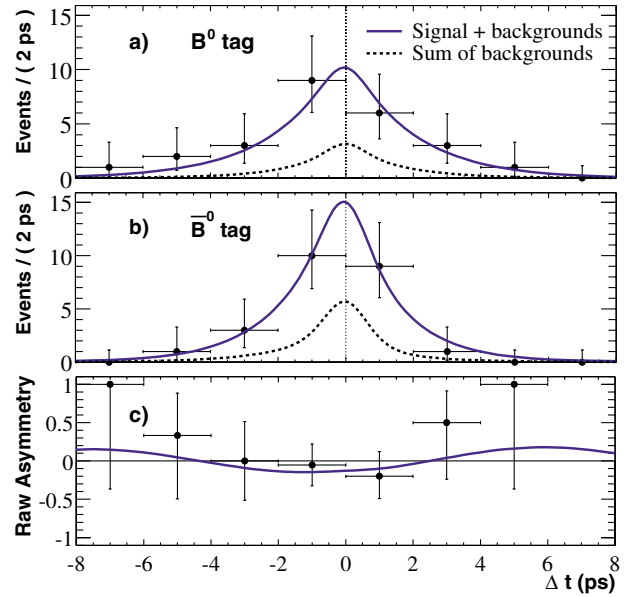
FIG. 2 (color online). Distributions of events (a) with a B^0 tag ( N_{B^0} ), (b) with a \bar{B}^0 tag ( N_{\bar{B}^0} ), and (c) the raw asymmetry (N_{B^0} - N_{\bar{B}^0}) / (N_{B^0} + N_{\bar{B}^0}) , as functions of \Delta t . Candidates in these plots are required to satisfy -0.11 < \Delta E < 0.11 GeV and m_{ES} > 5.27 GeV/ c^2 . Of the 49 signal and background events in this region, 25 have a B^0 tag and 24 have a \bar{B}^0 tag, with fit background contributions of approximately five and seven events, respectively. The curves are projections that use the values of the other variables in the likelihood to determine the contributions to the signal and backgrounds.
