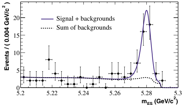
FIG. 1 (color online). Projection in m_{ES} for the results of the CP fit, displayed with the added requirement -0.11 < \Delta E < 0.11 GeV. In contrast, the CP fit uses the full \Delta E region. In the further restricted region m_{ES} > 5.27 GeV/ c^2 , there are 49 data events (points), of which about 12 events are fit as background. The background under the signal peak is composed of less than one event from B\bar{B} generic background and is roughly evenly divided among the other three background categories. Here, B^0 \rightarrow J/\psi K_S^0(\pi^0\pi^0) and inclusive J/\psi decays contribute to the enhancement in the background distribution at large m_{ES} .
