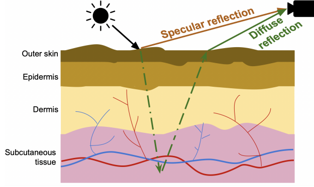
Figure 2.3: Illustration of the dichromatic skin model. Light incident on skin produces two reflective components. The specular component is due to the reflection from the skin surface, and the diffuse component is related to the absorption and scattering properties of the skin tissues. CHROM aims to eliminate contributions from the specular component in the RGB video since they do not contain pulsatile information.
