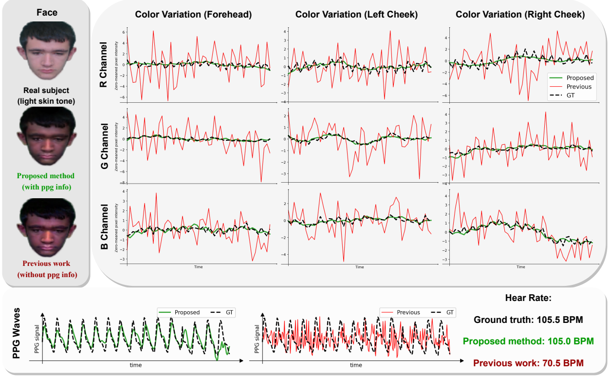
Figure 3.4: The proposed method successfully incorporates pulsatile signals into the generated videos, while the existing work [4] only focuses on the visual appearance. For different facial regions, frames generated by the proposed method exhibit similar pixel intensity variations as compared with frames from real videos, while the prior work shows unrealistic RGB variations. As a result, pulsatile signals can be well preserved in our method as opposed to the vanilla skin tone translation.
