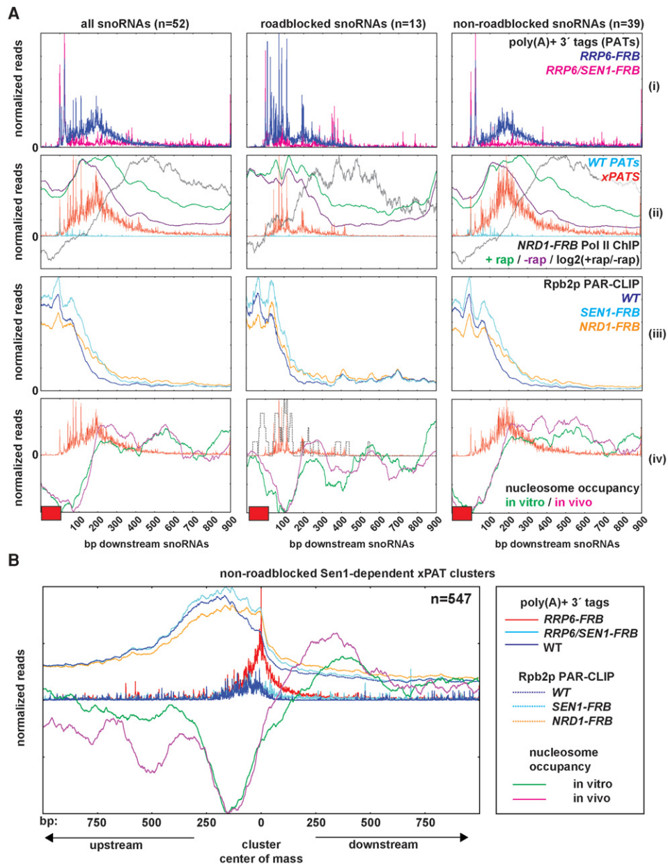
Figure 2. Two distinct classes of NNS-dependent snoRNA transcription termination. (A) Pile-up analysis of a 900-bp region downstream from snoRNA genes for all NNS-terminated snoRNAs ( left ), snoRNAs with RRP6/DIS3-FRB PAT (xPAT) cluster peaks associated with downstream DRS (roadblocked snoRNAs; middle ), and snoRNA xPAT cluster peaks without downstream DRS (nonroadblocked snoRNAs; right ). (i,ii,iv) PATs for the indicated strains. (ii) Pol II ChIP signal from NRD1-FRB strains in the absence (purple) or presence (green) of rapamycin, with the gray line indicating the log 2 ratio of rapamycin treated over untreated cells. (iii) Pol II occupancy as assayed by PAR-CLIP of Rpb2p for the indicated strains. (iv) The distribution of xPATs relative to nucleosome occupancy. (iv, middle) DRS signal (dashed gray line) included. The y-axes for all plots represent normalized reads. (B) Pile-up analysis on the centers of mass of clusters greater than or equal to twofold up-regulated in RRP6-FRB relative to RRP6/SEN1-FRB and lacking downstream DRS for the indicated data sets. Pol II PAR-CLIP and nucleosome occupancy are depicted as in A. The number of clusters included in pile-up analyses is indicated in the upper right ( n = 547).
