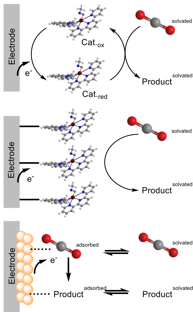
Figure 1. Illustration of catalytic CO 2 reduction by a homogeneous (top), an immobilized (middle), or a heterogeneous (bottom) catalyst. 8 Adapted with permission from ref 8. Copyright 2020 American Chemical Society.
