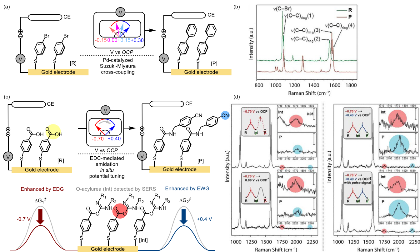
Figure 22. (a) Palladium-catalyzed Suzuki–Miyaura cross-coupling reaction, and (b) SERS of the reactant, 4-bromobenzenethiol (green line, R), and product, biphenyl-4-thiol (brown line, P). (c) Carbodiimide-mediated amidation reaction (CE, counter electrode; EDG, electron-donating group; EWG, electron-withdrawing group; OCP, open circuit potential; [R], reactant; [P], product; Int, intermediate; \Delta G_1^\ddagger , Gibbs free-energy barrier). (d) Left: Representative SERS of EDC-mediated amidation with -0.70 V (top graph) and a sequence of -0.70 V to OCP (bottom graph). Right: Representative SERS of EDC-mediated amidation after a sequence of -0.70 V to +0.40 V (top graph) and pulsed potential condition (bottom graph) (EDC = 1-ethyl-3-(3-(dimethylamino)propyl)carbodiimide). 132 Adapted with permission from ref 132. Copyright 2020 American Association for the Advancement of Science.
