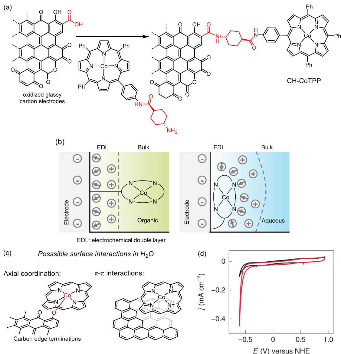
Figure 16. (a) Chemically anchored cobalt porphyrin with an aliphatic tether on the surface of a preoxidized glassy carbon electrode. (b) Interfacial environment of the electrode with chemically anchored cobalt porphyrin in an organic (left) and aqueous (right) electrolyte. (c) Possible noncovalent interactions between cobalt porphyrin and electrode in an aqueous electrolyte. (d) Representation of a cyclic voltammogram of hydrogen evolution using CH-CoTPP (red) in aqueous media (TPP = tetraphenylporphyrin). 114 Adapted with permission from ref 114. Copyright 2022 Nature Publishing Group.
