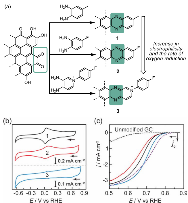
Figure 14. (a) Condensation of o -phenylenediamine derivatives with the o -quinone edge sites of graphene sheets to generate graphite-conjugated pyrazines. (b) Cyclic voltammograms of 1 (black), 2 (red), and 3 (blue) recorded in an N_2 saturated 0.1 M KOH electrolyte. (c) Linear sweep voltammograms of 1 (black), 2 (red), 3 (blue), and unmodified GC (dotted black) recorded in an O_2 saturated 0.1 M KOH electrolyte. 92 Adapted with permission from ref 92. Copyright 2015 American Chemical Society.
