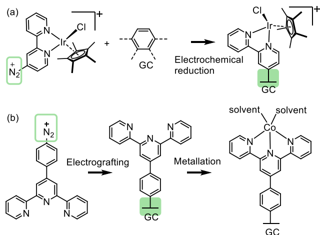
Figure 7. (a) Electrografting of iridium complex for water oxidation. 108 Adapted with permission from ref 108. Copyright 2012 American Chemical Society. (b) Electrografting of terpyridine followed by metallation to obtain surface-bound cobalt complex. 110 Adapted with permission from ref 110. Copyright 2015 The Royal Society of Chemistry.
