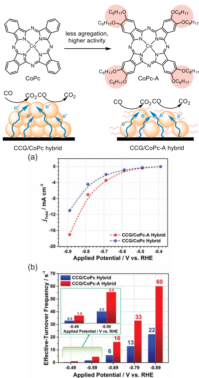
Figure 18. Ligand substitution of an immobilized cobalt complex reduces aggregation; CCG stands for chemically converted graphene. (a) Total current density for CCG/CoPc-A and CCG/CoPc hybrids in a CO 2 saturated electrolyte. (b) Effective TOFs for CO production by CCG/CoPc (blue bar) and CCG/CoPc-A (red bar) hybrids at different applied potentials. 137 Adapted with permission from ref 137. Copyright 2019 American Chemical Society.
