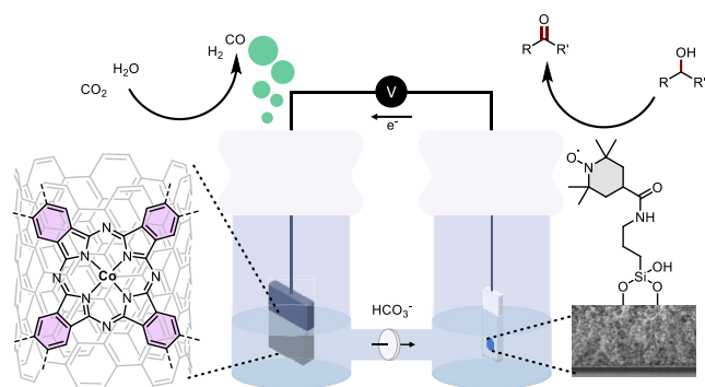
Figure 24. Integration of alcohol oxidation and CO 2 -to-syngas conversion in the same electrochemical setup. 39 Adapted with permission from ref 39. Copyright 2020 John Wiley & Sons, Inc.
