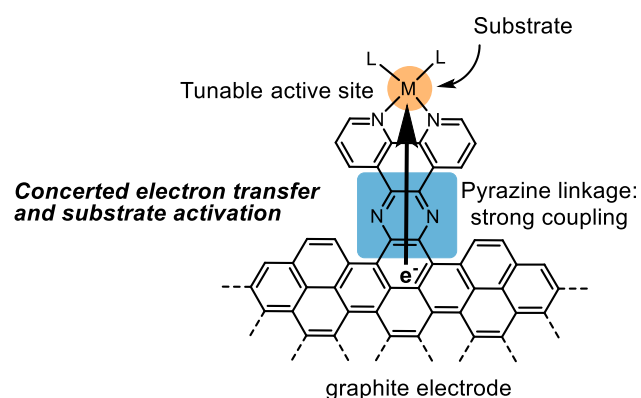
Figure 13. Graphite-conjugated catalyst coupled with the electrode through a pyrazine linkage. 94 Adapted with permission from ref 94. Copyright 2018 American Chemical Society.
