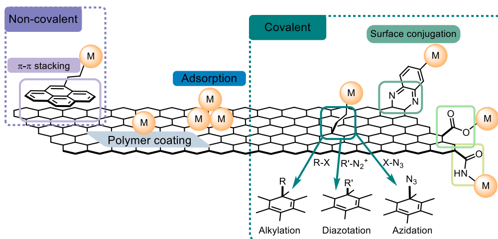
Figure 5. Common strategies for molecular surface functionalization of carbon-based electrodes. Pretreating the surface may be necessary to provide available sites for functionalization (e.g., oxidized glassy carbon electrode to increase carboxylic functionalities for the potential formation of ester or amide linkage). 11,72–76,97–99 Chemical structure of carbon electrode is simplified and does not reflect its complex chemical nature. Adapted with permission from ref 72. Copyright 2019 American Chemical Society.
