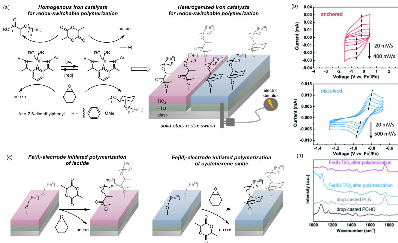
Figure 23. (a) Iron-based catalysts for redox-switchable polymerization of lactide and cyclohexene oxide, homogeneous and heterogenized on an electrode surface. (b) Cyclic voltammetry of an Fe(II)-TiO 2 -Ti mesh electrode (top) and a molecular bis(imino)pyridine iron bisphenoxide complex in solution (bottom) with varying scan rates. (c) Surface-initiated poly(lactide) from Fe(II)-modified TiO 2 electrode (left) and poly(cyclohexene oxide) obtained by oxidizing the surface Fe(II) complexes Fe(III) (right). (d) FTIR spectra of the functionalized surface after polymerization confirming the formation of surface-initiated polymers in comparison with drop-casted polymers on the surface. 40 Adapted with permission from ref 40. Copyright 2021 The Royal Society of Chemistry.
