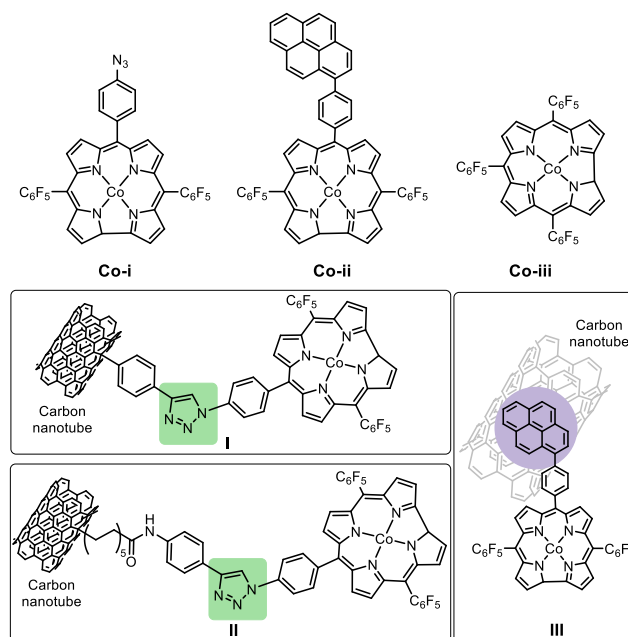
Figure 10. Homogenous cobalt complexes functionalized on carbon nanotubes affording modified electrodes through a short-conjugated linker (I), long alkene linker (II), and \pi – \pi interactions (III). 115 Hybrid electrode catalysts I and II are made from homogeneous cobalt complex Co-i. III is made from Co-ii. A cobalt complex without anchoring handles is exemplified by Co-iii. Adapted with permission from ref 115. Copyright 2018 John Wiley & Sons, Inc.
