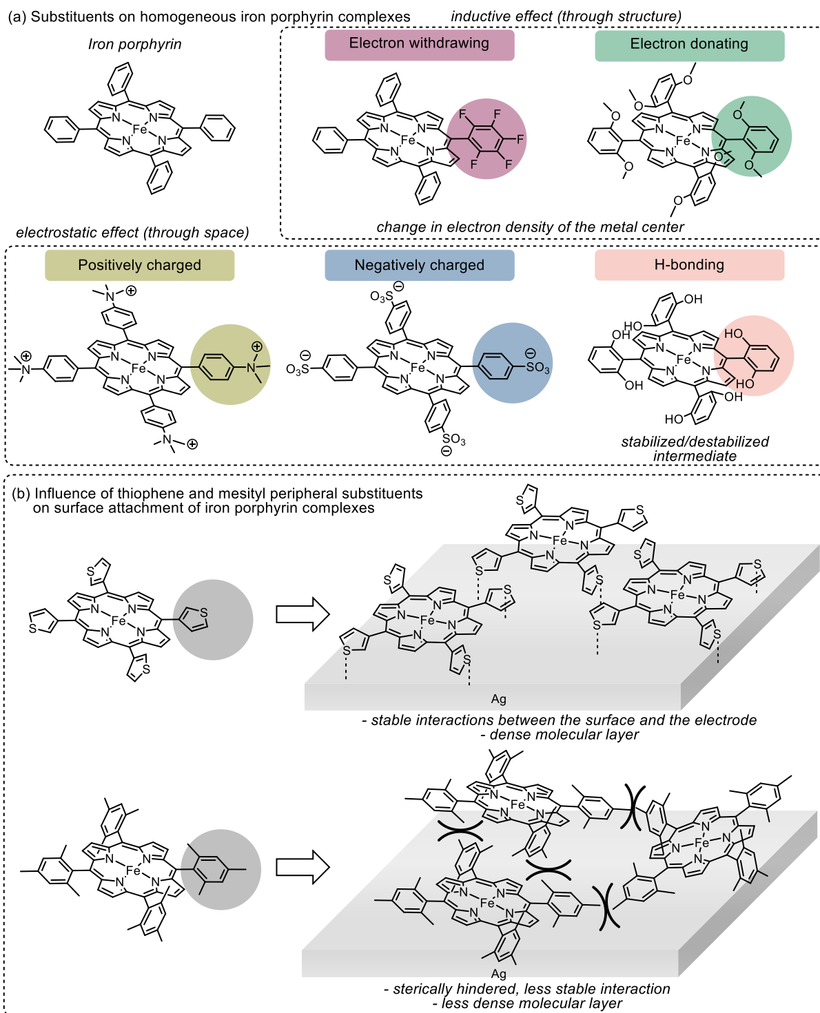
Figure 17. (a) Representations of iron porphyrin complexes with electron-withdrawing, electron-donating, positively, and negatively charged substituents on porphyrin, as well as substituents that possibly introduce H-bonding formation. (b) Homogenous iron complex with thiophenyl substituents resulted in a relatively dense molecular layer on an electrode surface, whereas bulky mesityl substituents resulted in a less stable interaction with the electrode surface and created less dense surface coverage. 133 Adapted with permission from ref 133. Copyright 2019 American Chemical Society.
