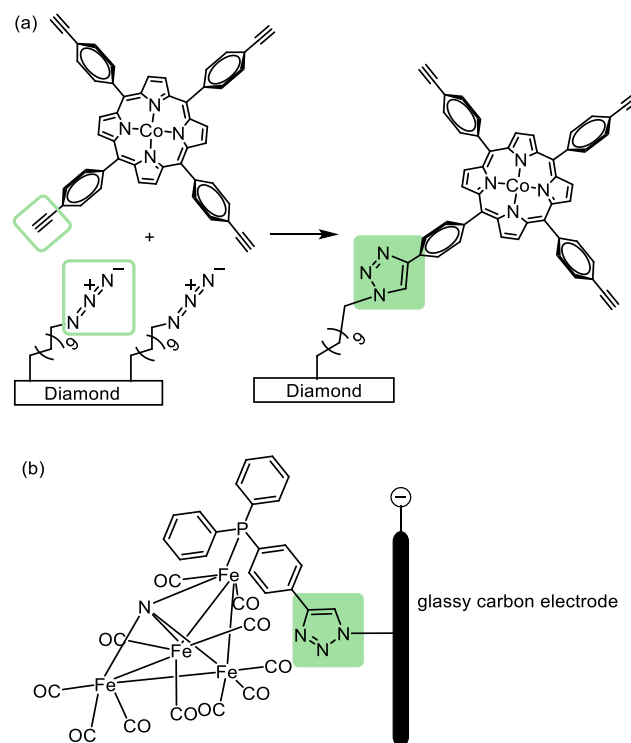
Figure 8. (a) Covalent immobilization using a click reaction with a cobalt complex. 17 Adapted with permission from ref 17. Copyright 2012 American Chemical Society. (b) Covalent immobilization of an iron complex via "click" reaction. 113 Adapted with permission from ref 113. Copyright 2019 American Chemical Society.
