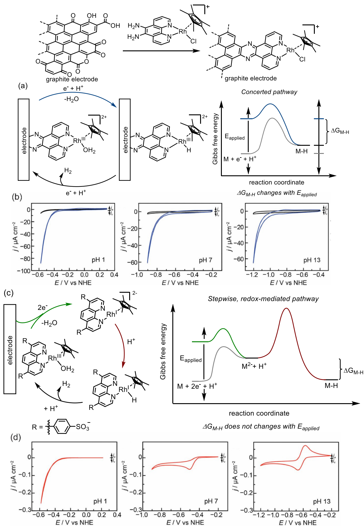
Figure 15. Graphite-conjugated rhodium system. (a) Graphite-conjugated rhodium undergoes concerted electron and proton transfer forming a metal–hydride ( M-H ) intermediate in hydrogen evolution. (b) pH dependence of hydrogen evolution using GCC-Rh (blue) and GCC-phenazine (black) at pH 1, 7, and 13. (c) Molecular rhodium catalyst undergoes stepwise electron transfer and substrate activation. E_{\text{applied}} is the applied potential,
