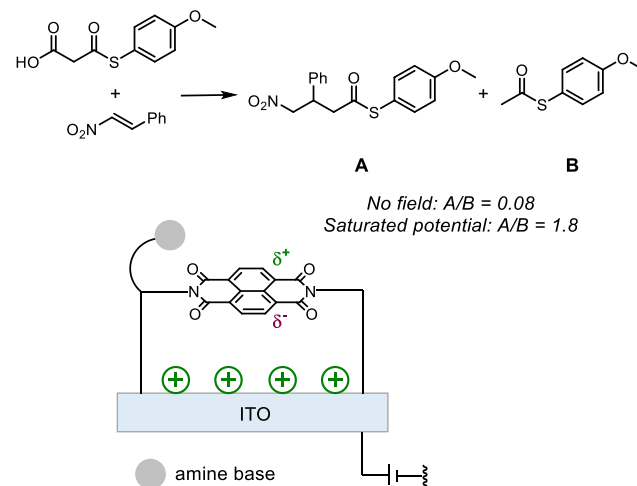
Figure 19. Anion- \pi catalysis assisted by an electric field. 162 Adapted with permission from ref 162. Copyright 2017 American Chemical Society.
