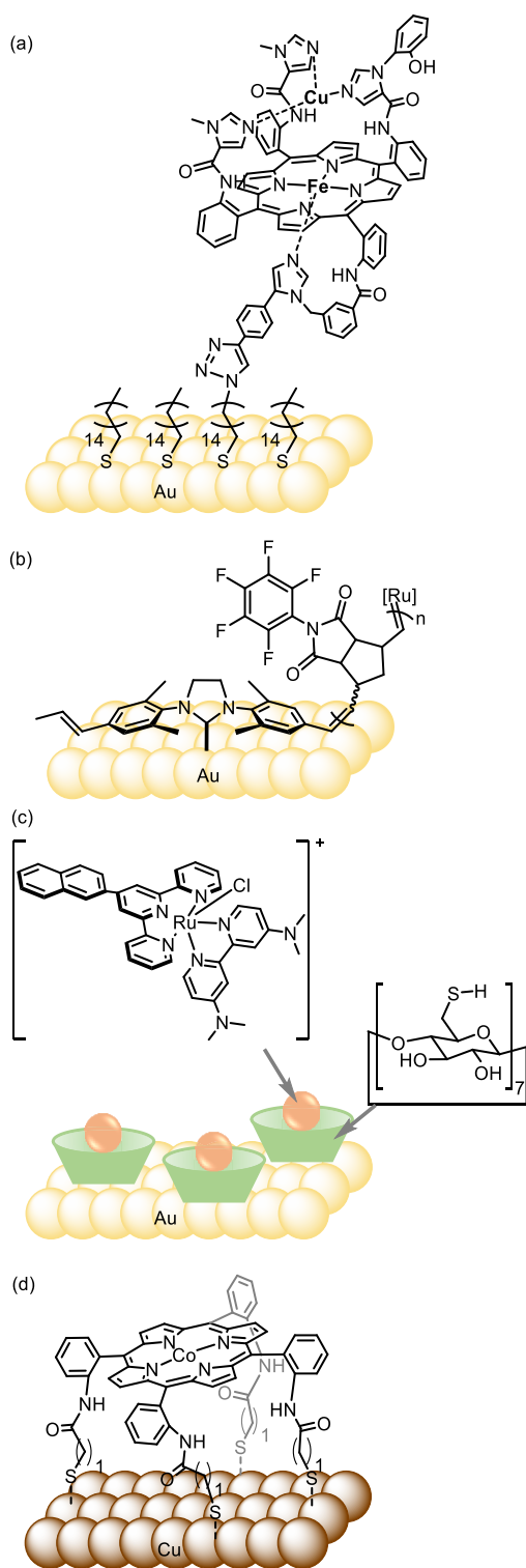
Figure 2. (a) Covalently attached functional model of cytochrome c oxidase to a gold electrode by using a terminal acetylene with a terminal azide bound to a self-assembled monolayer of thiolates. 26 Adapted with permission from ref 26. Copyright 2007 American Association for the Advancement of Science. (b) Gold surface functionalized with N-heterocyclic carbenes with polymer brushes containing ruthenium. 30 Adapted with permission from ref 30. Copyright 2013 American Chemical Society. (c) Ruthenium complex immobilized on a gold electrode surface through a surface-bound thiolated cyclodextrin host. 33 Adapted with permission from ref 33. Copyright 2021 Nature Publishing Group. (d) Copper electrode surface functionalized with a
