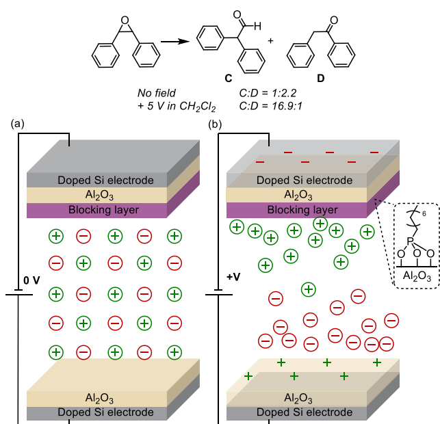
Figure 20. Selectivity in epoxide rearrangement achieved by an externally applied electric field in a parallel plate cell. 165 Illustration of the metal oxide–electrolyte interface at 0 V (a) and positive voltage (b) showing a significant voltage-dependent electric field at the interface. At 0 V, ions are assumed to distribute evenly at the interface, whereas, in the presence of an applied voltage, ions move toward the polarized plates generating an interfacial electric field as a result. Catalysis was confined to the bottom Al 2 O 3 layer by blocking the top layer with a monolayer of alkylphosphonic acid. Adapted with permission from ref 165. Copyright 2012 American Chemical Society.
