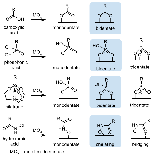
Figure 4. Possible binding modes of carboxylic acid, phosphonic acid, silatrane, and hydroxamic acid surface anchors to metal oxide surfaces (MO x ). The most favored binding modes are highlighted. 37 Bridging refers to binding of two metal ions on the metal oxide surface, and chelating refers to the binding of a chelating ligand to a single metal. Adapted with permission from ref 37. Copyright 2017 The Royal Society of Chemistry.
