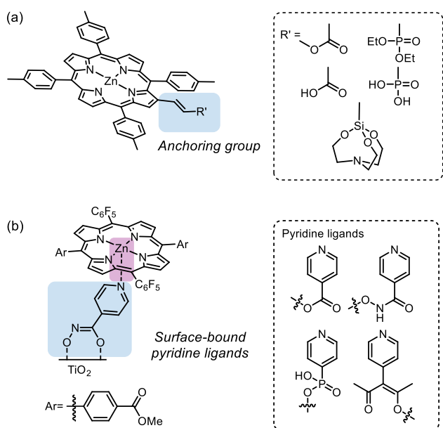
Figure 3. (a) Examples of metal complexes with molecular modifications on the ligand structure to enable surface anchoring. 57 Adapted with permission from ref 57. Copyright 2013 The Royal Society of Chemistry. (b) Metal complexes coordinated to surface-bound pyridine ligands as linkers. 62 Adapted with permission from ref 62. Copyright 2013 American Chemical Society.
