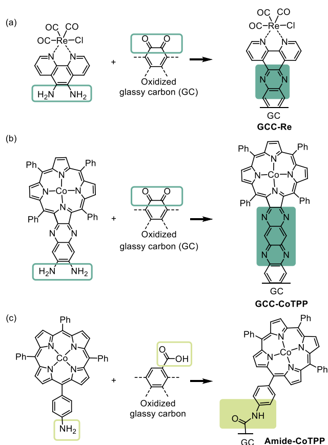
Figure 9. (a) Representation of graphite-conjugated rhenium active site for CO 2 reduction. 96 Adapted with permission from ref 96. Copyright 2016 American Chemical Society. (b and c) Immobilization of cobalt porphyrin on a modified electrode surface through a conjugated pyrazine and an amide linkage, respectively. 20 Adapted with permission from ref 20. Copyright 2019 American Chemical Society.
