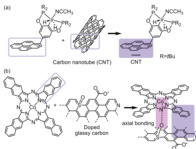
Figure 6. Noncovalent immobilization of metal complexes onto a carbon-based electrode. (a) Illustration of surface-bound Ir pincer catalyst. 102 Adapted with permission from ref 102. Copyright 2014 John Wiley & Sons, Inc. (b) Immobilized cobalt naphthalocyanine via \pi – \pi stacking and axial bonding. 105 Adapted with permission from ref 105. Copyright 2019 John Wiley & Sons, Inc.
