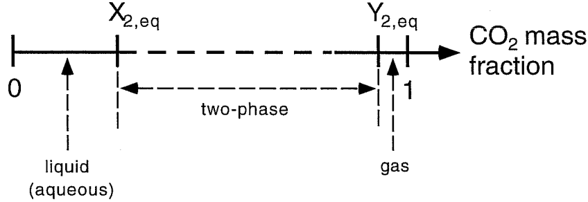
Figure 6. CO 2 phase partitioning in the system H 2 O - NaCl - CO 2 . The CO 2 mass fraction in brine-CO 2 mixtures can vary in the range from 0 (no CO 2 ) to 1 (no brine). X_{2,eq} and Y_{2,eq} denote, respectively, the CO 2 mass fractions in aqueous and gas phases corresponding to equilibrium phase partitioning in two-phase conditions. Mass fractions less than X_{2,eq} correspond to conditions in which only an aqueous phase is present, while mass fractions larger than Y_{2,eq} correspond to single-phase gas conditions. Mass fractions intermediate between X_{2,eq} and Y_{2,eq} correspond to two-phase conditions with different proportions of aqueous and gas phases.
