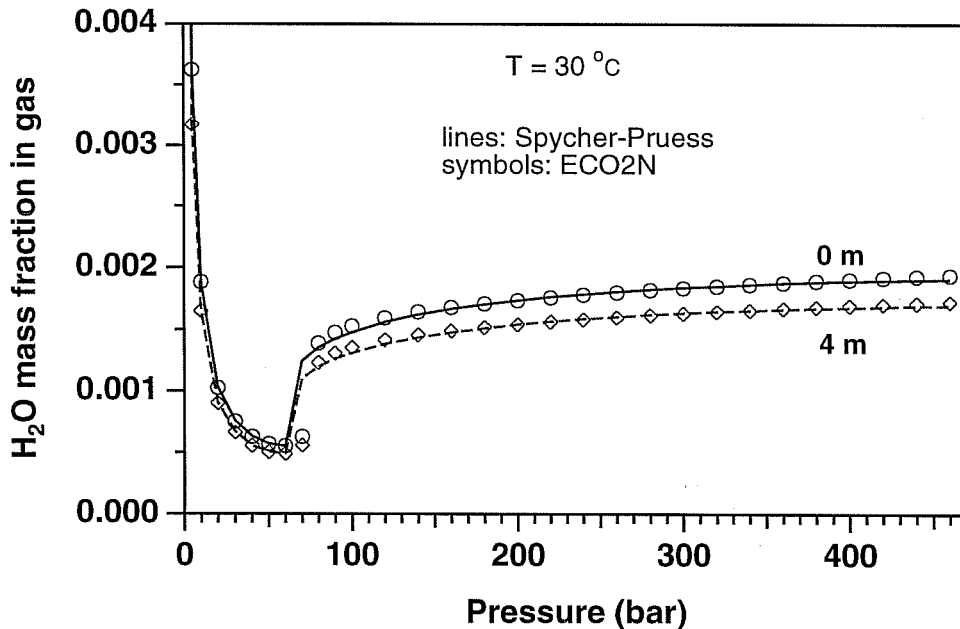
Figure 4. \text{H}_2\text{O} mass fractions in gas in two-phase system at T = 30^\circ\text{C} for pure water (0m) and 4-molal NaCl brine. Lines represent the original correlation of Spycher and Pruess (2005) that uses a Redlich-Kwong EOS for molar volume of \text{CO}_2 . Symbols represent data calculated by ECO2N in which the molar volume of \text{CO}_2 is obtained from the correlations of Altunin (1975).
