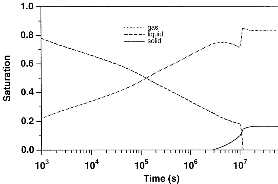
Figure 37. Phase saturations at the well block (A15 1).
