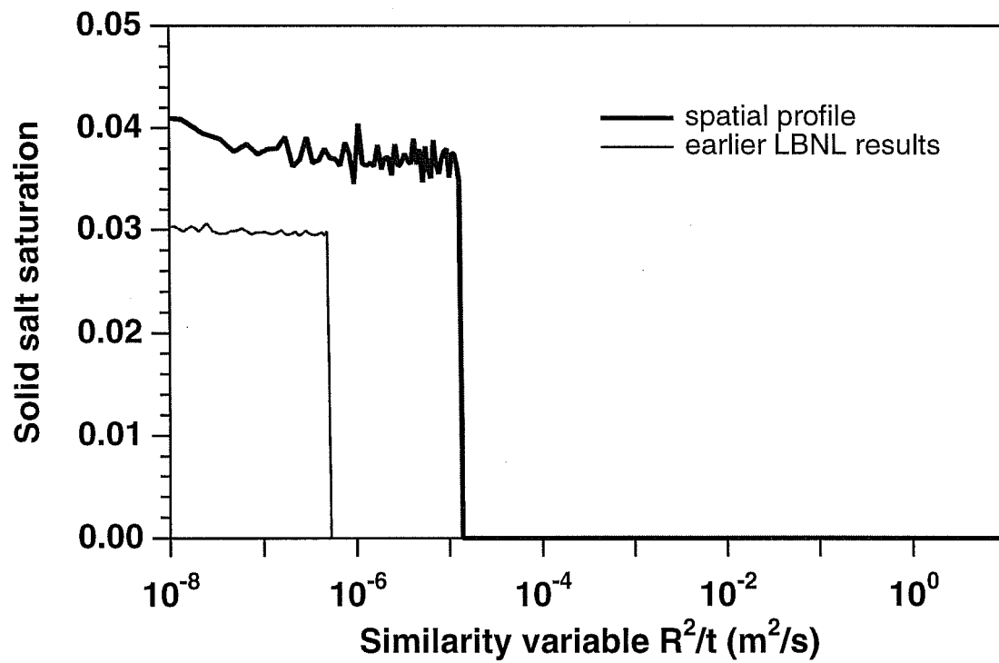
Figure 20. Simulated solid saturations.
