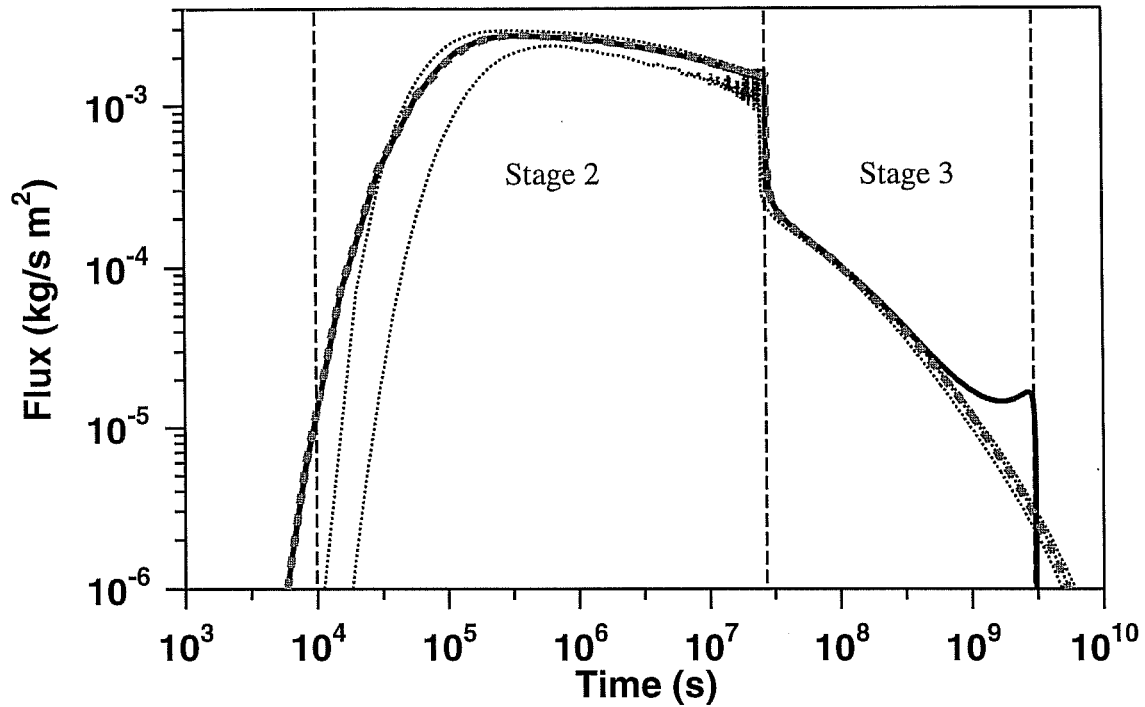
Figure 27. Simulated water flux at top of fault zone. Thick line is for variation (1), dashed line for variation (2), and thin lines represent results submitted in the code intercomparison project.
