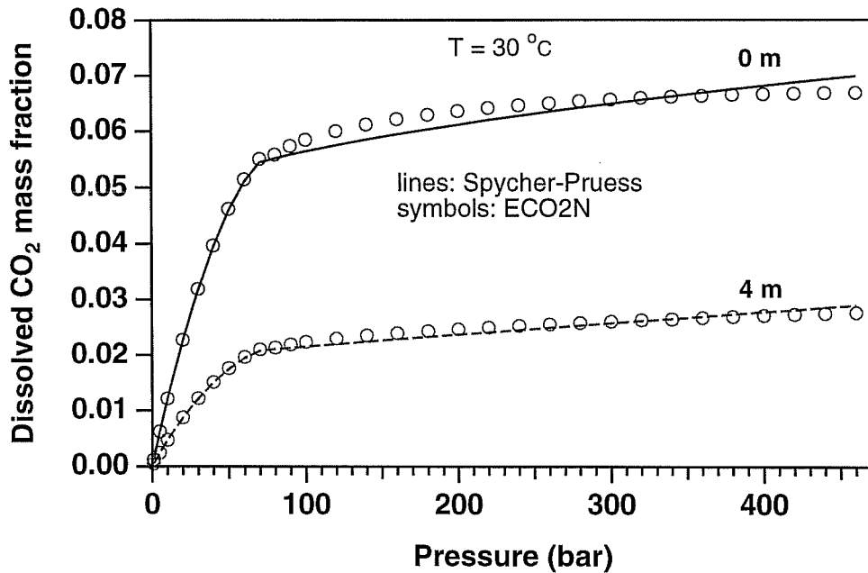
Figure 3. Dissolved \text{CO}_2 mass fractions in two-phase system at T = 30^\circ\text{C} for pure water (0m) and 4-molal NaCl brine. Lines represent the original correlation of Spycher and Pruess (2005) that uses a Redlich-Kwong EOS for molar volume of \text{CO}_2 . Symbols represent data calculated by ECO2N in which the molar volume of \text{CO}_2 is obtained from the correlations of Altunin (1975).
