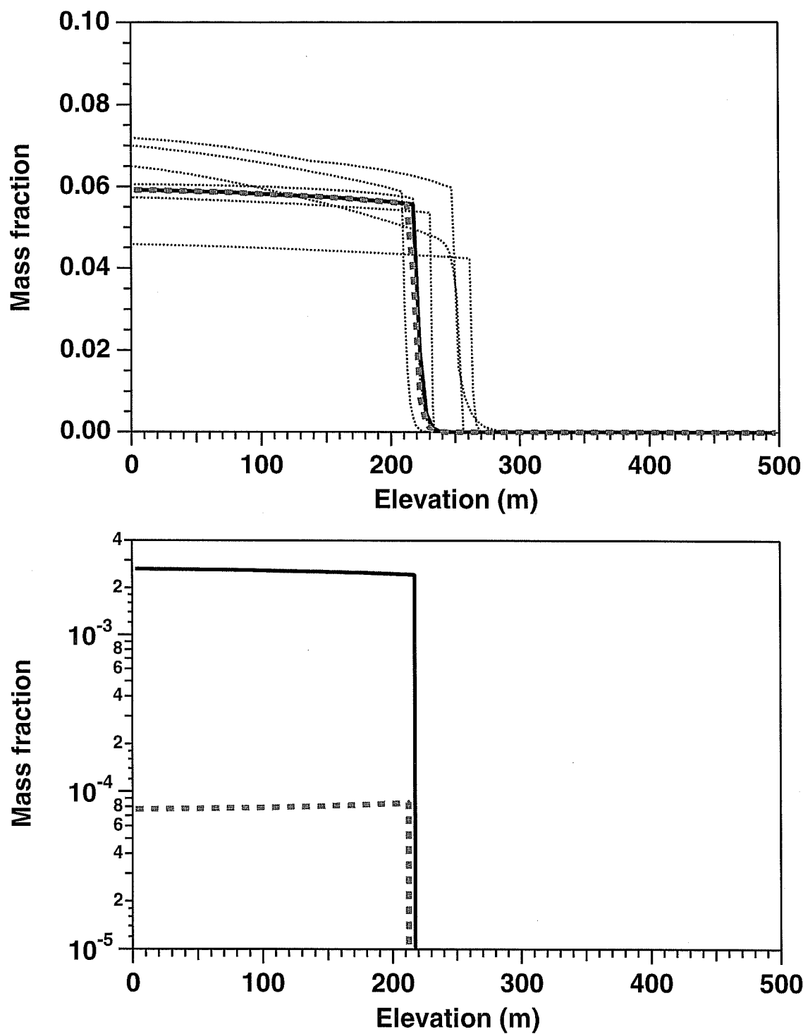
Figure 30. Dissolved CO 2 mass fraction in aqueous phase (top) and dissolved water mass fraction in gas (bottom) after 10 7 s. Thick lines are for variation (1), dashed lines for variation (2), and thin lines represent results submitted in the code intercomparison project.
