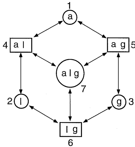
Figure 1. Possible phase combinations in the system water-CO 2 . The phase designations are a - aqueous, l - liquid CO 2 , g - gaseous CO 2 . Separate liquid and gas phases exist only at subcritical conditions.
