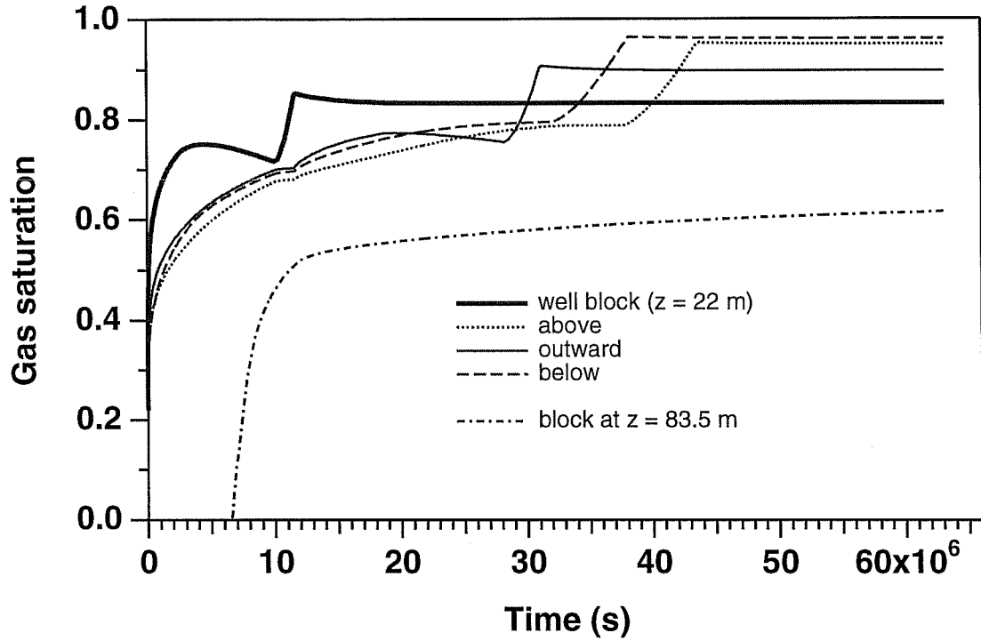
Figure 36. Gas saturations at the well block and its neighbors (above - A16 1; outward - A15 2; below - A14 1). Gas saturations at block A1G 1 at an elevation of 83.5 m (61.5 m above well block) are also shown.
